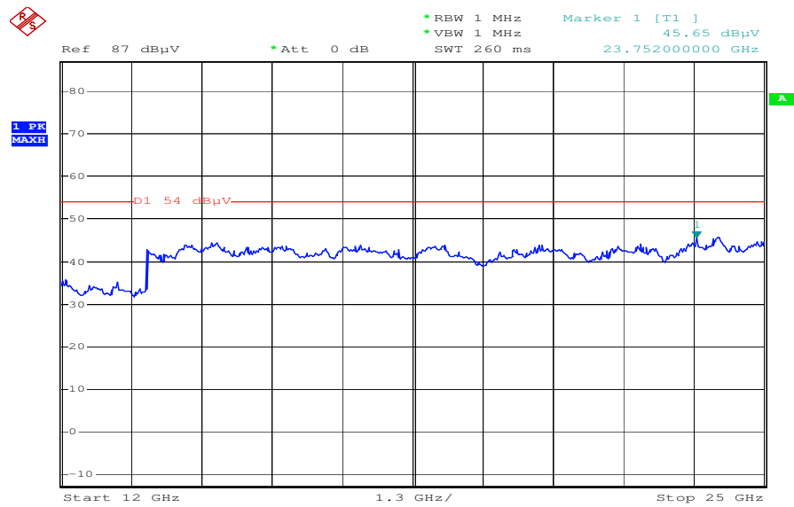
Plot 5: 12 - 25 GHz vertical/horizontal (receiver)
