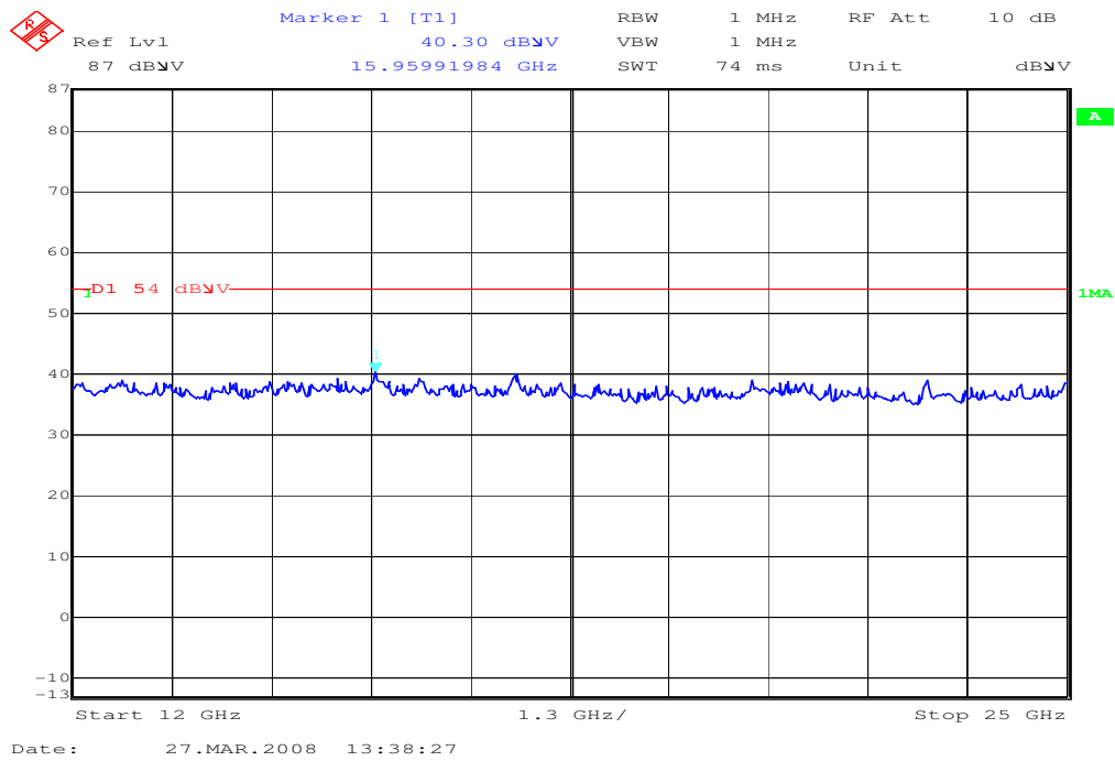
Plot 8: RX (12 GHz to 25 GHz)
