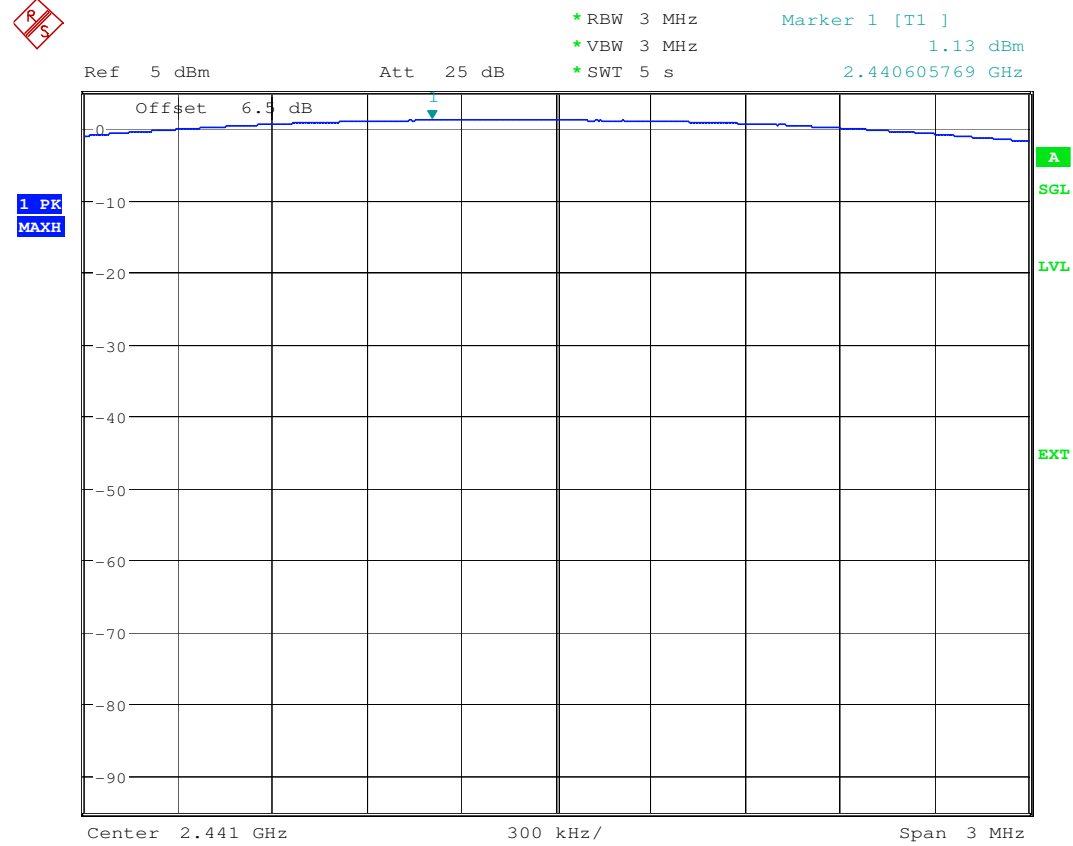
Plot 2 GFSK
