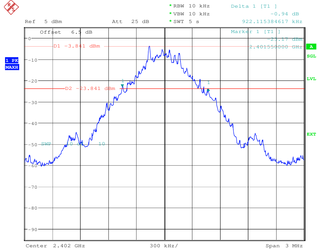
Plot 1 GFSK
