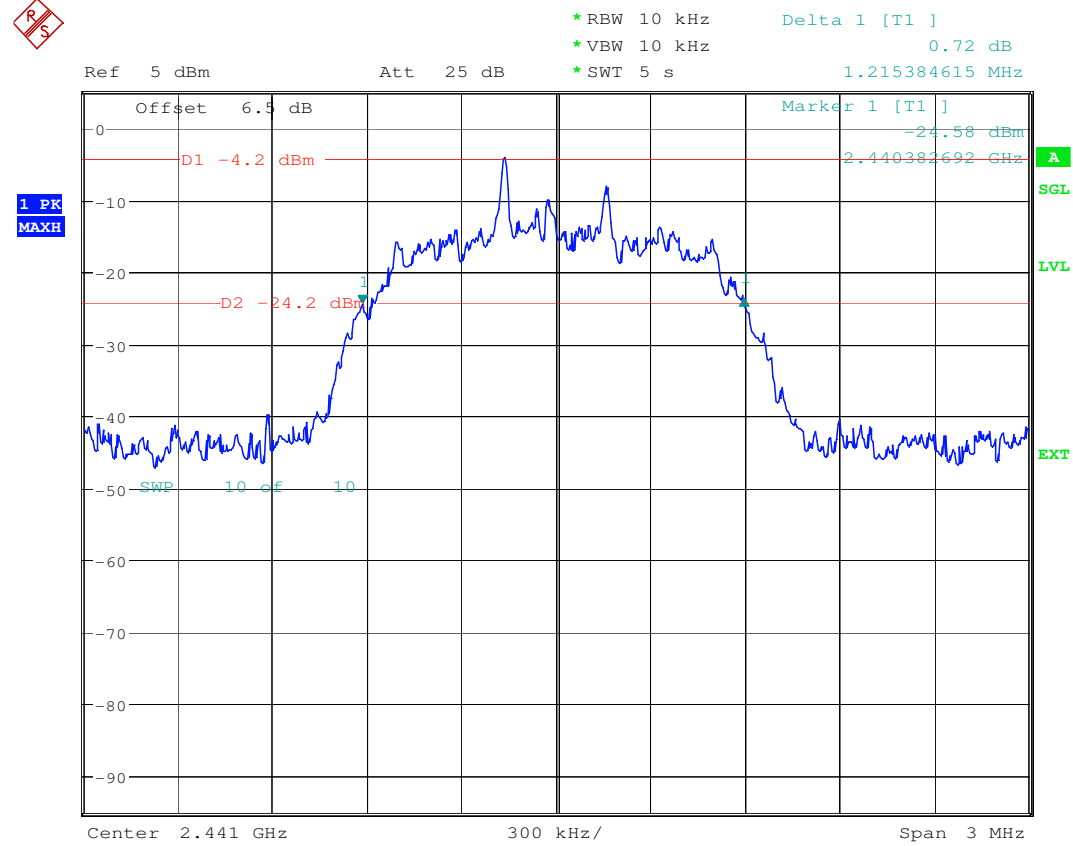
Plot 8 8DPSK
