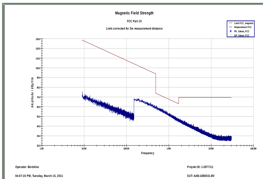
Plot 1: 9 kHz to 30 MHz / channel 00
