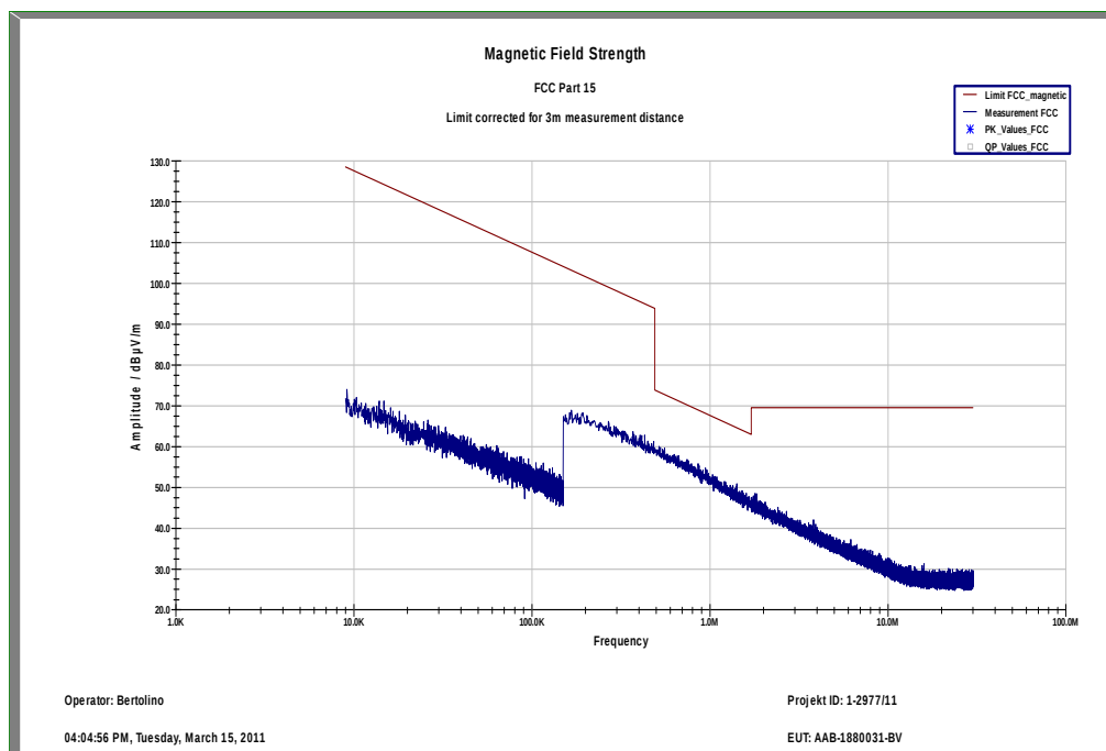
Plot 4: 9 kHz to 30 MHz; RX / Idle mode
