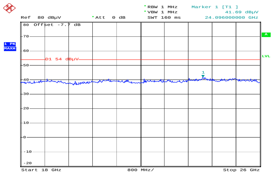
Plot 12: 18 GHz to 26 GHz / channel 78 (horizontal/vertical)
