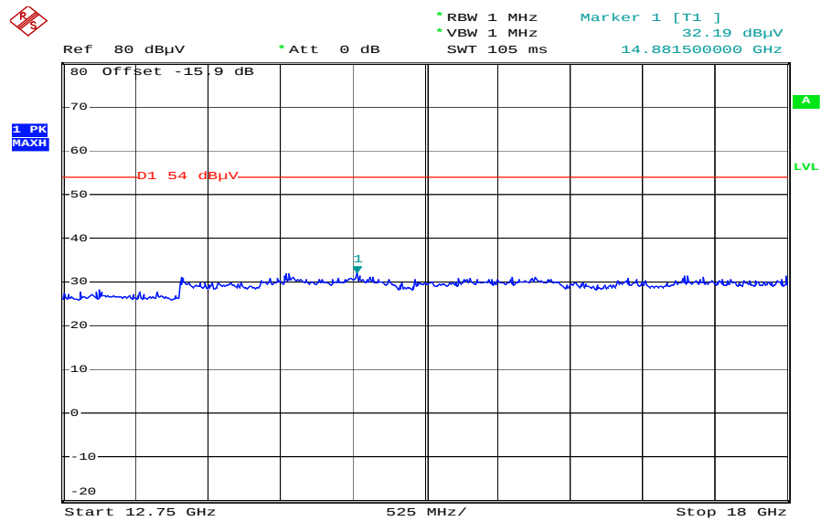
Plot 11: 12 GHz to 18 GHz / channel 78 (horizontal/vertical)
