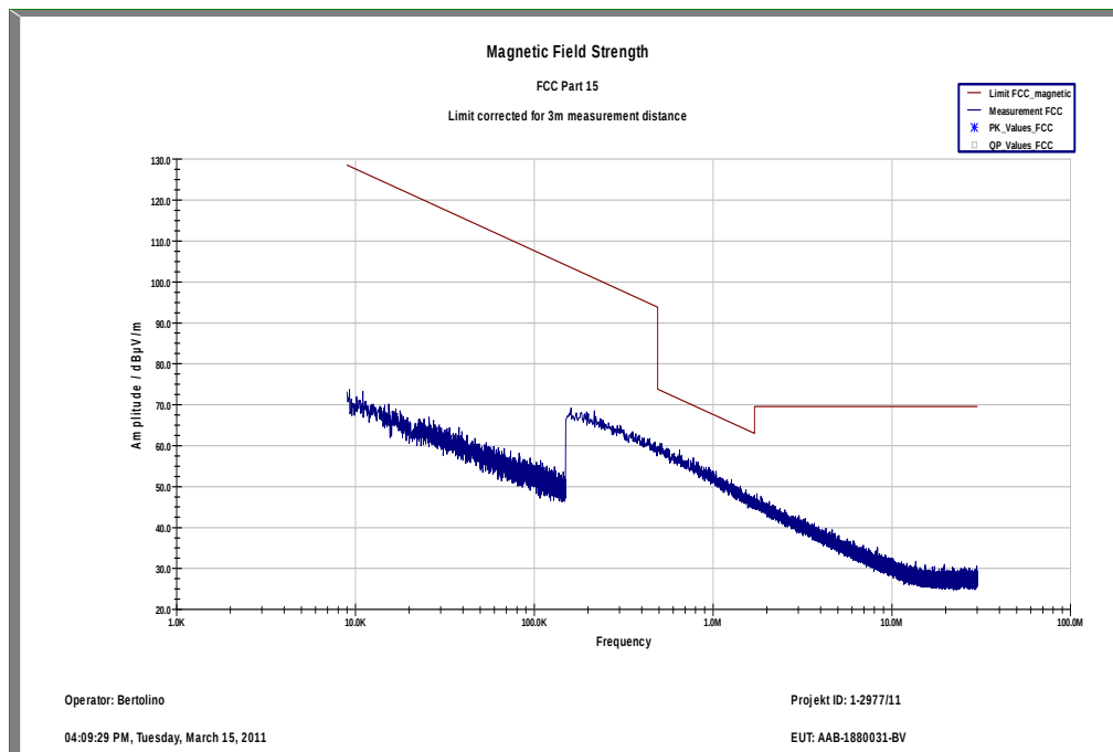
Plot 2: 9 kHz to 30 MHz / channel 39
