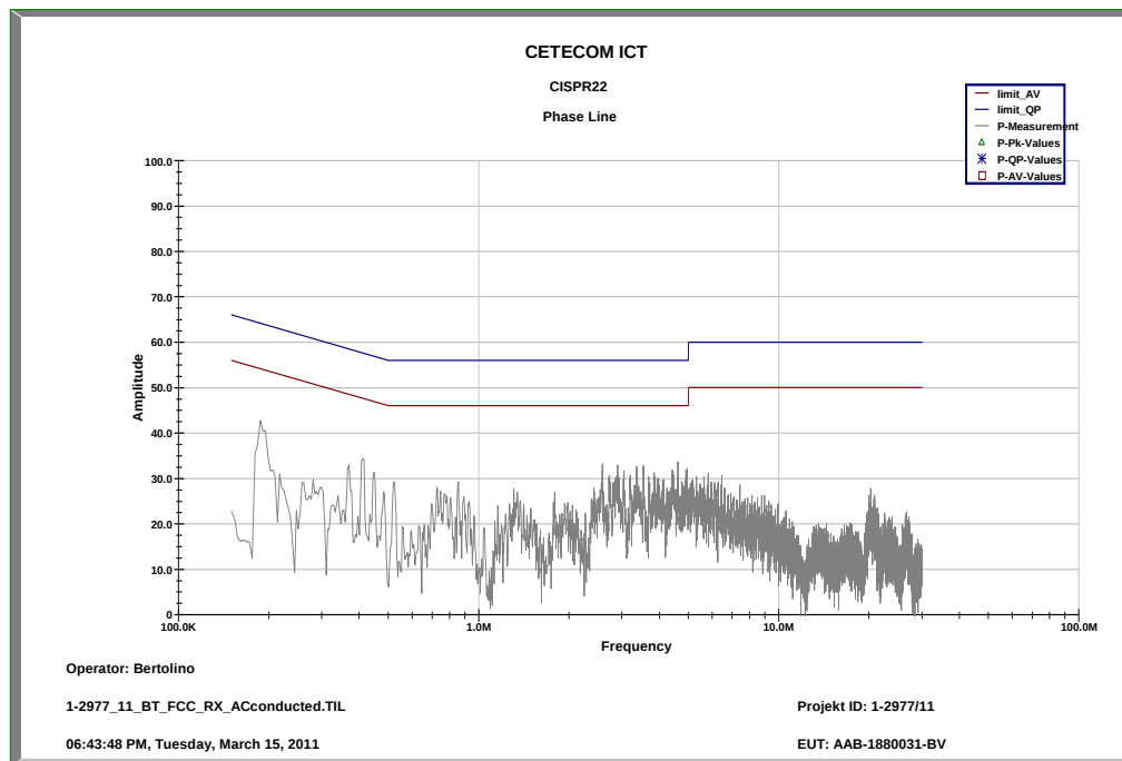
Plot 3: 9 kHz to 30 MHz / phase line
