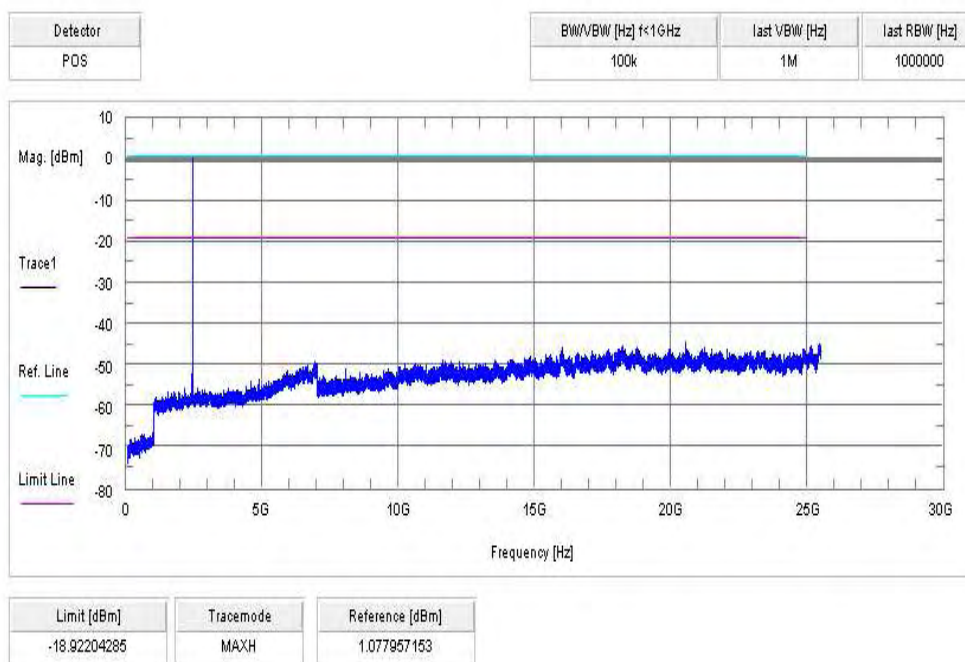
Plot 8: Channel 00 / 8DPSK
