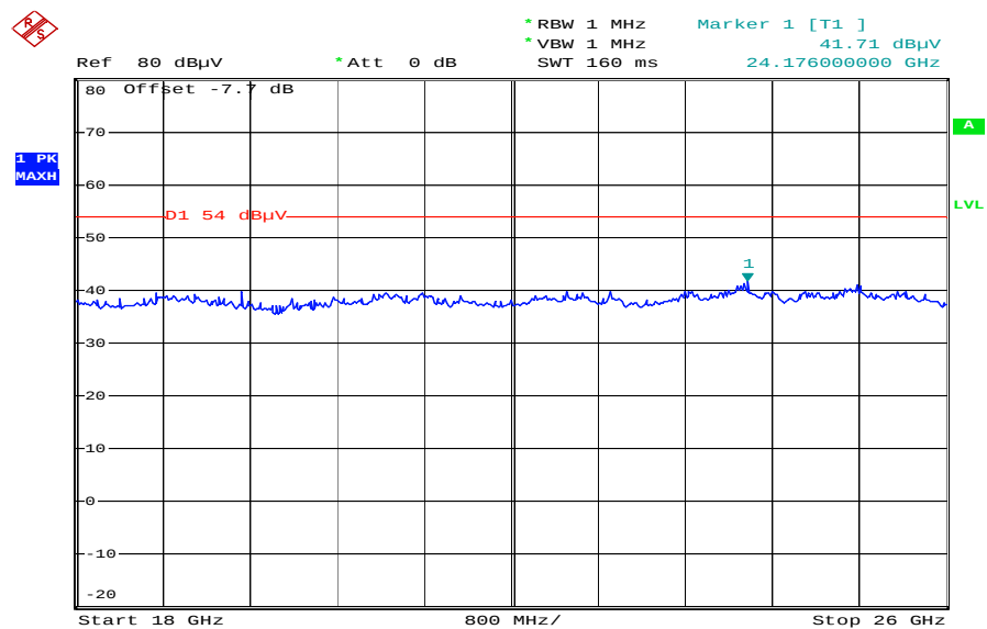
Plot 8: 18 GHz to 26 GHz / channel 39 (horizontal/vertical)
