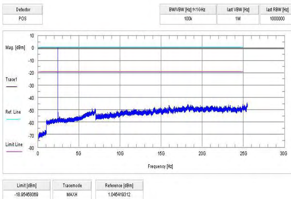
Plot 7: Channel 00 / 8DPSK
