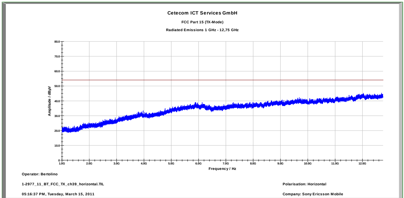
Plot 6: 1 GHz to 12.75 GHz / channel 39 (horizontal/vertical)
