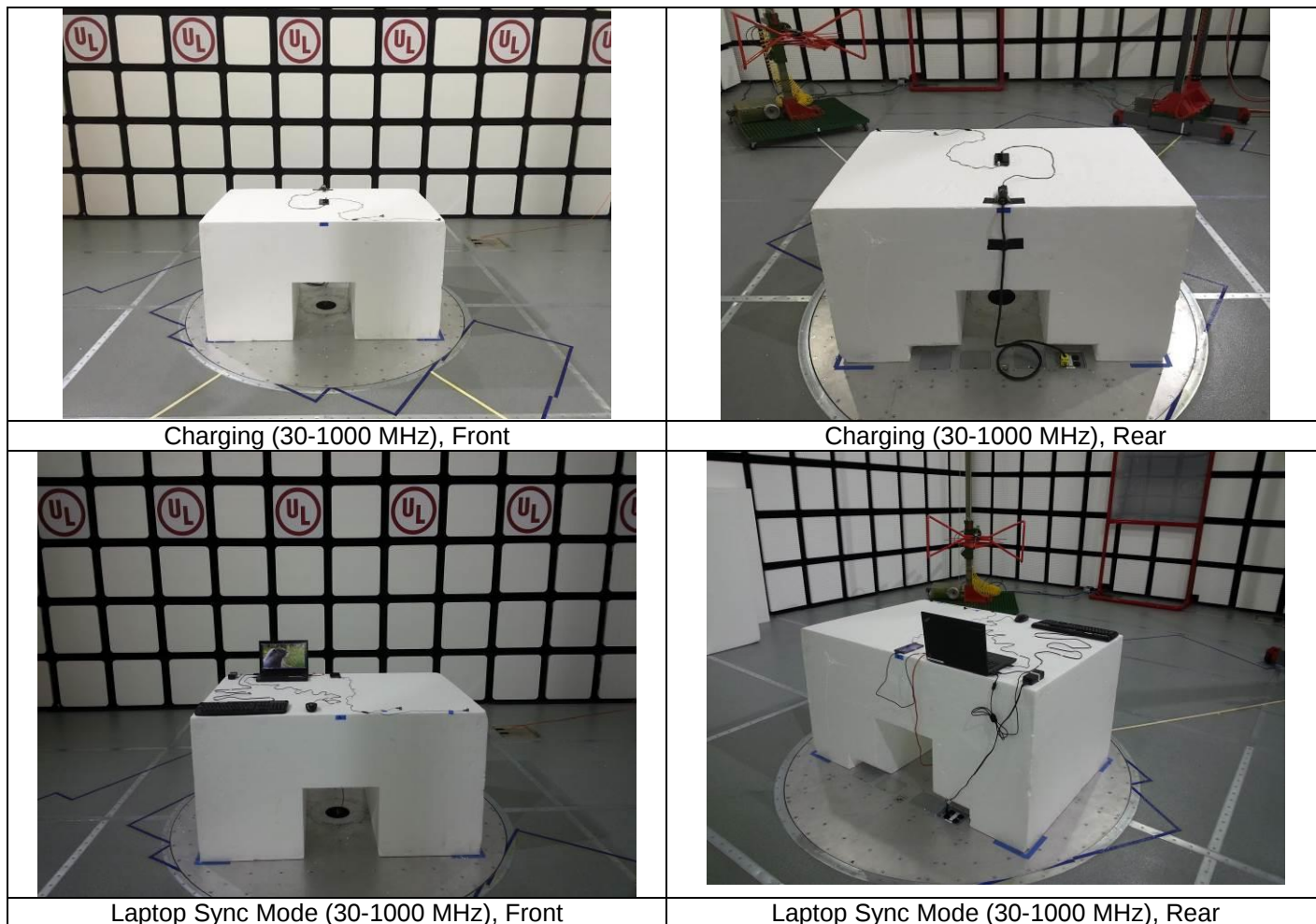
Figure 4 Test setup for Radiated Emissions < 1GHz
