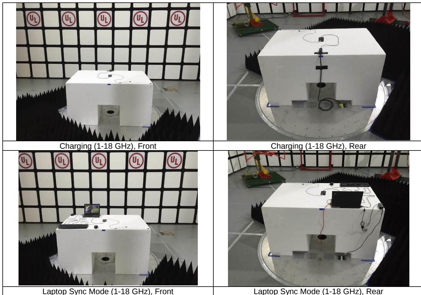
Figure 5 Test setup for Radiated Emissions > 1GHz
