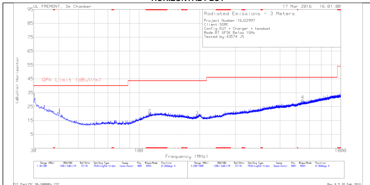
HORIZONTAL PLOT
