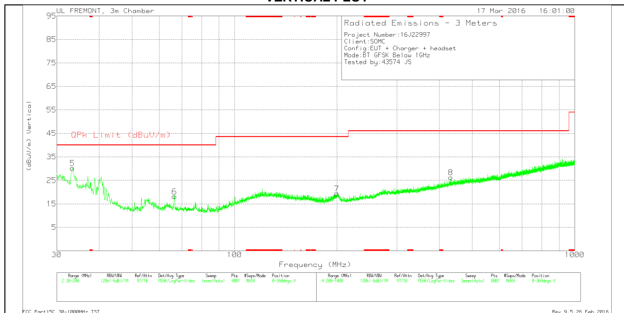
VERTICAL PLOT
