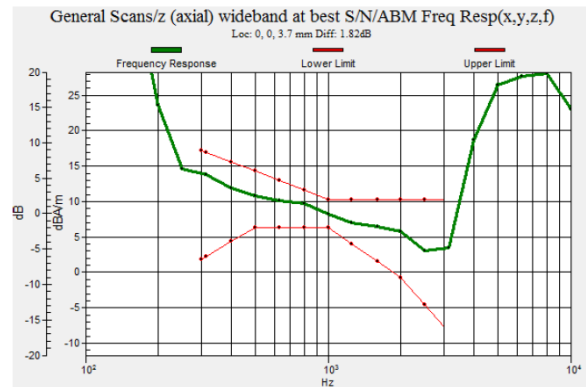
Fig 7.2 GSM1900 Ch661
