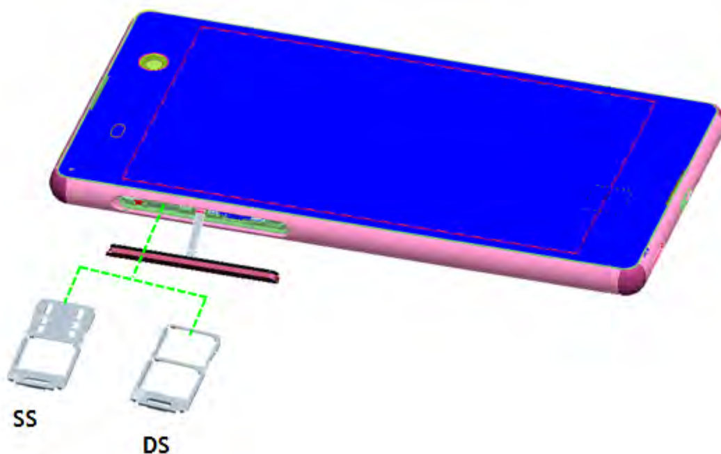
Fig.20 SIM Tray difference
