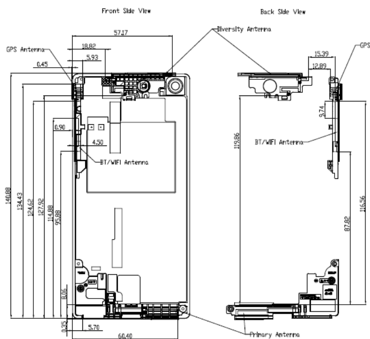
Fig.19 Antenna position of EUT
