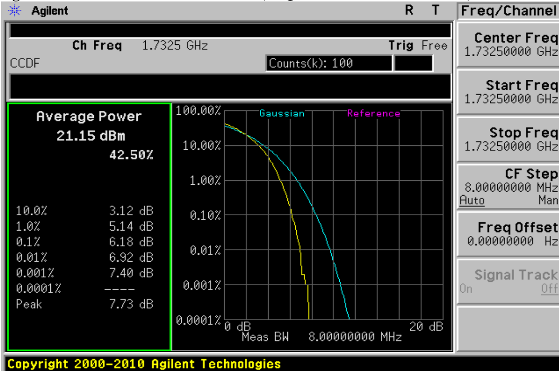
Figure 13-74: 10MHz BW LTE-Band 4(16QAM Number: 50 Offset: 0) Channel Mid
