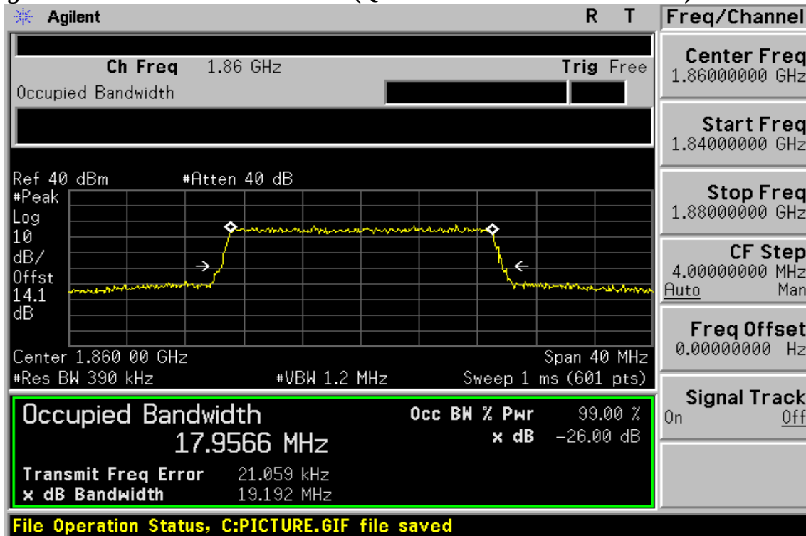
Figure 8-67: 20MHz BW LTE-Band 2(QPSK RB Number: 100 Offset: 0) Channel Low
