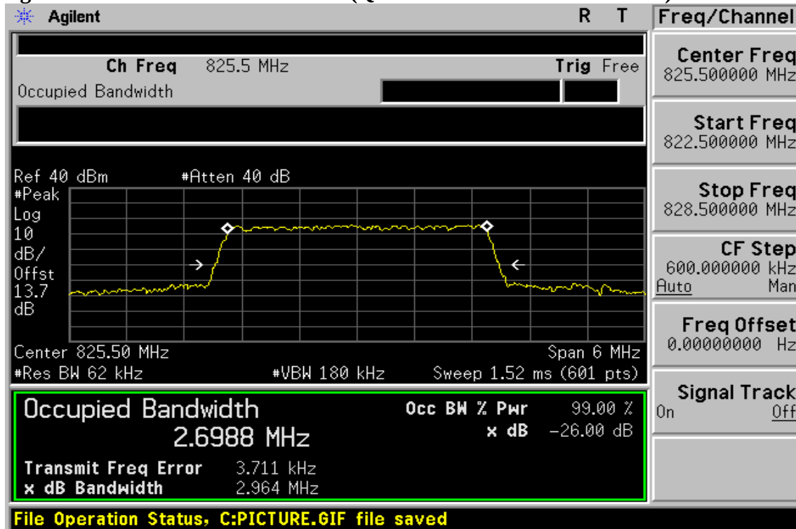
Figure 8-79: 3MHz BW LTE-Band 5(QPSK RB Number: 15 Offset: 0) Channel Low
