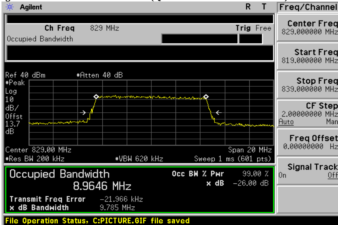
Figure 8-91: 10MHz BW LTE-Band 5(QPSK RB Number: 50 Offset: 0) Channel Low
