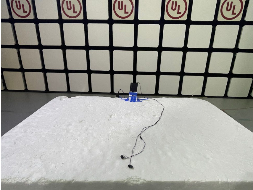
RADIATED PHOTO (30-1000MHz NFC)
