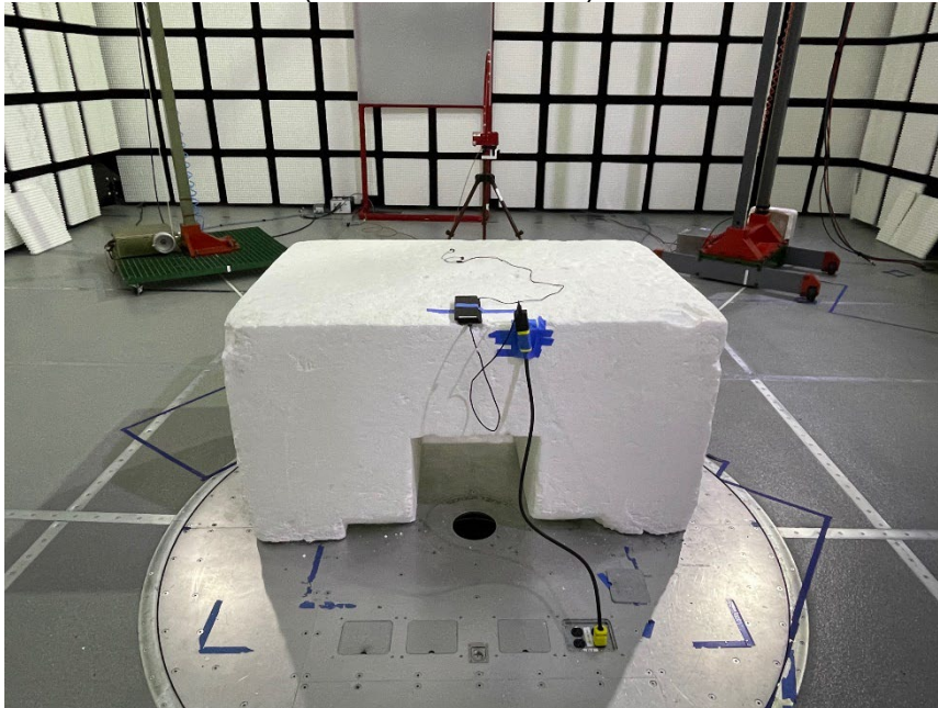
RADIATED PHOTO (0.009-30MHz WPT)
