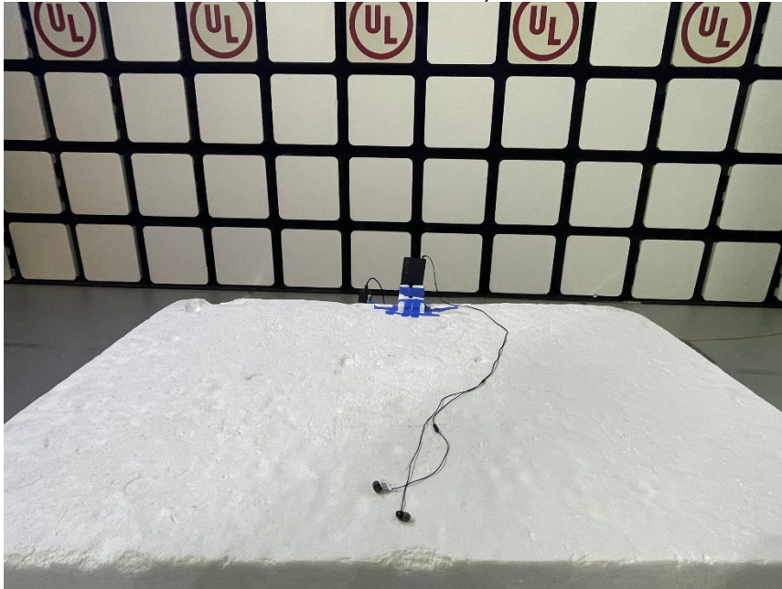
RADIATED PHOTO (0.009-30MHz NFC)
