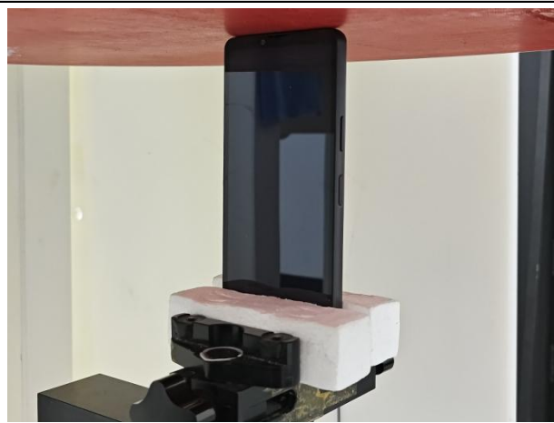
Photo 21: Top Side 0mm(NFC)
