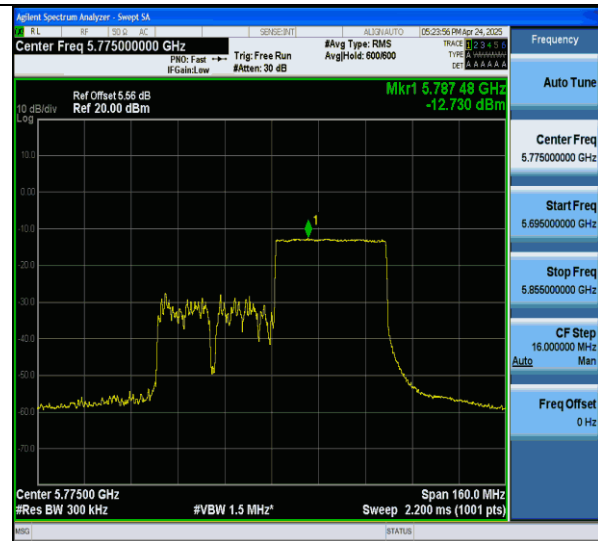
11ax80MIMO-Ant7-5775-484Tone-RU66-PASS
