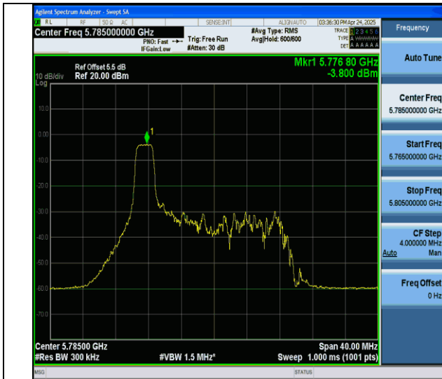
11ax20MIMO-Ant6-5785-26Tone-RU0-PASS
