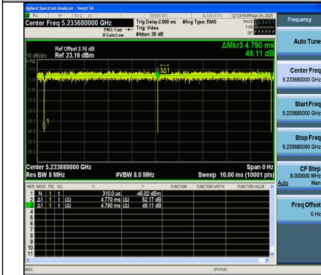
NTNV-11ax20MIMO-Ant6-5240-106Tone-RU53
