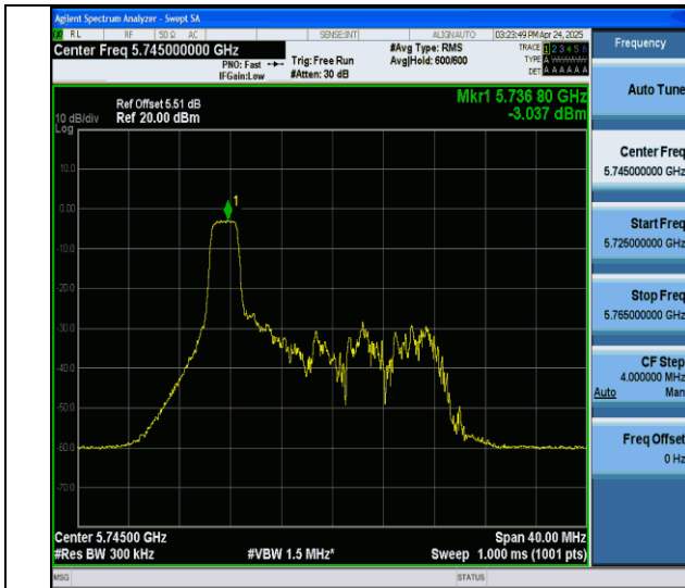
11ax20MIMO-Ant6-5745-26Tone-RU0-PASS
