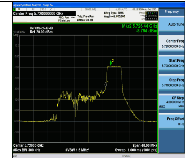
11ax20MIMO-Ant6-5720 UNII-3-52Tone-RU40-PASS
