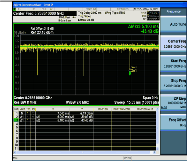
NTVN-11ax20MIMO-Ant7-5260-26Tone-RU8
