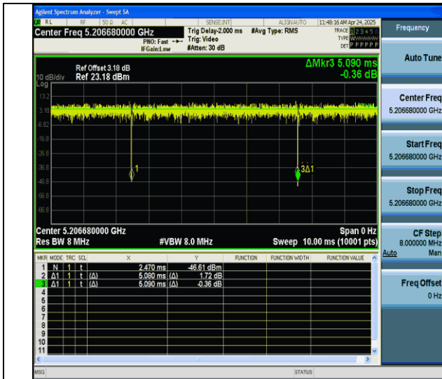
NTNV-11ax20MIMO-Ant6-5200-52Tone-RU40
