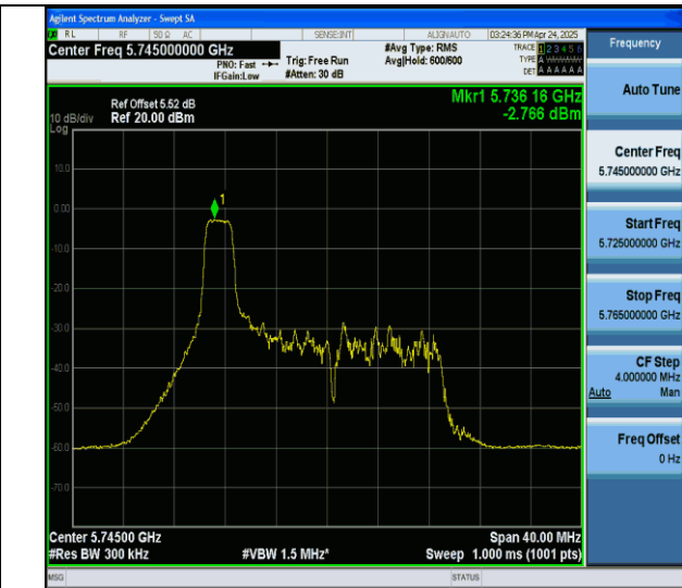
11ax20MIMO-Ant7-5745-26Tone-RU0-PASS
