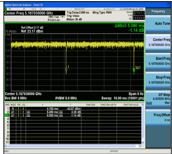
NTNV-11ax20MIMO-Ant7-5180-52Tone-RU40
