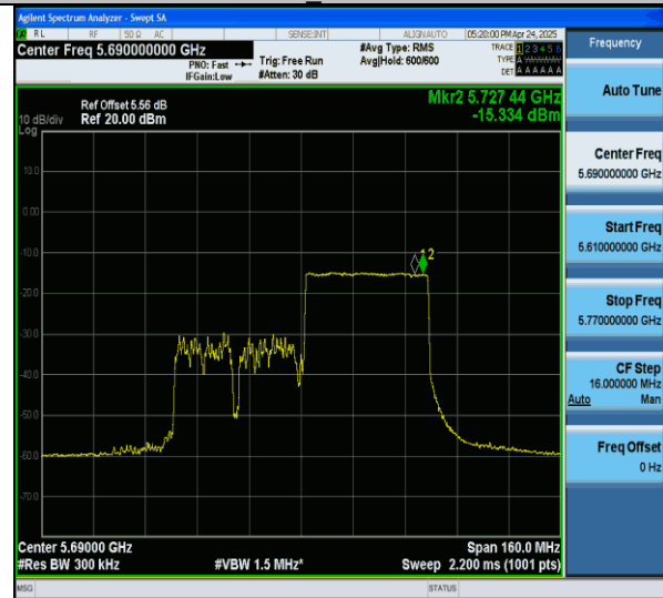
11ax80MIMO-Ant7-5690 UNII-3-484Tone-RU66-PASS
