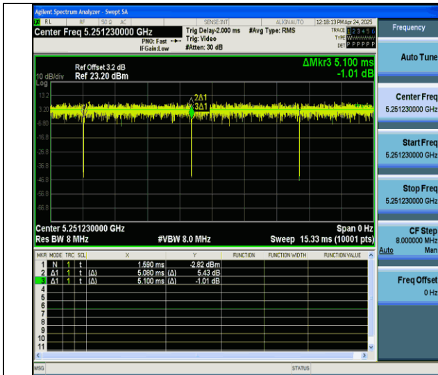
NTVN-11ax20MIMO-Ant6-5260-26Tone-RU0
