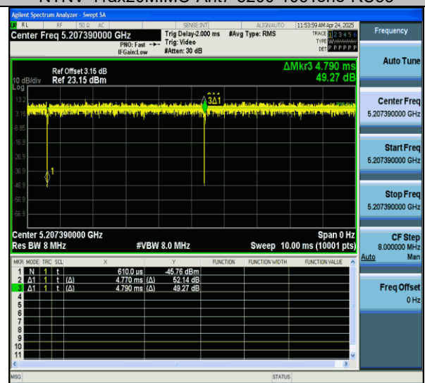
NTNV-11ax20MIMO-Ant7-5200-106Tone-RU54
