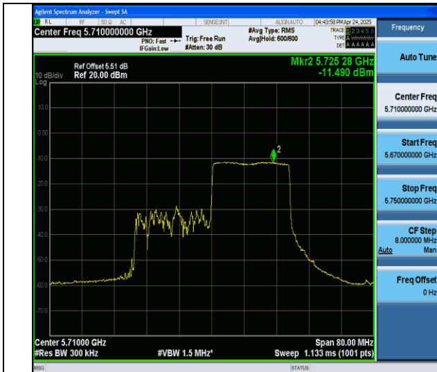
11ax40MIMO-Ant6-5710 UNII-3-242Tone-RU62-PASS
