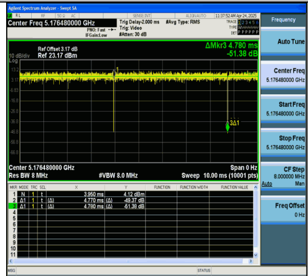
NTNV-11ax20MIMO-Ant7-5180-106Tone-RU53
