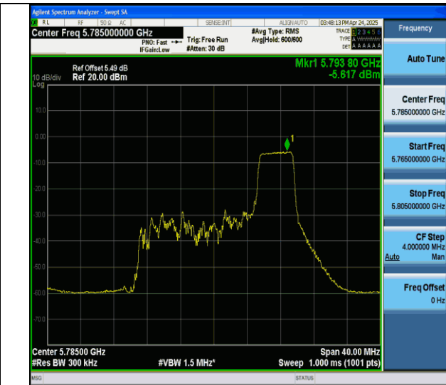
11ax20MIMO-Ant7-5785-52Tone-RU40-PASS
