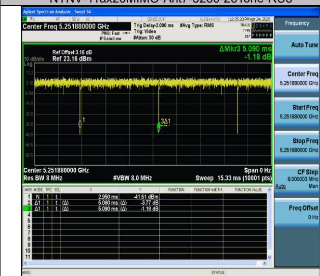
NTVN-11ax20MIMO-Ant7-5260-52Tone-RU37
