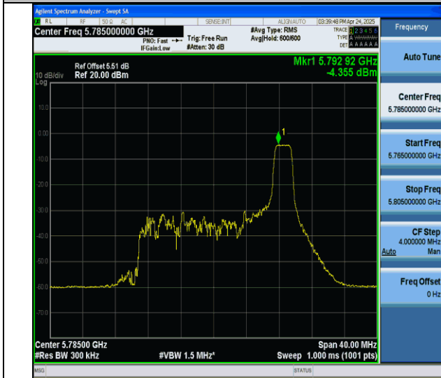
11ax20MIMO-Ant6-5785-26Tone-RU8-PASS
