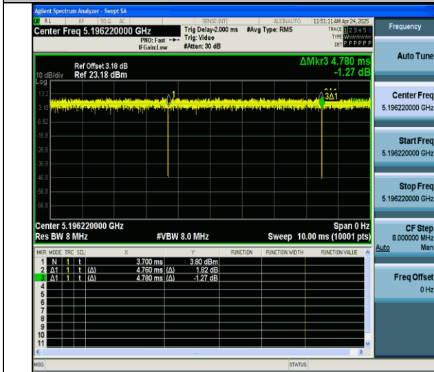
NTNV-11ax20MIMO-Ant6-5200-106Tone-RU53
