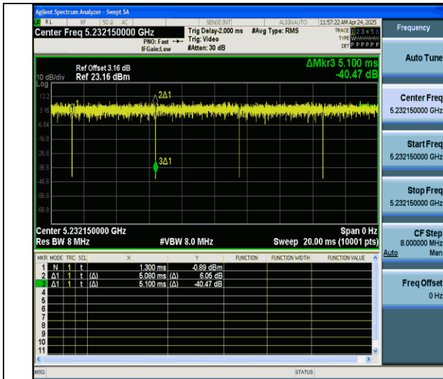
NTVN-11ax20MIMO-Ant6-5240-26Tone-RU0
