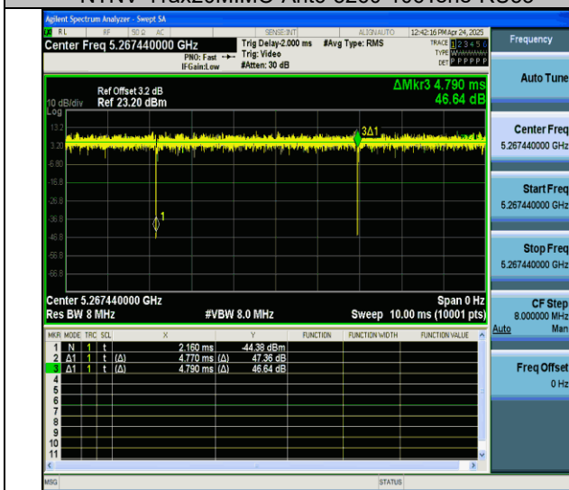
NTNV-11ax20MIMO-Ant6-5260-106Tone-RU54
