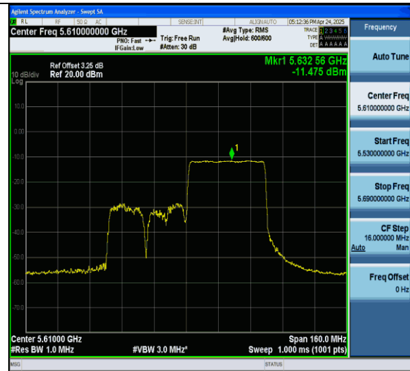
11ax80MIMO-Ant7-5610-484Tone-RU66-PASS
