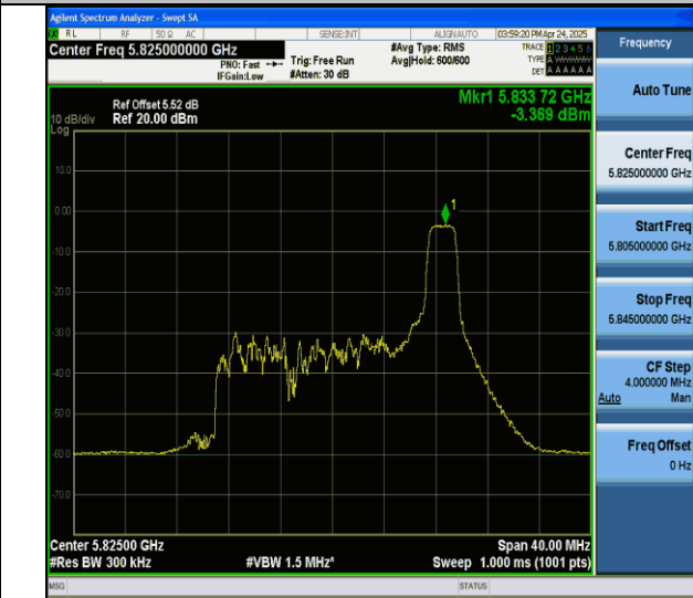
11ax20MIMO-Ant7-5825-26Tone-RU8-PASS
