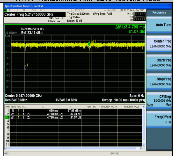
NTNV-11ax20MIMO-Ant7-5240-106Tone-RU54
