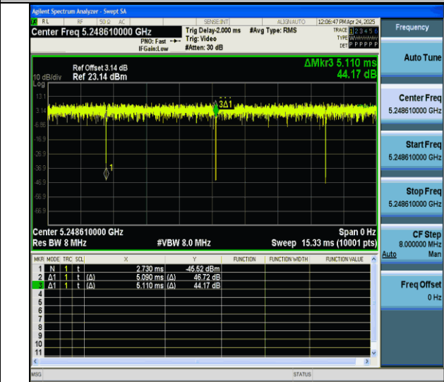
NTVN-11ax20MIMO-Ant7-5240-26Tone-RU8
