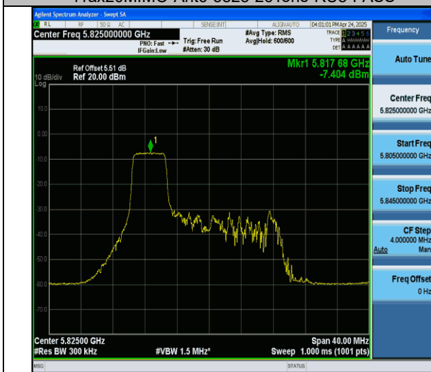
11ax20MIMO-Ant6-5825-52Tone-RU37-PASS
