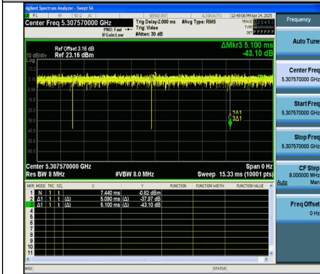
NTVN-11ax20MIMO-Ant6-5300-26Tone-RU8
