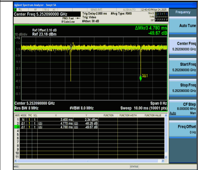
NTNV-11ax20MIMO-Ant7-5260-106Tone-RU53
