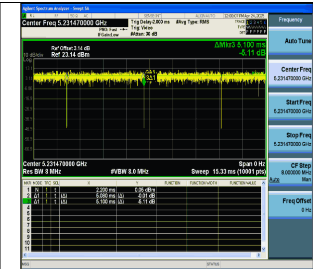
NTVN-11ax20MIMO-Ant7-5240-26Tone-RU0
