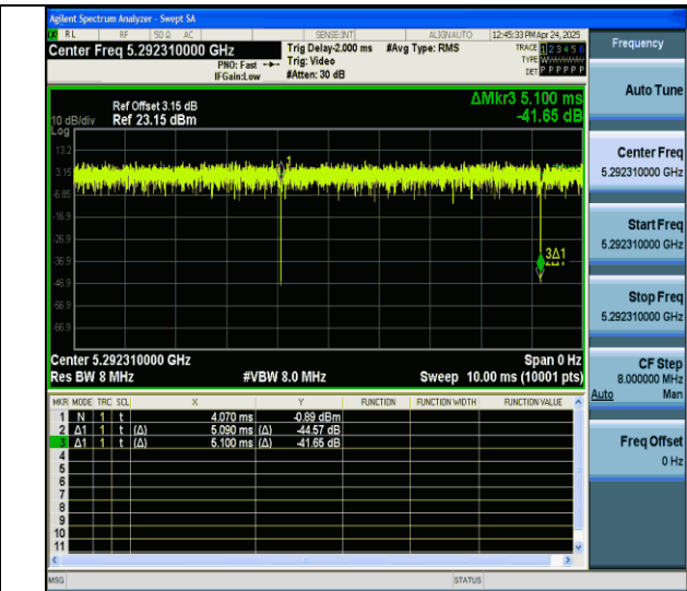
NTVN-11ax20MIMO-Ant7-5300-26Tone-RU0
