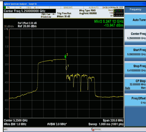
11ax160MIMO-Ant7-5250 UNII-1-996Tone-RU67-PASS
