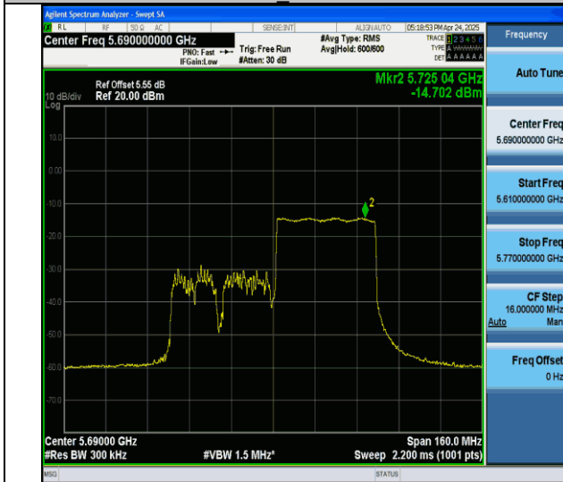
11ax80MIMO-Ant6-5690 UNII-3-484Tone-RU66-PASS
