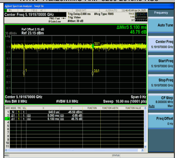
NTVN-11ax20MIMO-Ant7-5200-52Tone-RU37
