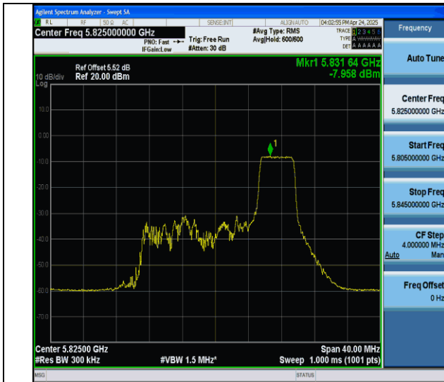
11ax20MIMO-Ant6-5825-52Tone-RU40-PASS
