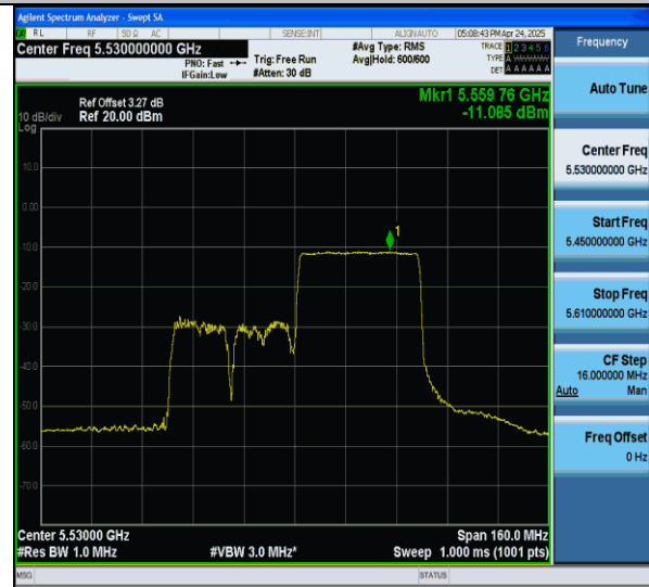
11ax80MIMO-Ant7-5530-484Tone-RU66-PASS
