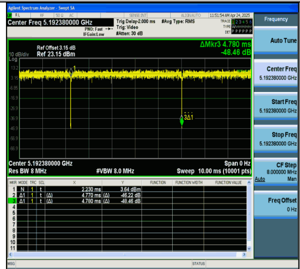
NTNV-11ax20MIMO-Ant7-5200-106Tone-RU53
