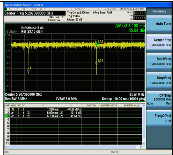
NTNV-11ax20MIMO-Ant7-5200-52Tone-RU40
