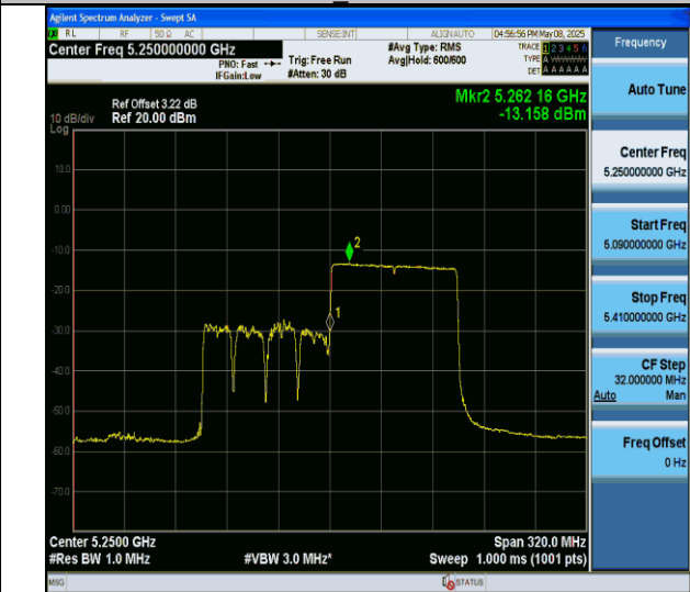
11ax160MIMO-Ant6-5250 UNII-2A-996Tone-RU68-PASS
