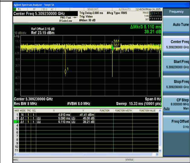
NTVN-11ax20MIMO-Ant7-5300-26Tone-RU8
