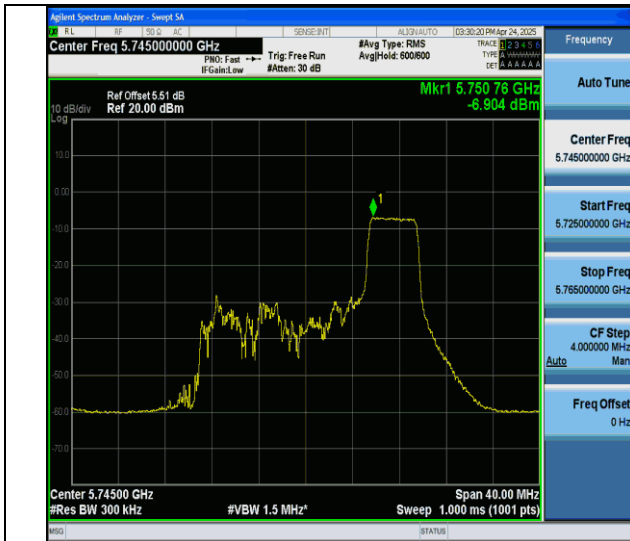
11ax20MIMO-Ant6-5745-52Tone-RU40-PASS
