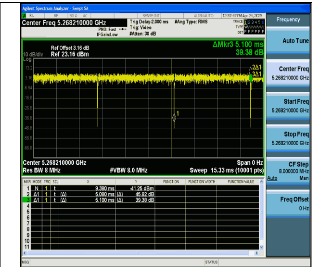
NTNV-11ax20MIMO-Ant7-5260-52Tone-RU40
