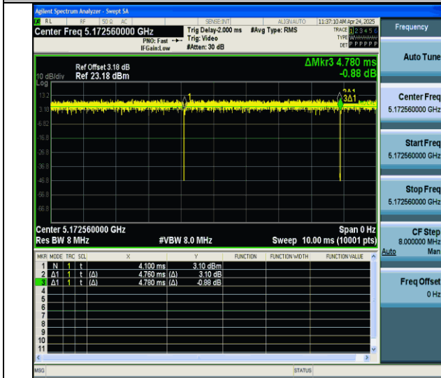
NTNV-11ax20MIMO-Ant6-5180-106Tone-RU53
