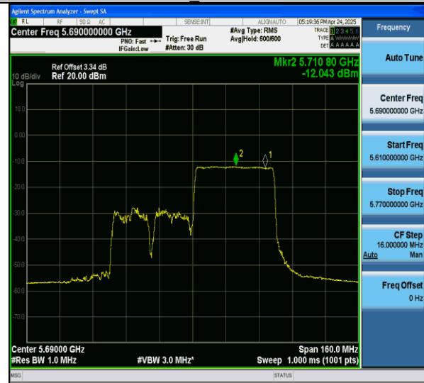
11ax80MIMO-Ant7-5690_UHII-2C-484Tone-RU66-PASS
