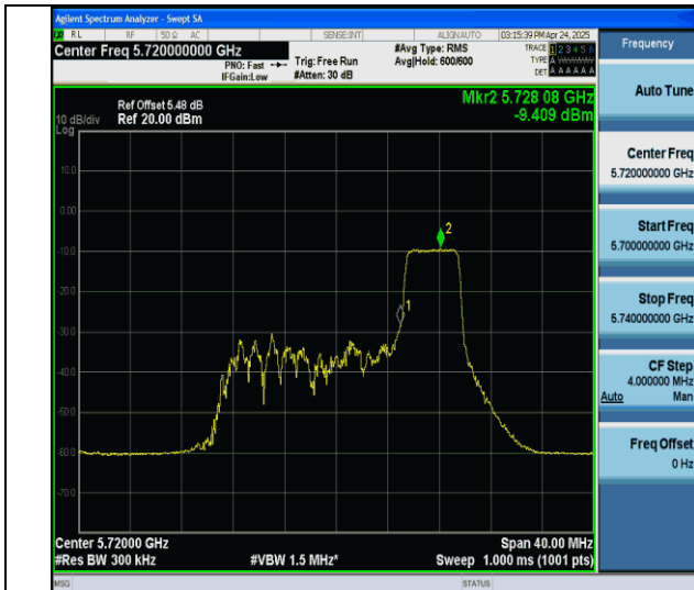
11ax20MIMO-Ant7-5720 UNII-3-52Tone-RU40-PASS
