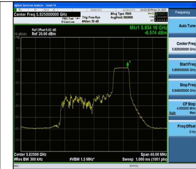
11ax20MIMO-Ant7-5825-52Tone-RU40-PASS
