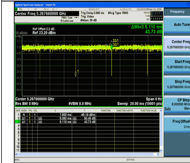
NTVN-11ax20MIMO-Ant6-5260-26Tone-RU8
