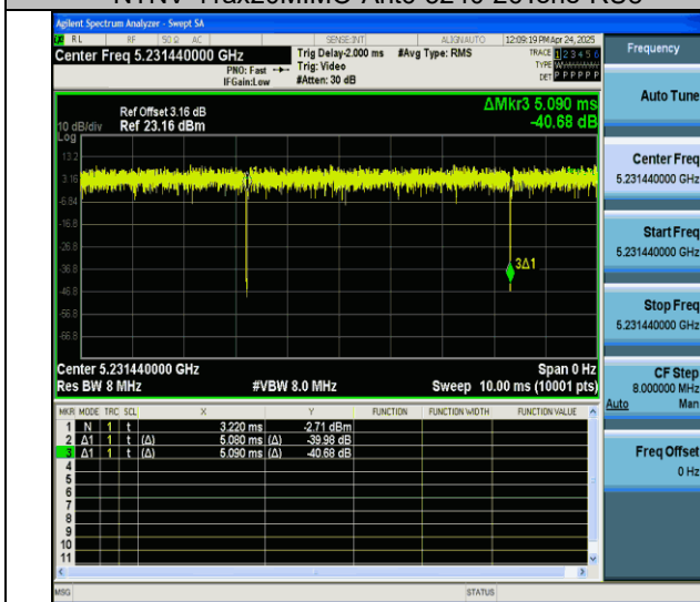
NTVN-11ax20MIMO-Ant6-5240-52Tone-RU37
