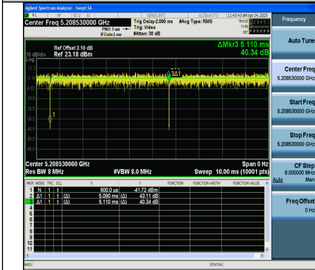
NTVN-11ax20MIMO-Ant6-5200-26Tone-RU8
