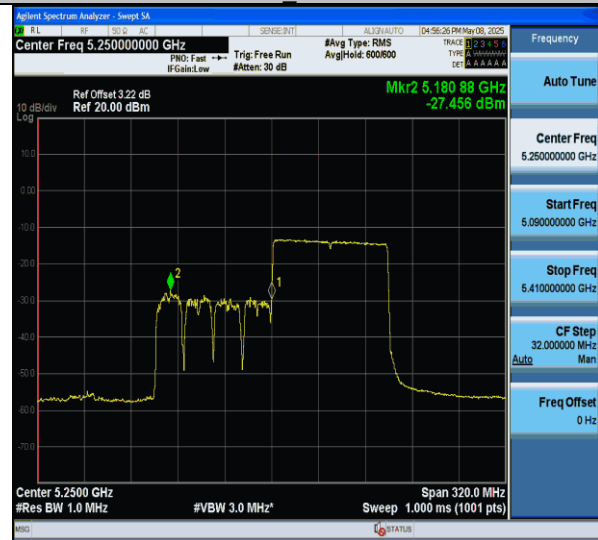
11ax160MIMO-Ant6-5250 UNII-1-996Tone-RU68-PASS
