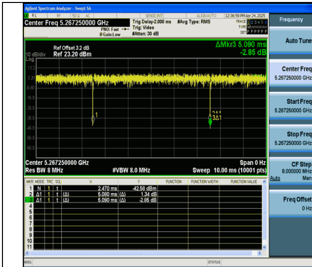
NTNV-11ax20MIMO-Ant6-5260-52Tone-RU40
