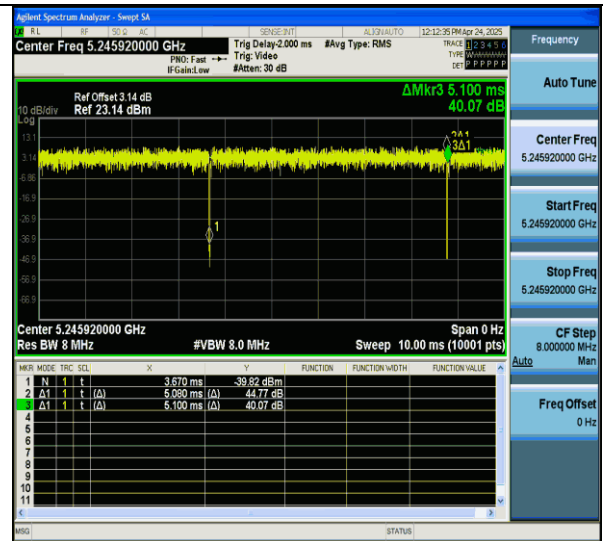
NTNV-11ax20MIMO-Ant7-5240-52Tone-RU40
