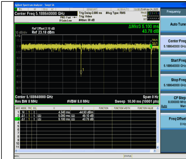
NTNV-11ax20MIMO-Ant6-5180-52Tone-RU40
