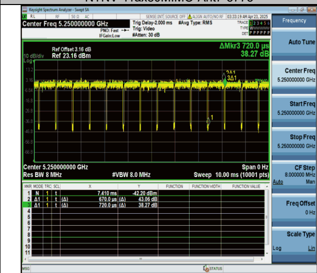
NTVN-11ax160MIMO-Ant7-5250
