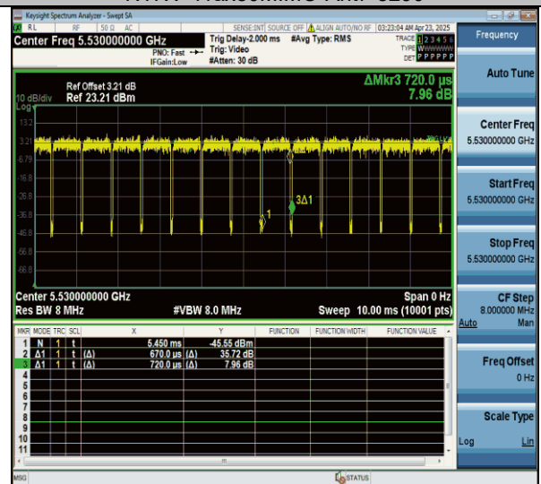
NTVN-11ax80MIMO-Ant7-5530
