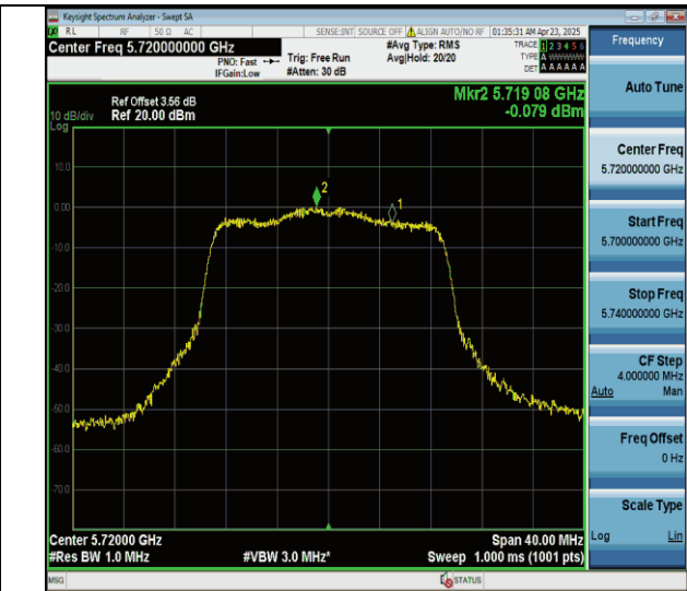
11n20MIMO-Ant7-5720 UNII-2C-PASS
