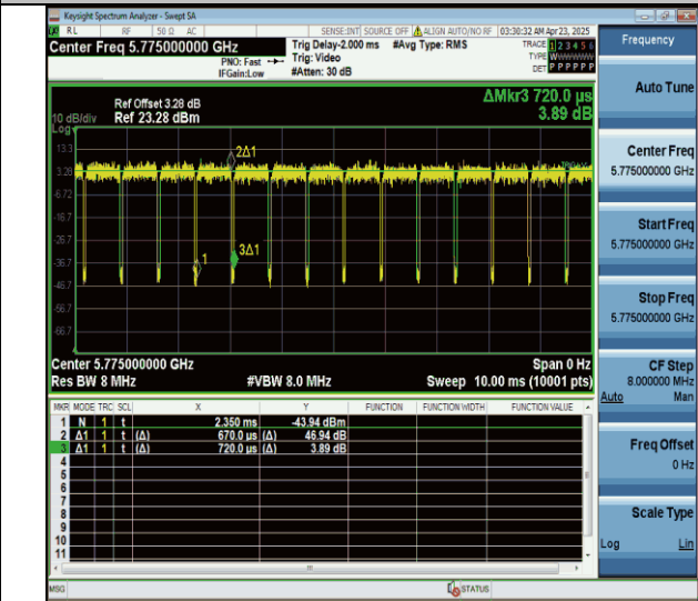
NTVN-11ax80MIMO-Ant7-5775
