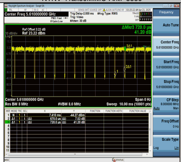
NTVN-11ax80MIMO-Ant7-5610
