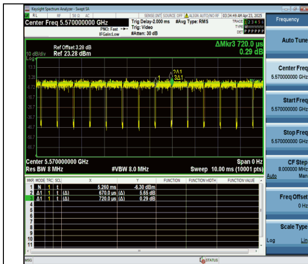
NTNV-11ax160MIMO-Ant6-5570
