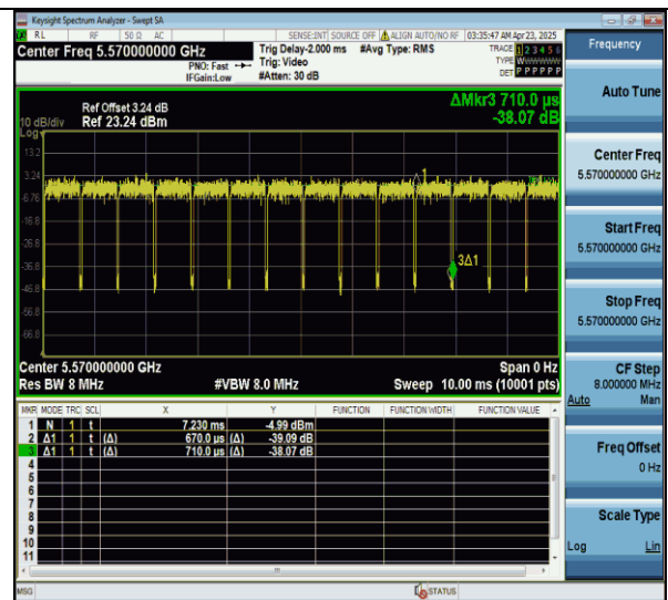
NTNV-11ax160MIMO-Ant7-5570
