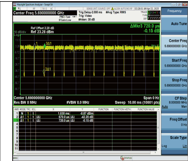
NTVN-11ax80MIMO-Ant7-5690
