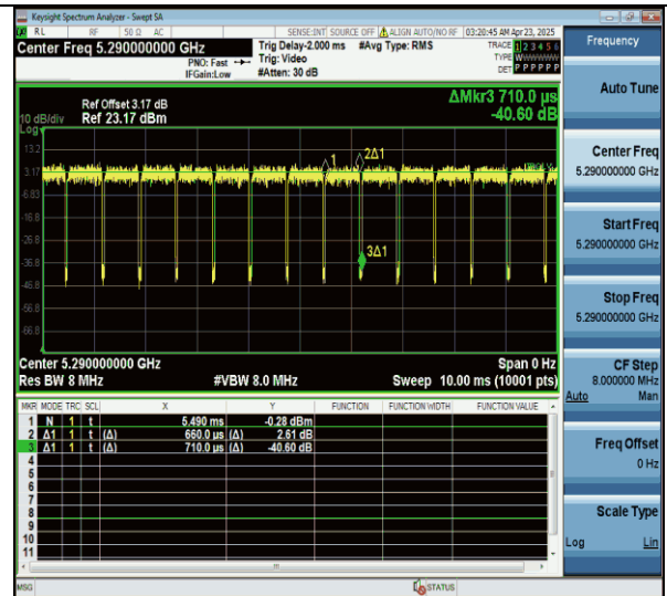
NTVN-11ax80MIMO-Ant7-5290
