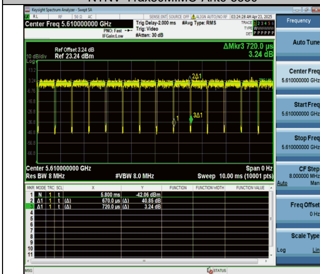
NTVN-11ax80MIMO-Ant6-5610
