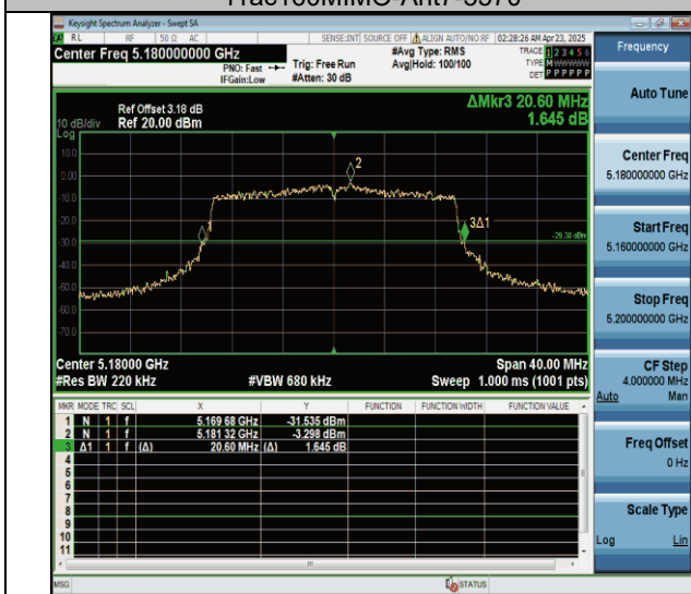
11ax20MIMO-Ant6-5180
