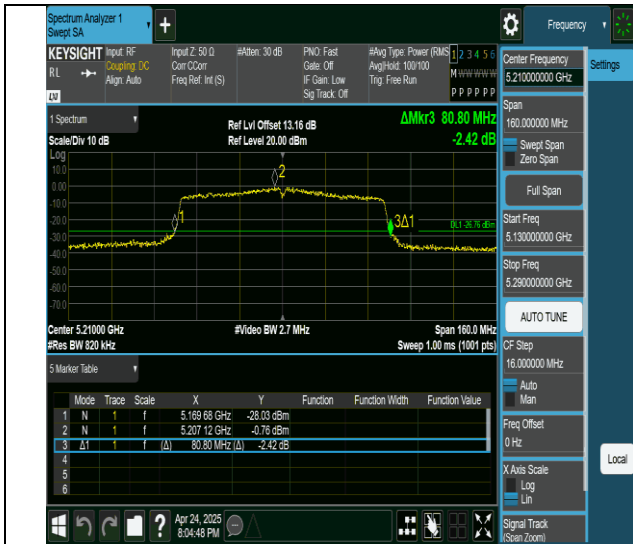
11ac80MIMO-Ant6-5210
