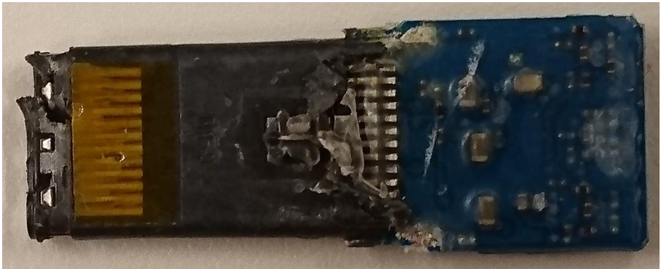
USB (Rear)
