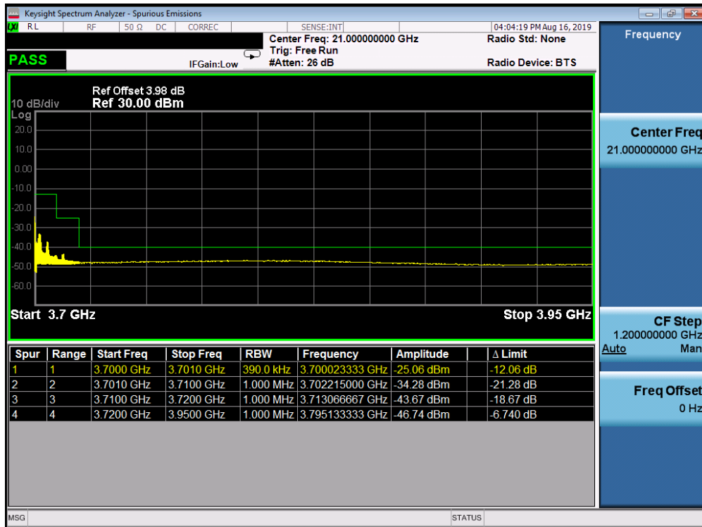
Plot 7-25. Conducted Spurious Plot (LTE Band 48 - 20.0MHz QPSK - RB Size 1, RB Offset 0 - High Channel)
