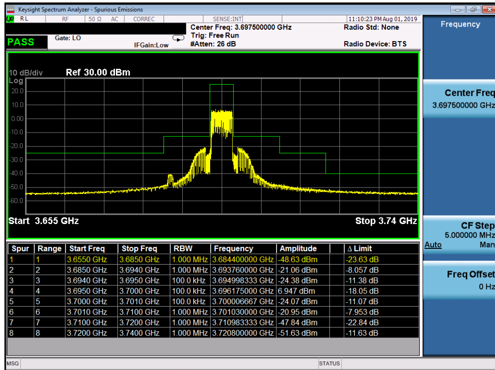
Plot 7-30. Upper ACP Plot (LTE Band 48 - 5.0MHz QPSK - Full RB Configuration)
