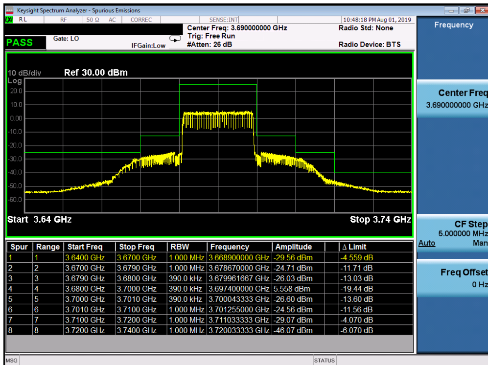
Plot 7-39. Upper ACP Plot (LTE Band 48 - 20.0MHz QPSK - Full RB Configuration)
