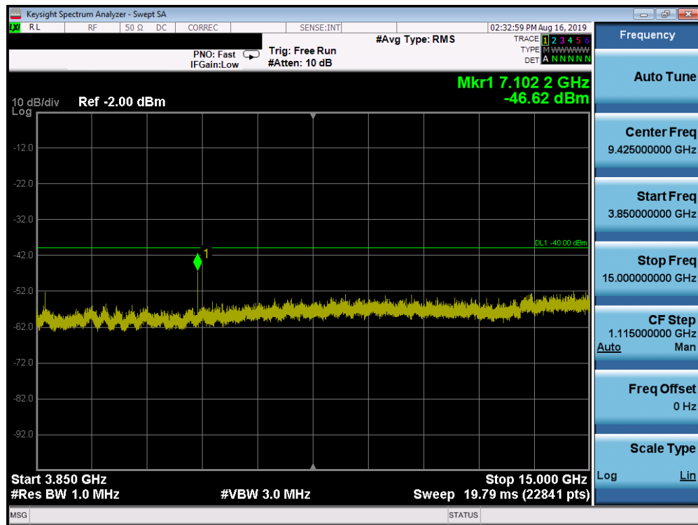
Plot 7-16. Conducted Spurious Plot (LTE Band 48 - 20.0MHz QPSK - RB Size 1, RB Offset 0 - Low Channel)
