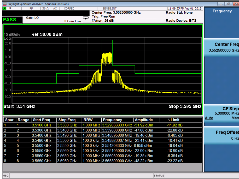
Plot 7-28. Lower ACP Plot (LTE Band 48 - 5.0MHz QPSK - Full RB Configuration)
