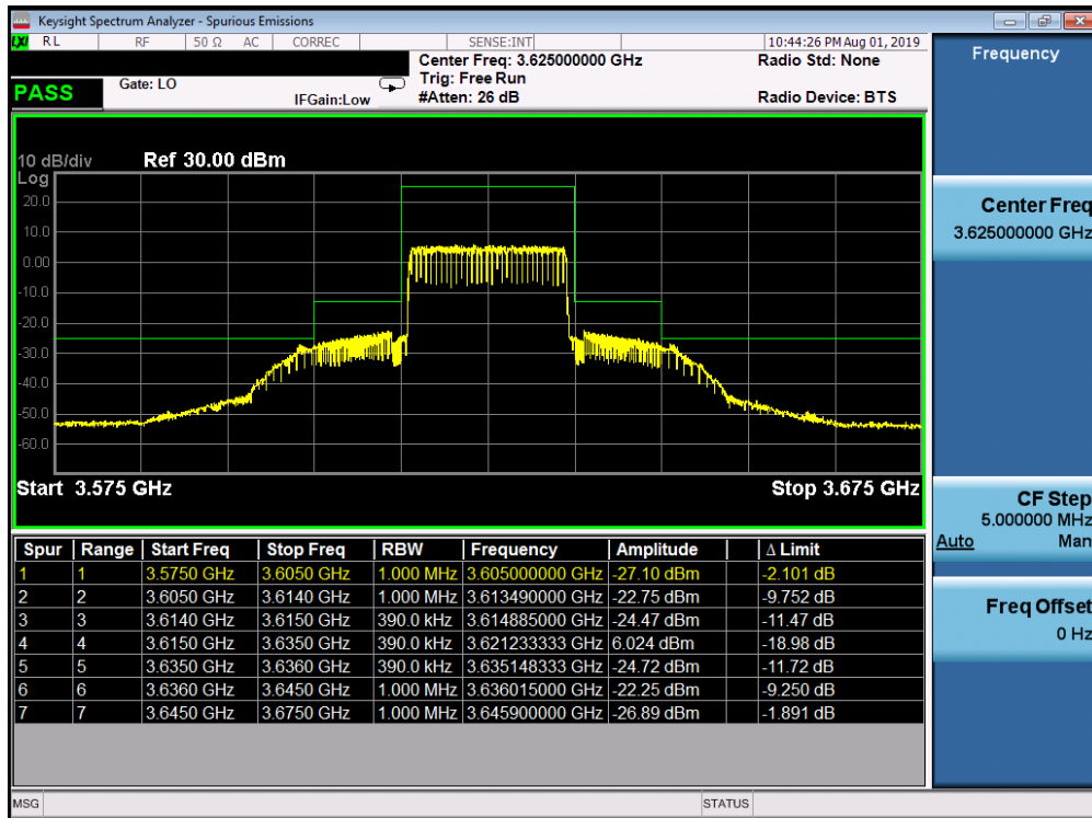
Plot 7-38. Mid ACP Plot (LTE Band 48 - 20.0MHz QPSK - Full RB Configuration)
