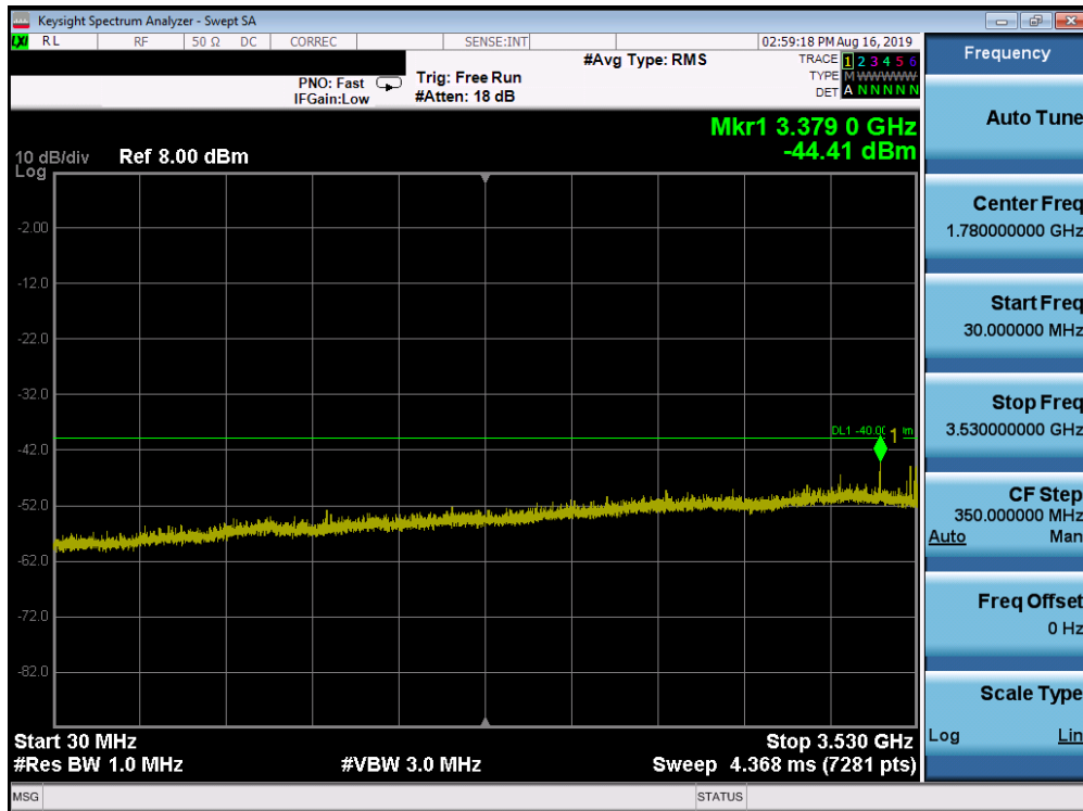
Plot 7-23. Conducted Spurious Plot (LTE Band 48 - 20.0MHz QPSK - RB Size 1, RB Offset 0 - High Channel)
