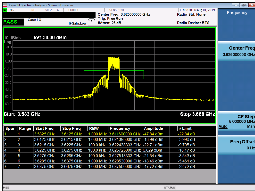
Plot 7-29. Mid ACP Plot (LTE Band 48 - 5.0MHz QPSK - Full RB Configuration)
