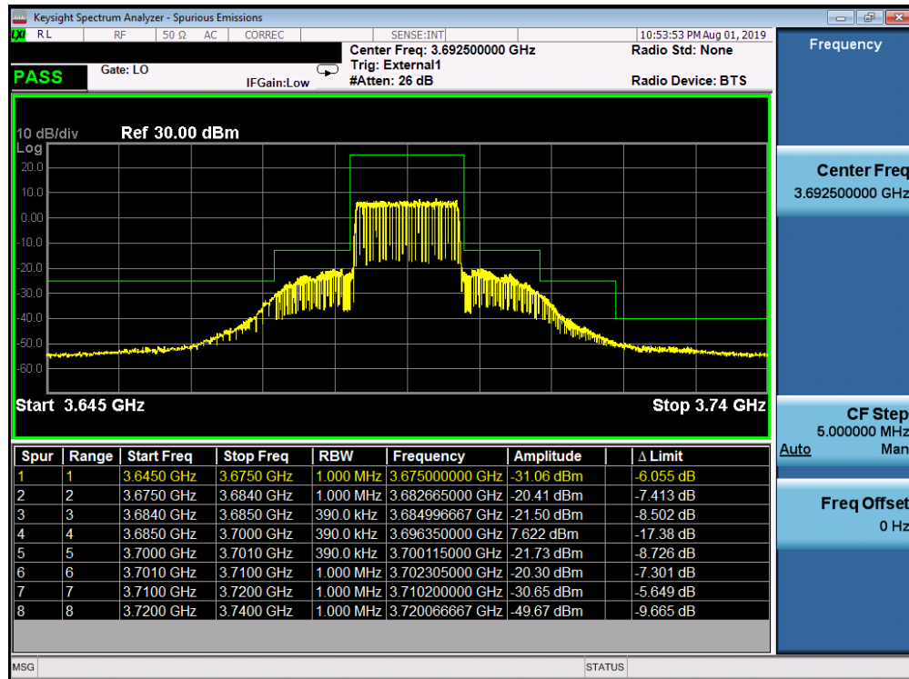
Plot 7-36. Upper ACP Plot (LTE Band 48 - 15.0MHz QPSK - Full RB Configuration)
