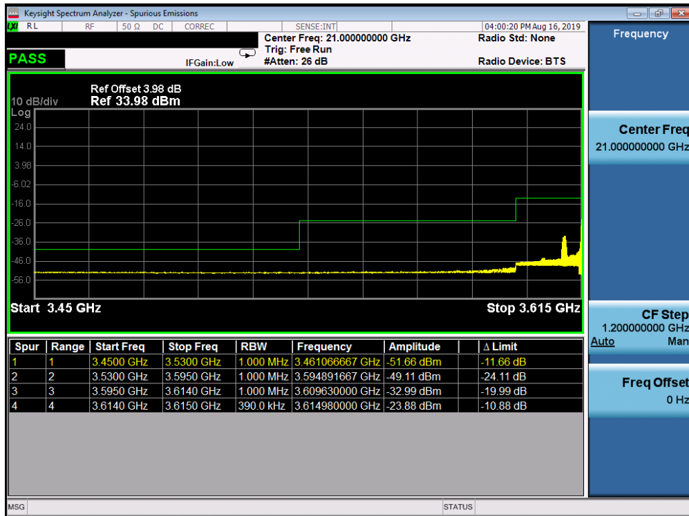
Plot 7-19. Conducted Spurious Plot (LTE Band 48 - 20.0MHz QPSK - RB Size 1, RB Offset 0 - Mid Channel)
