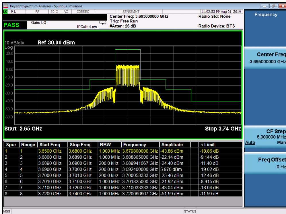
Plot 7-33. Upper ACP Plot (LTE Band 48 - 10.0MHz QPSK - Full RB Configuration)
