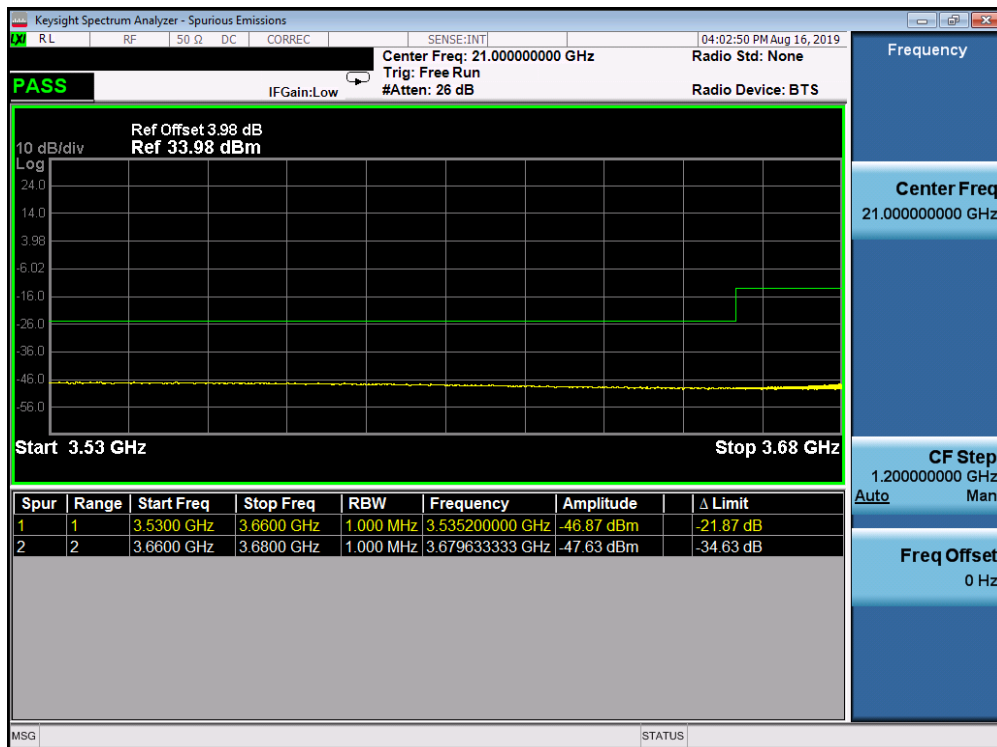
Plot 7-24. Conducted Spurious Plot (LTE Band 48 - 20.0MHz QPSK - RB Size 1, RB Offset 0 - High Channel)
