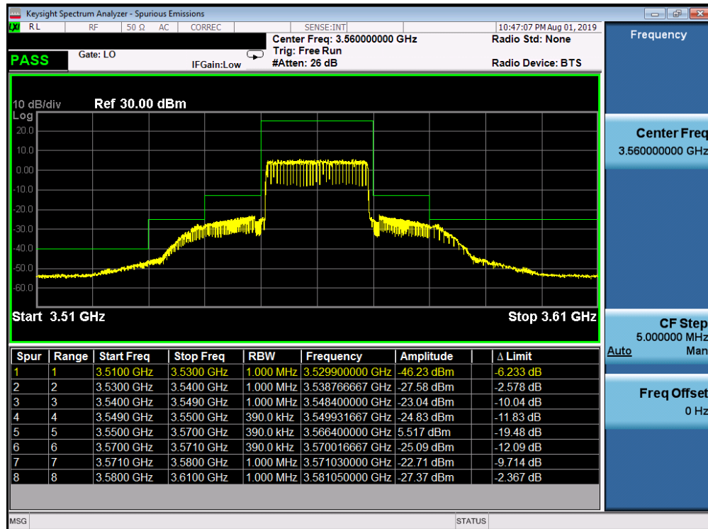
Plot 7-37. Lower ACP Plot (LTE Band 48 - 20.0MHz QPSK - Full RB Configuration)
