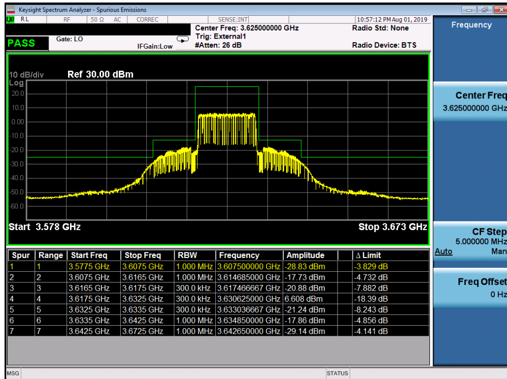
Plot 7-35. Mid ACP Plot (LTE Band 48 - 15.0MHz QPSK - Full RB Configuration)
