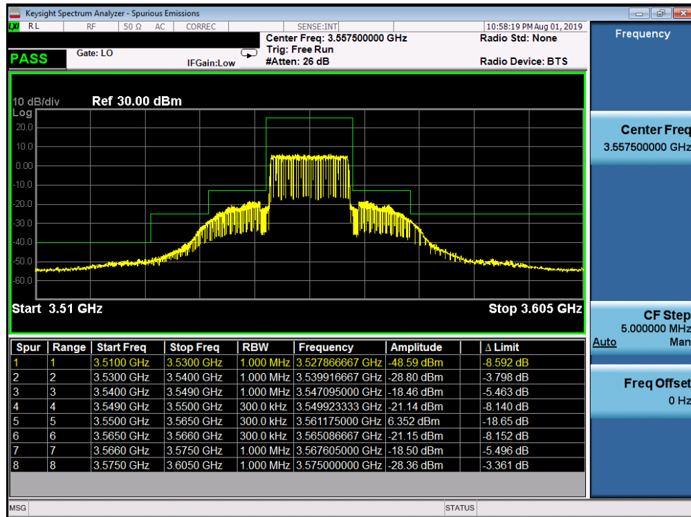
Plot 7-34. Lower ACP Plot (LTE Band 48 - 15.0MHz QPSK - Full RB Configuration)
