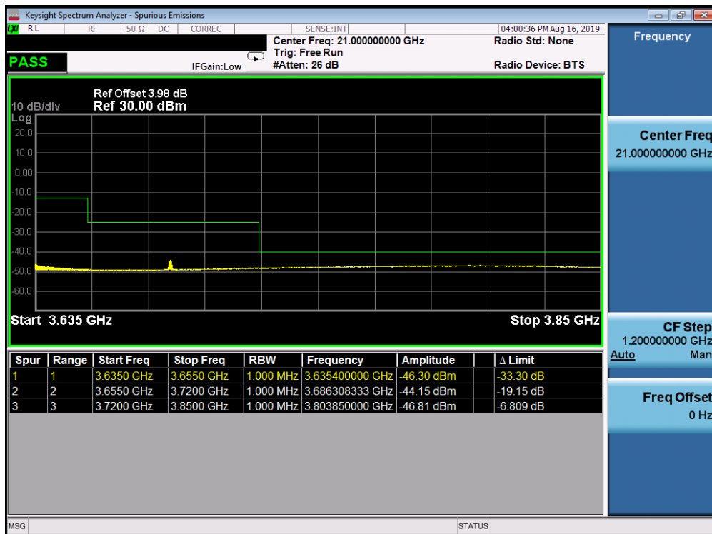
Plot 7-20. Conducted Spurious Plot (LTE Band 48 - 20.0MHz QPSK - RB Size 1, RB Offset 0 - Mid Channel)
