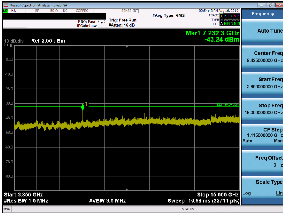
Plot 7-21. Conducted Spurious Plot (LTE Band 48 - 20.0MHz QPSK - RB Size 1, RB Offset 0 - Mid Channel)
