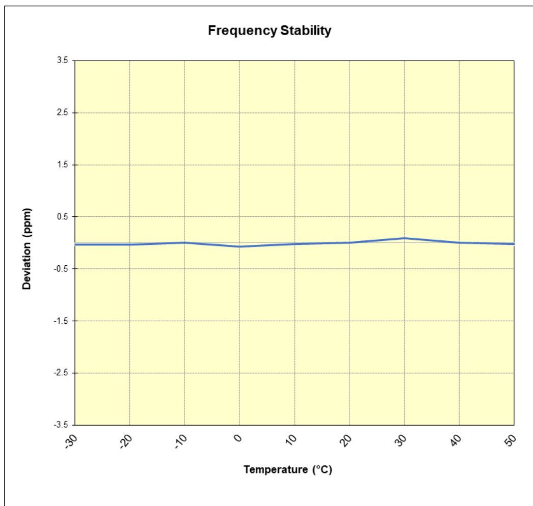
Figure 7-6. Frequency Stability Graph (LTE Band 48)
