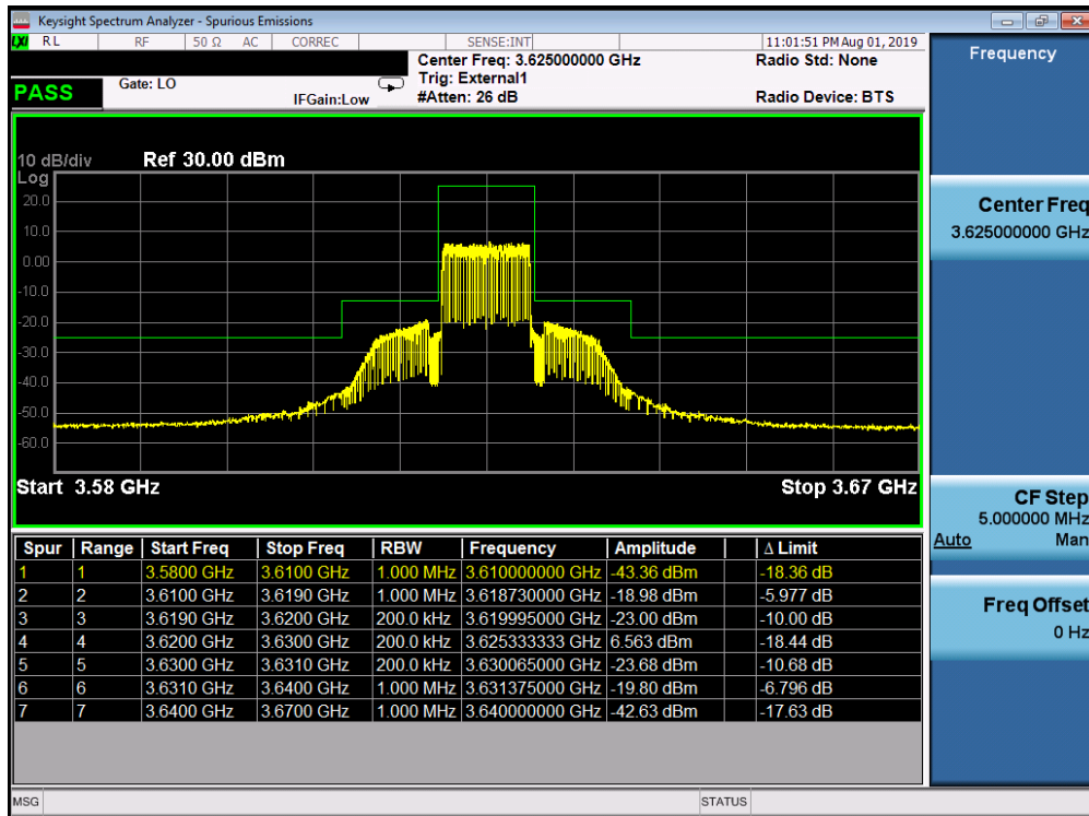
Plot 7-32. Mid ACP Plot (LTE Band 48 - 10.0MHz QPSK - Full RB Configuration)
