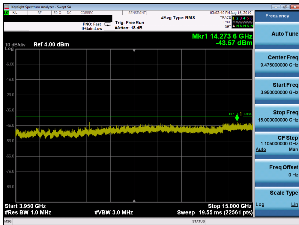
Plot 7-26. Conducted Spurious Plot (LTE Band 48 - 20.0MHz QPSK - RB Size 1, RB Offset 0 - High Channel)
