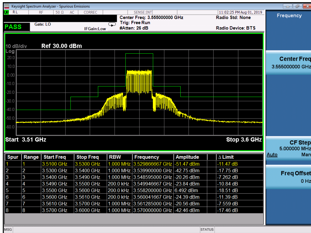
Plot 7-31. Lower ACP Plot (LTE Band 48 - 10.0MHz QPSK - Full RB Configuration)
