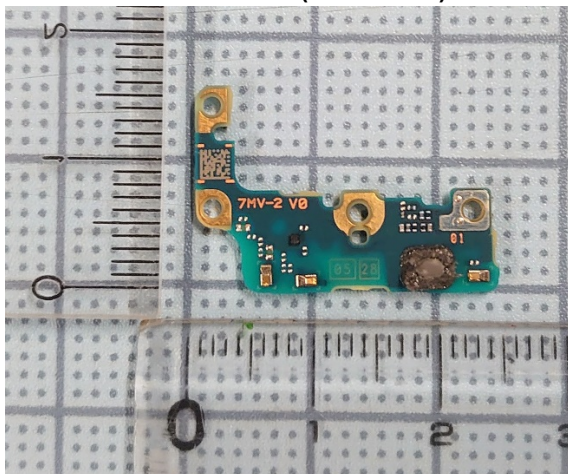
Internal Sub-PWB (Front-side)
