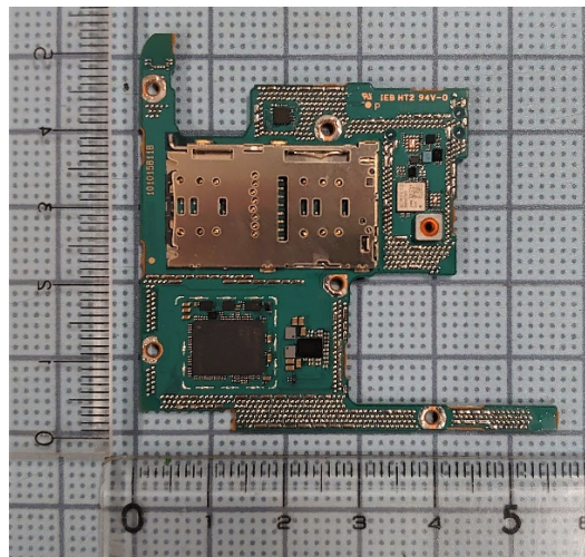
Internal Main-PWB Rear without Shield cases (Front-side)
