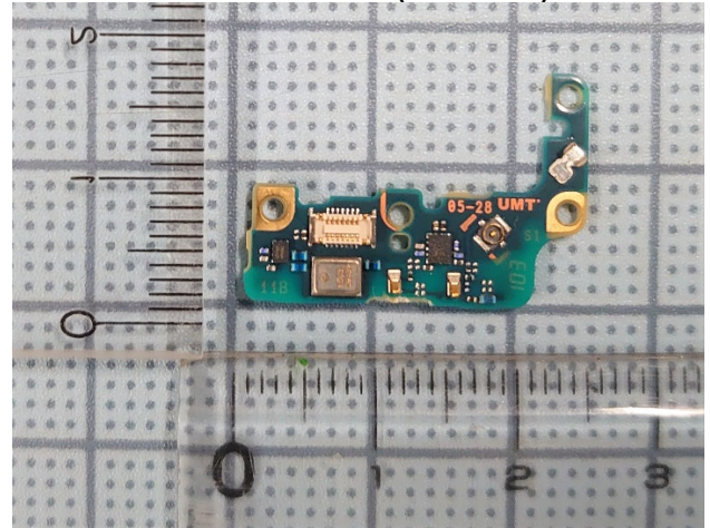
Internal Sub-PBA (Rear-side)
