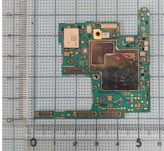
Internal Main-PWB Rear with Shield cases (Rear-side)
