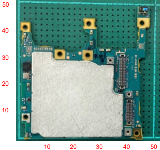
Internal Main-PWB Front with Shield cases(Front-side)
