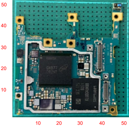
Internal Main-PWB Front without Shield cases (Front-side)
