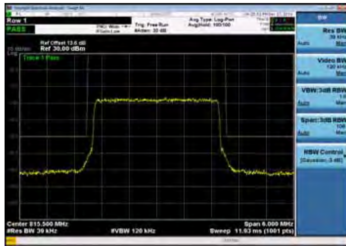
Emission Mask_Band26 for Part 90S_3M_QPSK_MID_RB15,0
