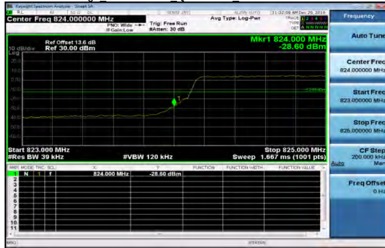
Band Edge Band5 3MHz QPSK 15 0 LowCH20415-825.5
