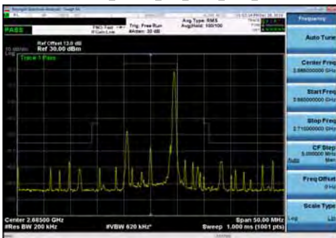
Emission Mask_Band 41_10M_QPSK_HIGH_RB1,49
