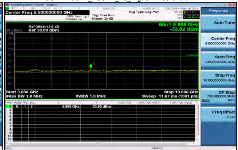
3GHz~10GHz HSUPA B5 HighCH4233-846.6
