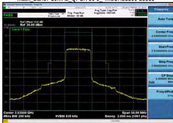
Mask Band7 10MHz QPSK 50 0 MidCH21100-25355
