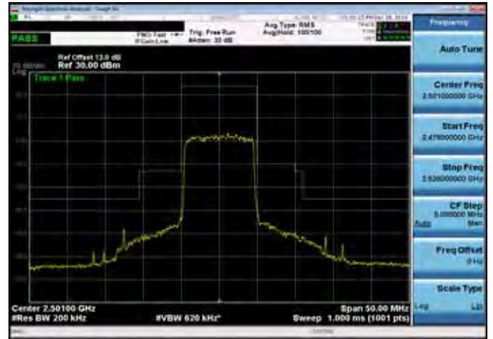
Emission Mask_Band 41_10M_QPSK_MID_RB50,0
