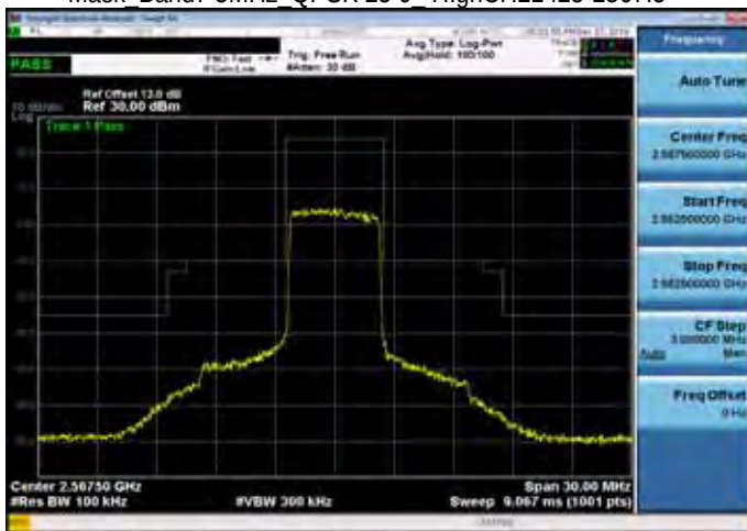
Mask Band7 5MHz QPSK 25 0 HighCH21425-2567.5
