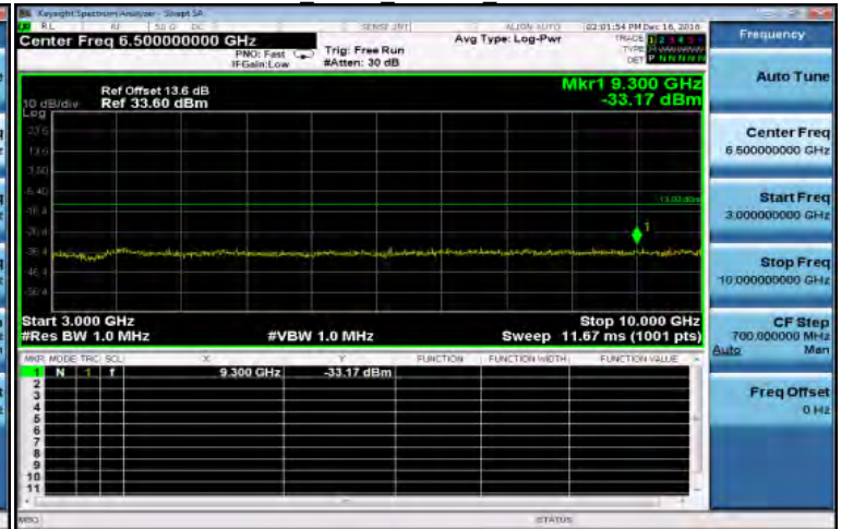
3GHz-10GHz EDGE 850MHz MidCH190-836.6
