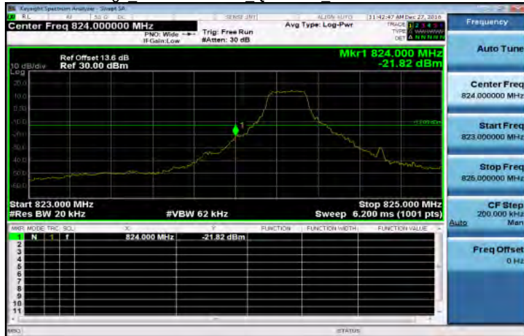
Band Edge Band26 1.4MHz QPSK 1 0 LowCH26797-824.7
