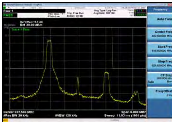
Emission Mask_Band26 for Part 90S_3M_QPSK_HIGH_RB1,0
