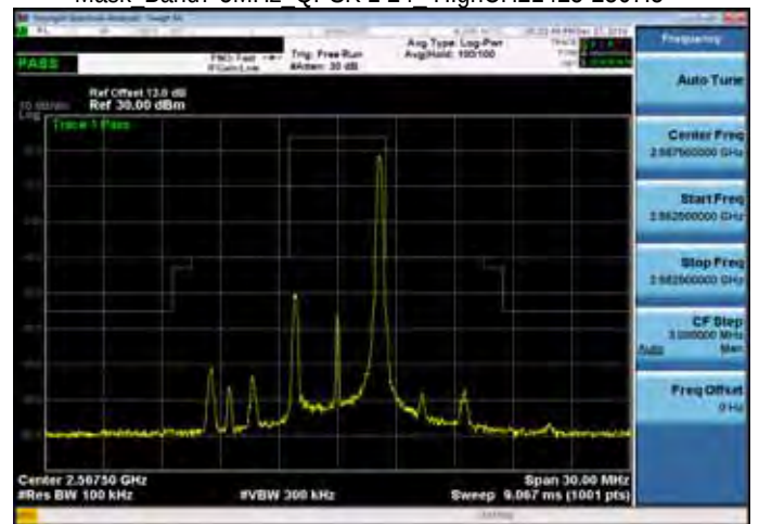
Mask Band7 5MHz QPSK 1 24 HighCH21425-2567.5
