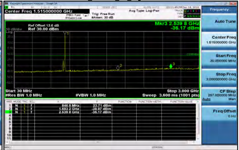
30MHz~3GHz HSDPA B5 HighCH4233-846.6
