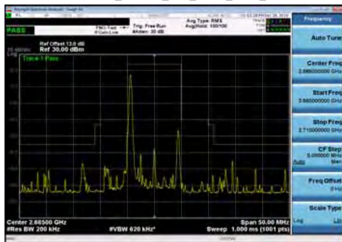
Emission Mask_Band 41_10M_QPSK_HIGH_RB1,0
