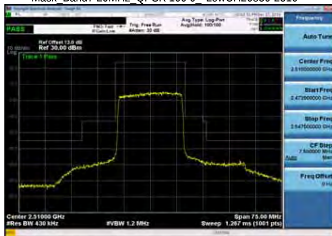
Mask Band7 20MHz_QPSK 100 0 LowCH20850-2510
