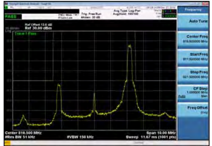
Emission Mask_Band26 for Part 90S_5M_QPSK_MID_RB1,24
