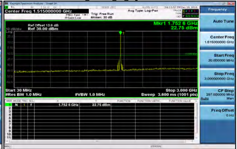
30MHz~3GHz HSUPA B4 HighCH1513-1752.6
