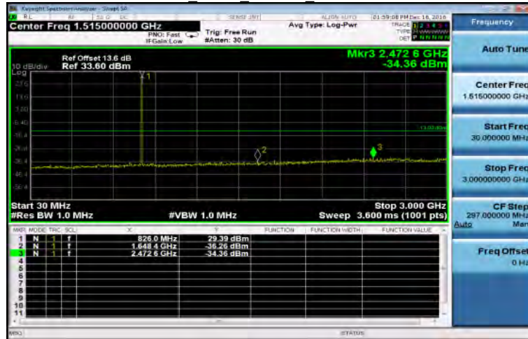
30MHz-3GHz EDGE 850MHz LowCH128-824.2
