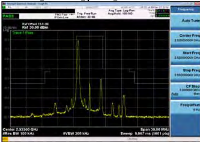
Mask Band7 5MHz QPSK 1 0 MidCH21100-2535
