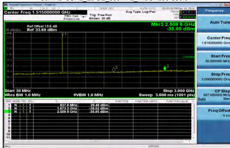
30MHz-3GHz EDGE 850MHz MidCH190-836.6
