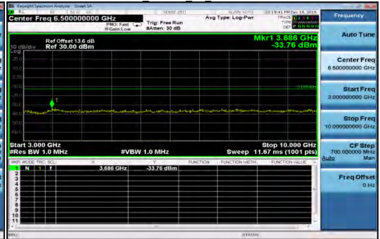
3GHz~10GHz HSUPA B5 MidCH4183-836.6
