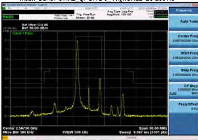
Mask Band7 5MHz QPSK 1 0 HighCH21425-2567.5
