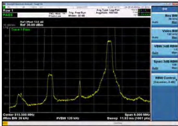
Emission Mask_Band26 for Part 90S_3M_QPSK_MID_RB1,14
