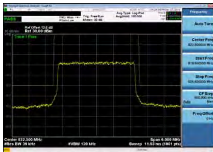
Emission Mask_Band26 for Part 90S_3M_QPSK_HIGH_RB15,0
