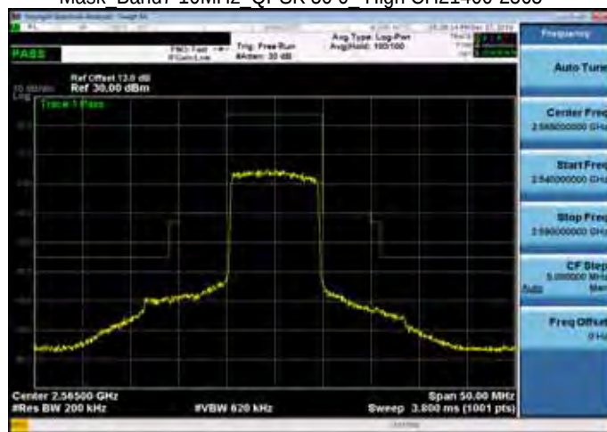
Mask Band7 10MHz QPSK 50 0 High CH21400-2565
