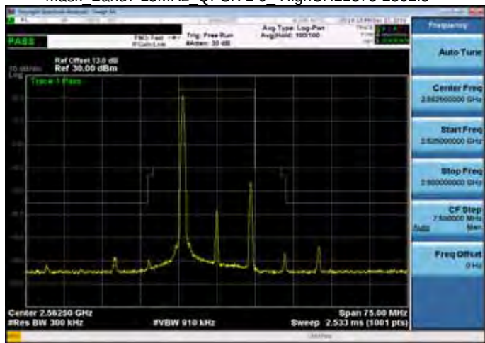
Mask Band7 15MHz_QPSK 1 0_HighCH21375-2562.5
