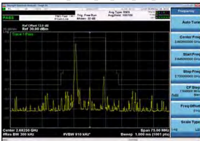
Emission Mask_Band 41_15M_QPSK_HIGH_RB1,0
