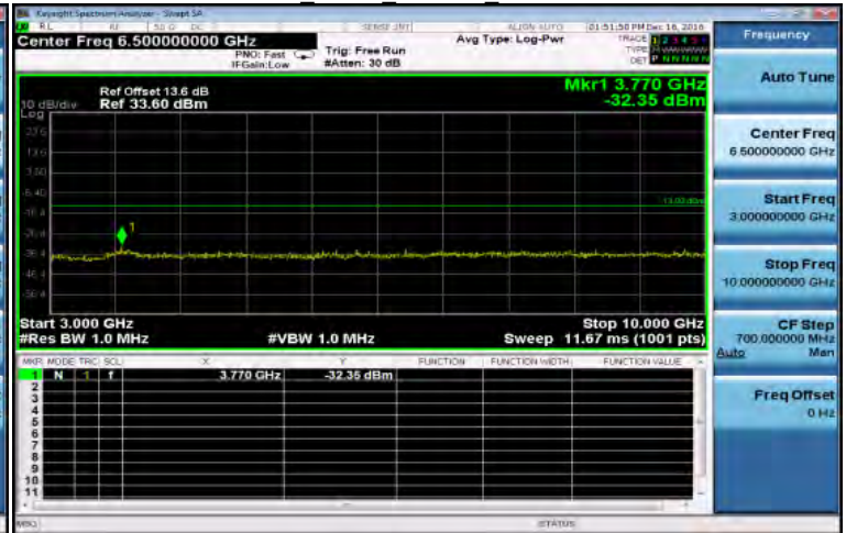
3GHz-10GHz GPRS 850MHz MidCH190-836.6
