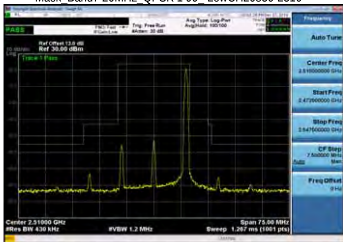
Mask Band7 20MHz_QPSK 1 99 LowCH20850-2510
