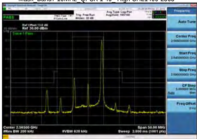
Mask Band7 10MHz QPSK 1 49 High CH21400-2565
