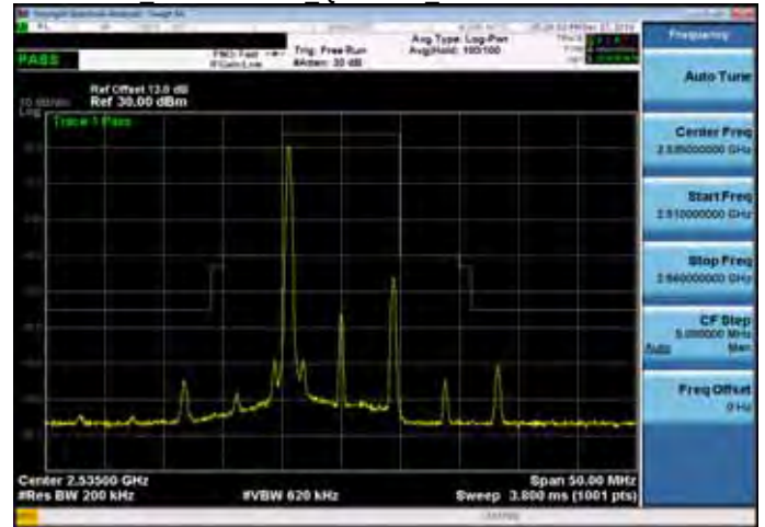
Mask Band7 10MHz QPSK 1 0 MidCH21100-25355
