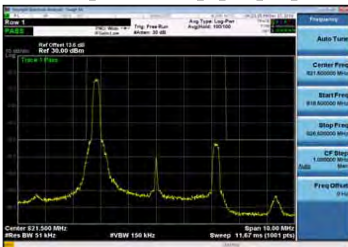
Emission Mask_Band26 for Part 90S_5M_QPSK_HIGH_RB1,0
