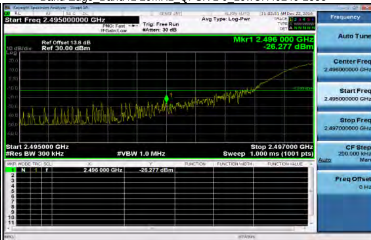
Band Edge Band41 20MHz QPSK 1 0 LowCH40240-2555
