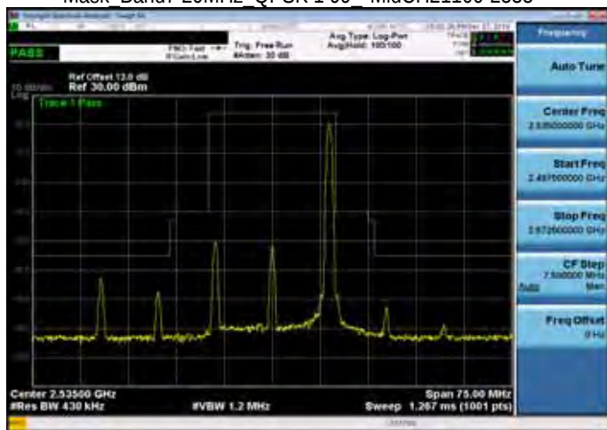
Mask Band7 20MHz_QPSK 1 99 MidCH21100-2535
