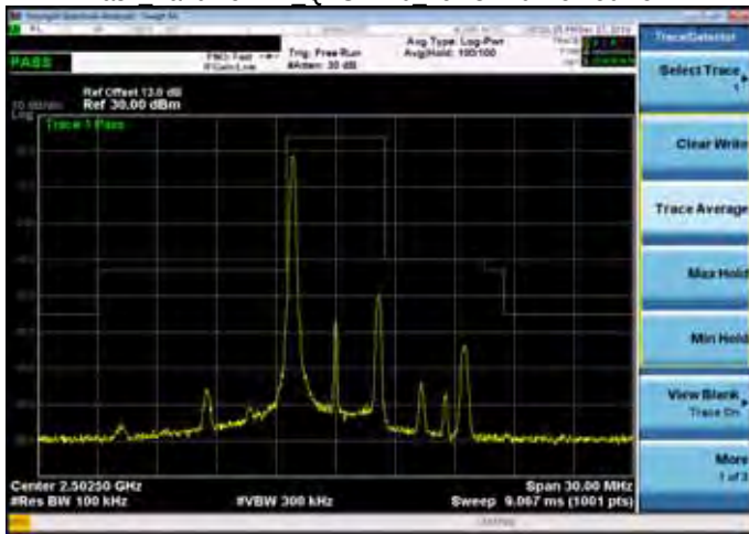
Mask Band7 5MHz QPSK 1 0 LowCH20775-2502.5
