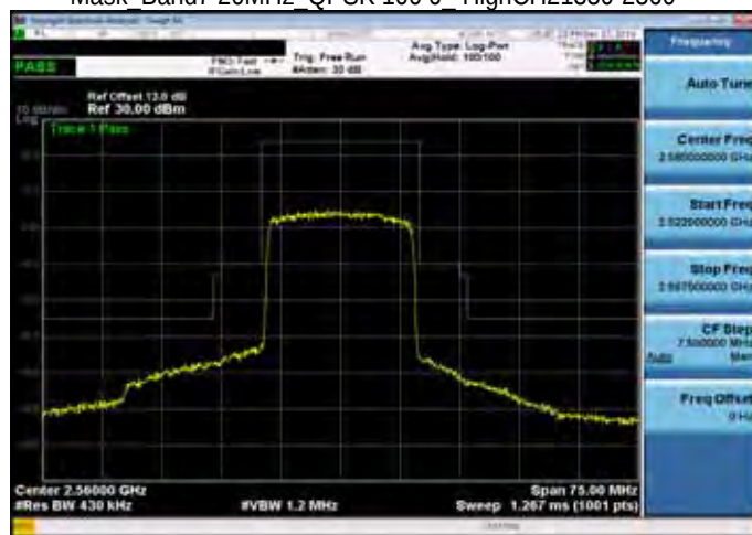
Mask Band7 20MHz_QPSK 100 0 HighCH21350-2560
