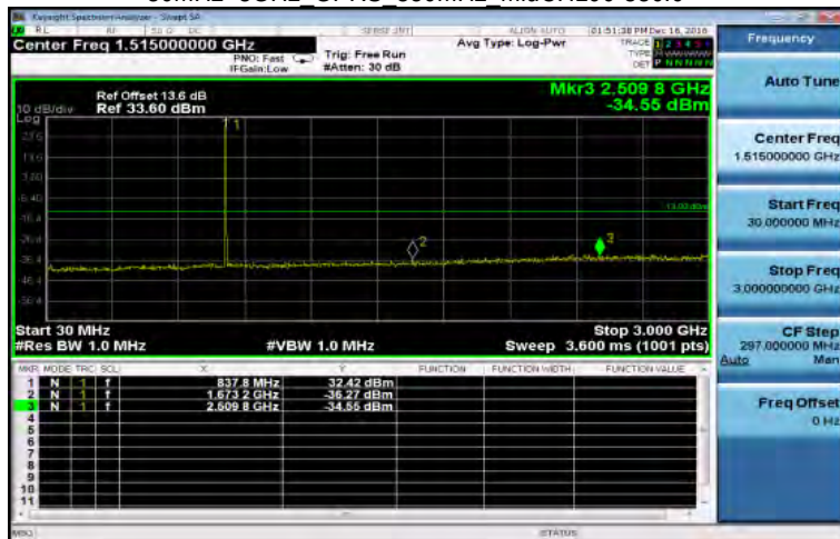
30MHz-3GHz GPRS 850MHz MidCH190-836.6
