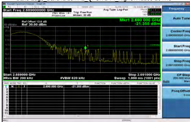
Band Edge Band41 15MHz QPSK 1 74 HighCH41165-2647.5
