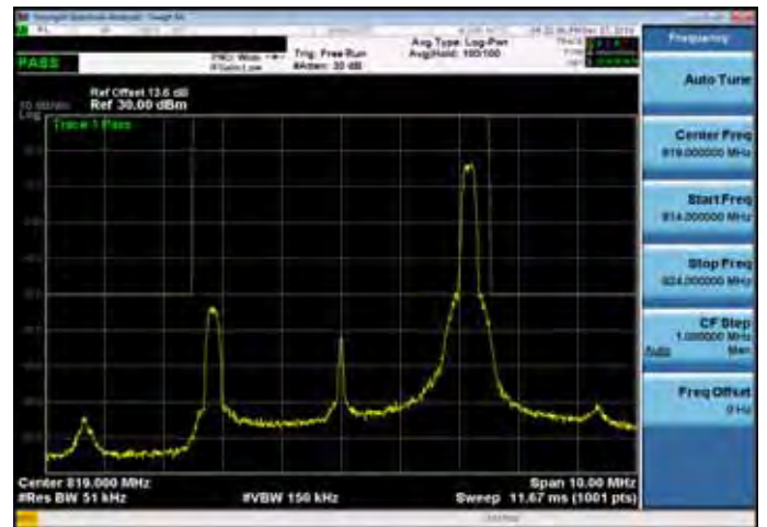
Emission Mask_Band26 for Part 90S_5M_QPSK_HIGH_RB1,24
