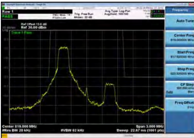
Emission Mask_Band26 for Part 90S_1.4M_QPSK_HIGH_RB1,0
