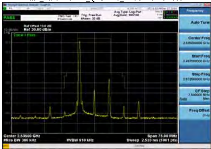
Mask Band7 15MHz_QPSK 1 0_MidCH20175-2535
