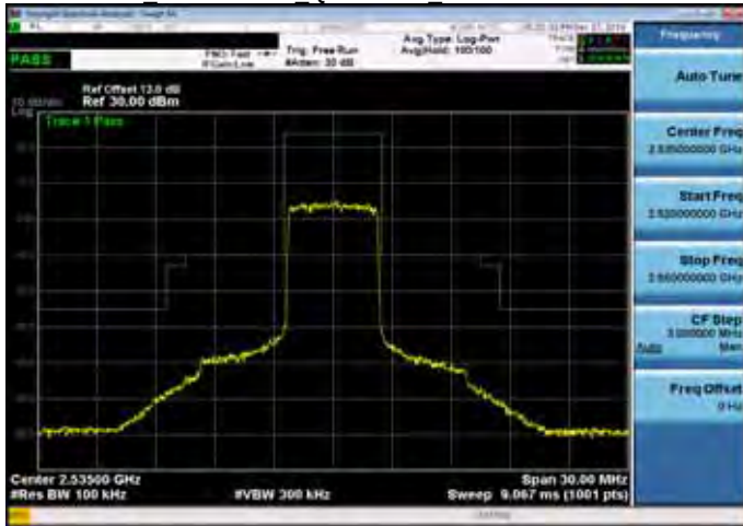
Mask Band7 5MHz QPSK 25 0 MidCH21100-2535
