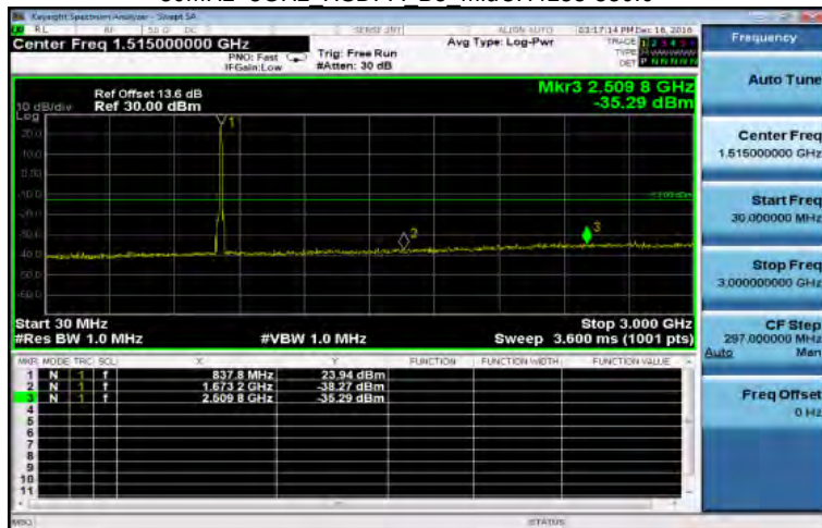
30MHz~3GHz HSDPA B5 MidCH4183-836.6
