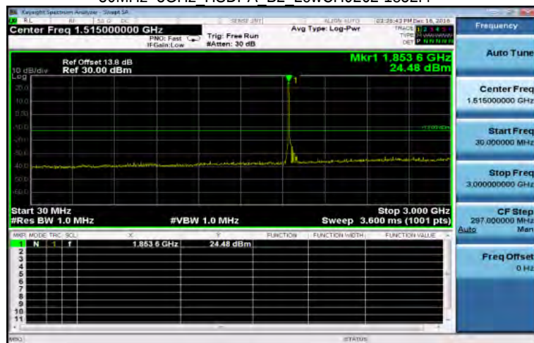
30MHz~3GHz HSDPA B2 LowCH9262-1852.4
