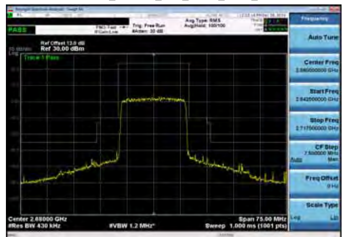
Emission Mask_Band 41_20M_QPSK_HIGH_RB100,0
