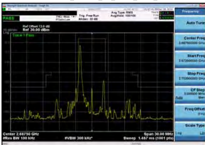
Emission Mask_Band 41_5M_QPSK_HIGH_RB1,0
