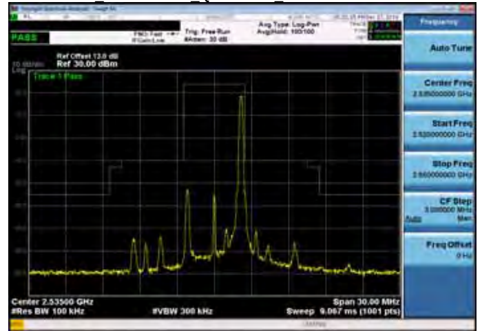
Mask Band7 5MHz QPSK 1 24 MidCH21100-2535
