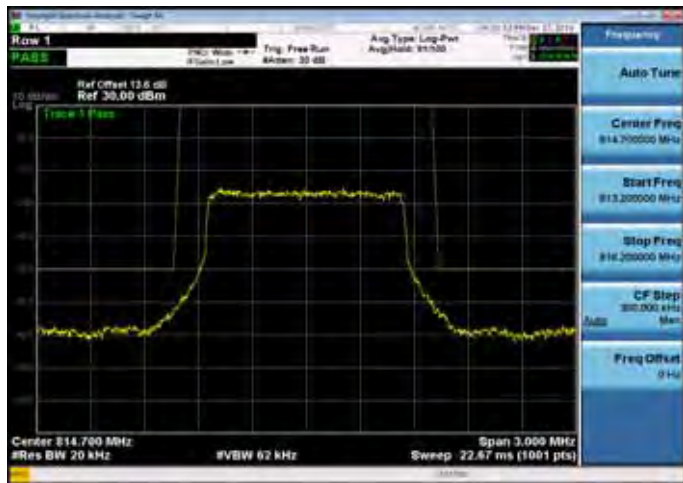
Emission Mask_Band26 for Part 90S_1.4M_QPSK_MID_RB6,0
