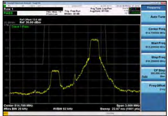
Emission Mask_Band26 for Part 90S_1.4M_QPSK_MID_RB1,5
