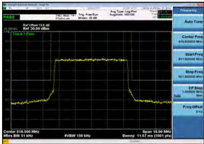
Emission Mask_Band26 for Part 90S_5M_QPSK_MID_RB25,0
