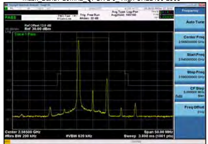
Mask Band7 10MHz QPSK 1 0 High CH21400-2565
