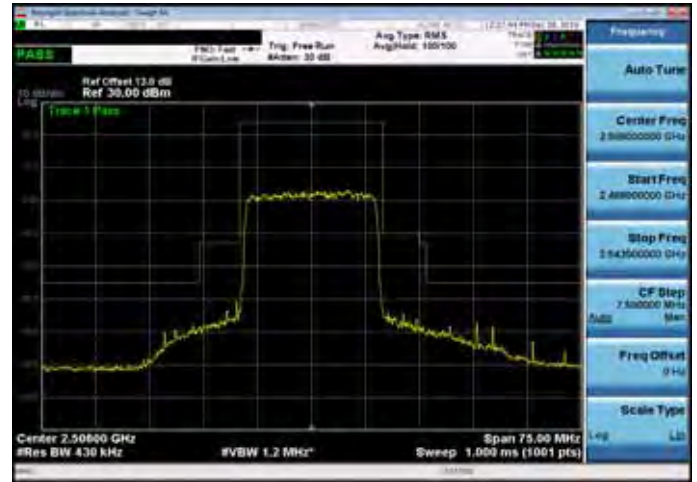
Emission Mask_Band 41_20M_QPSK_MID_RB100,0
