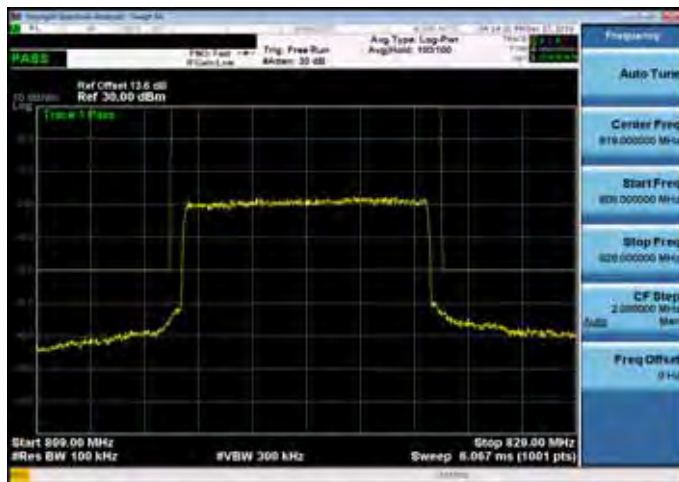
Emission Mask_Band26 for Part 90S_10M_QPSK_MID_RB50,0
