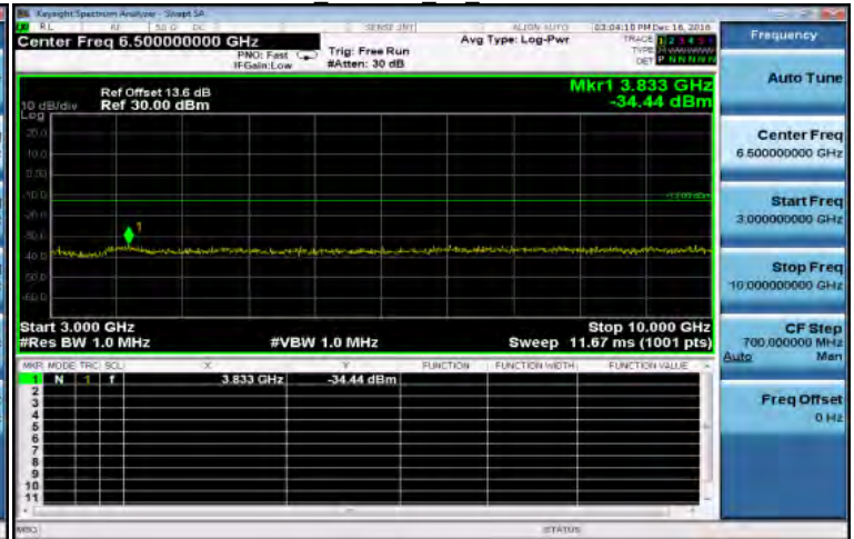
3GHz~10GHz WCDMA B5 MidCH4183-836.6
