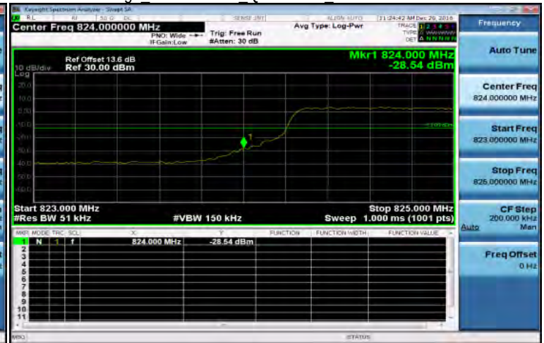
Band Edge Band5 5MHz QPSK 25 0 LowCH20425-826.5
