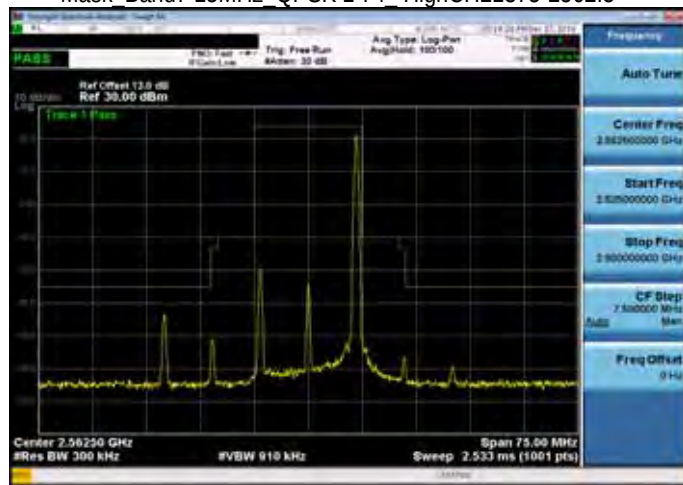
Mask Band7 15MHz_QPSK 1 74_HighCH21375-2562.5
