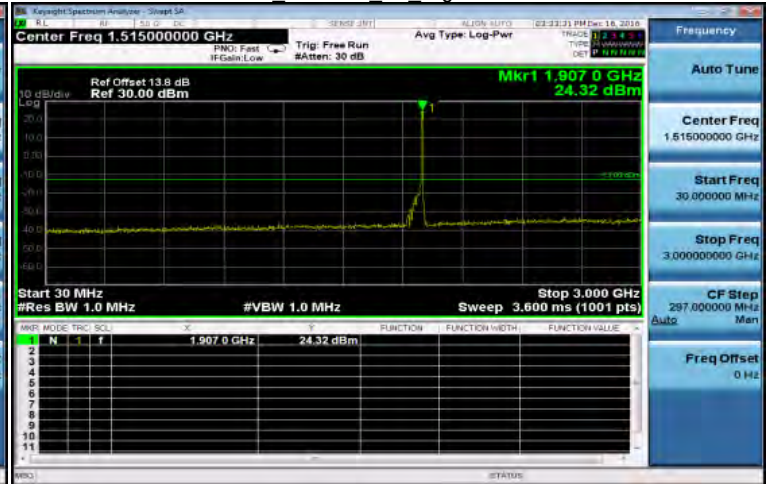
30MHz~3GHz WCDMA B2 HighCH9538-1907.6
