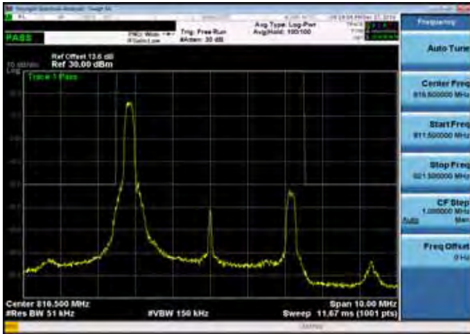
Emission Mask_Band26 for Part 90S_5M_QPSK_MID_RB1,0
