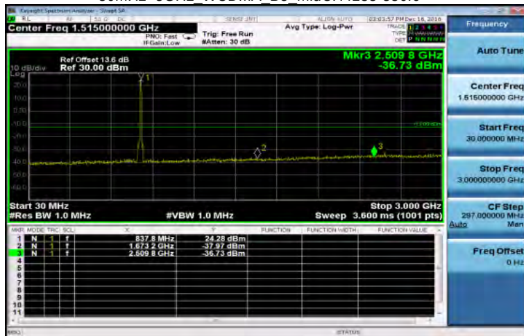
30MHz~3GHz WCDMA B5 MidCH4183-836.6
