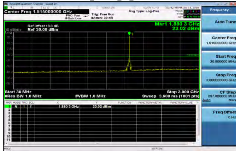
30MHz~3GHz HSUPA B2 MidCH9400-1880
