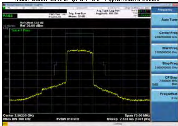
Mask Band7 15MHz_QPSK 75 0_HighCH21375-2562.5
