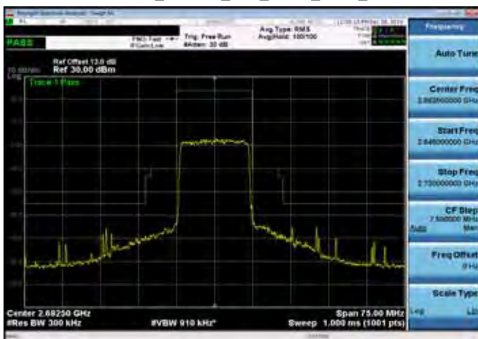
Emission Mask_Band 41_15M_QPSK_HIGH_RB75,0
