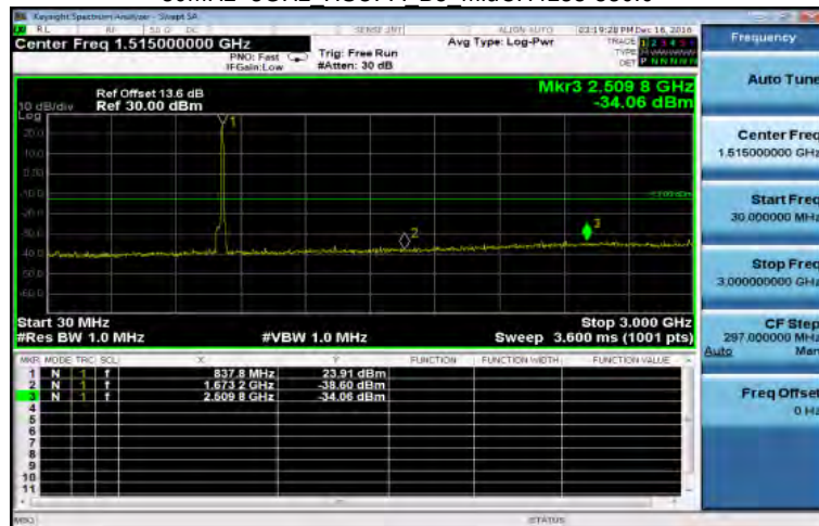
30MHz~3GHz HSUPA B5 MidCH4183-836.6
