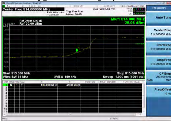
Band Edge Band 26 for Part 90S 5M-QPSK-25 0-LOW
