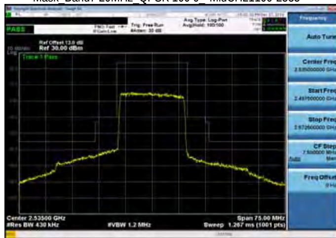
Mask Band7 20MHz_QPSK 100 0 MidCH21100-2535
