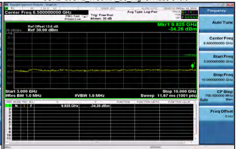
3GHz~10GHz WCDMA B5 HighCH4233-846.6
