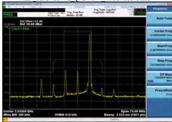
Mask Band7 15MHz_QPSK 1 74_MidCH20175-2535
