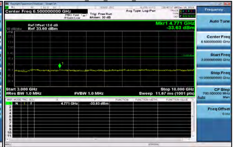
3GHz~10GHz GSM 850MHz MidCH190-836.6
