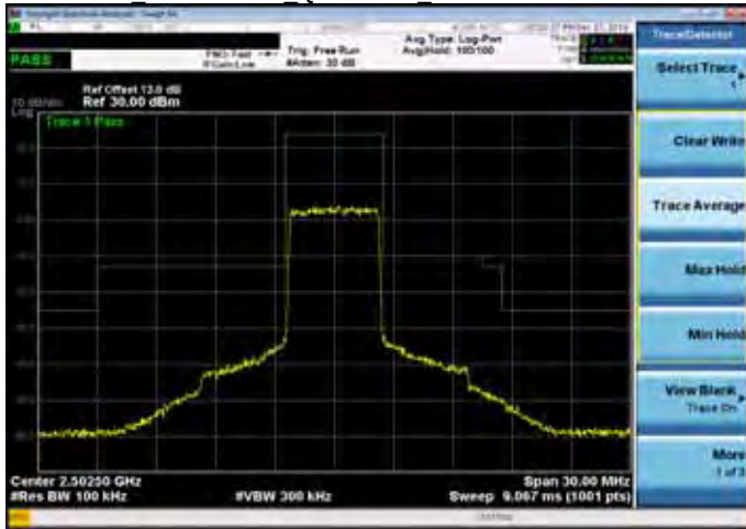
Mask Band7 5MHz QPSK 25 0 LowCH20775-2502.5
