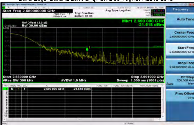
Band Edge Band41 20MHz QPSK 1 99 HighCH41140-2645
