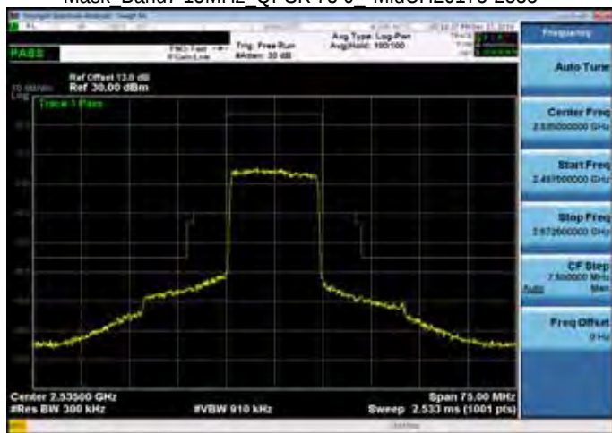
Mask Band7 15MHz_QPSK 75 0_MidCH20175-2535
