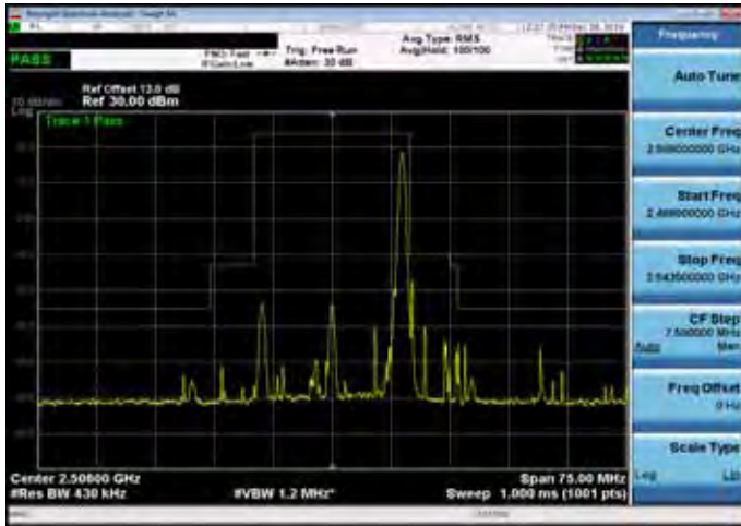
Emission Mask_Band 41_20M_QPSK_MID_RB1,99
