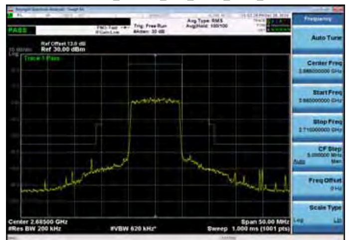
Emission Mask_Band 41_10M_QPSK_HIGH_RB50,0
