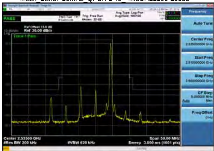
Mask Band7 10MHz QPSK 1 49 MidCH21100-25355
