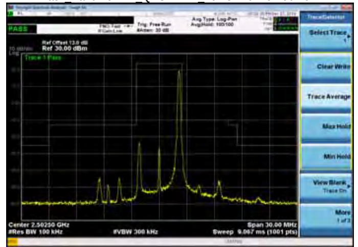
Mask Band7 5MHz QPSK 1 24 LowCH20775-2502.5
