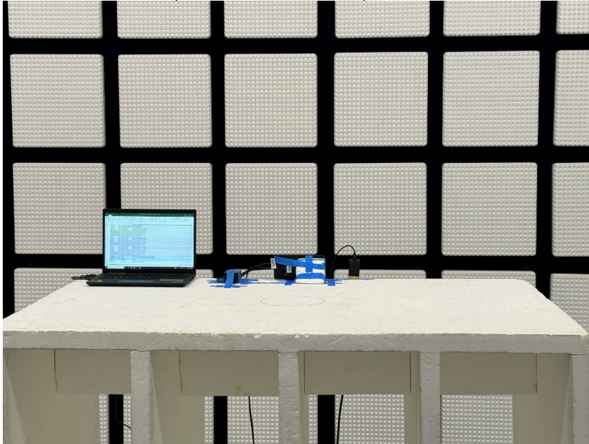
RADIATED PHOTO (>1GHz BLE/BT C0/C1)
