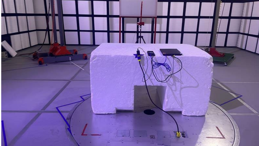
RADIATED PHOTO (<30 MHz 6 GHz WLAN MIMO)
