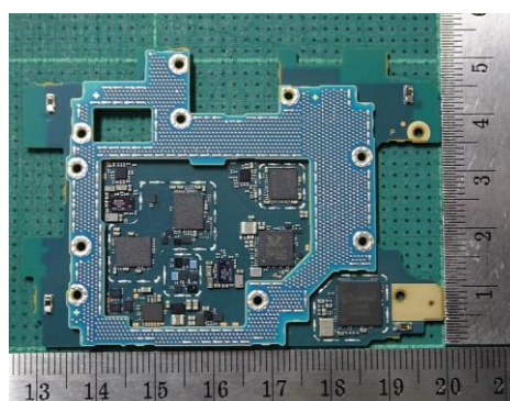
Only ②Rear PBA without Shield case (Front-side)
