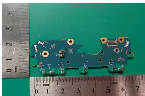
Internal Ant_Sub-PBA (Front-side)
