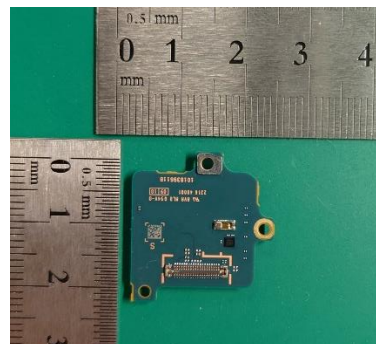
Internal Back-PBA (Rear-side)
