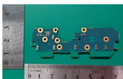
Internal Ant_Sub-PBA (Rear-side)
