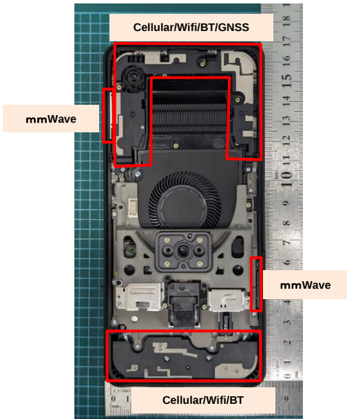
Without Rear panel --Antenna: in red frame
