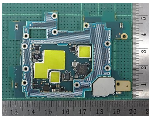
Only ②Rear PBA with Shield case (Front-side)
