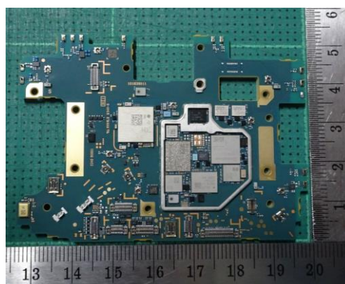
Combined ①Front PBA and ②Rear PBA without Shield case (Rear-side)
