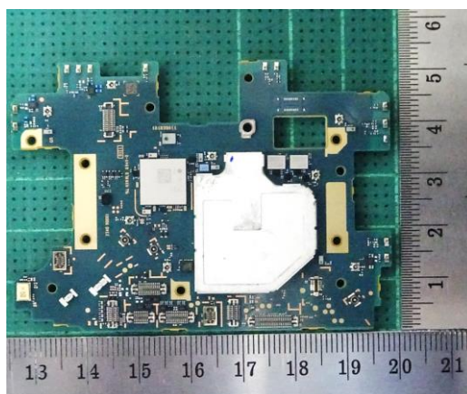
Combined ①Front PBA and ②Rear PBA with Shield case (Rear-side)
