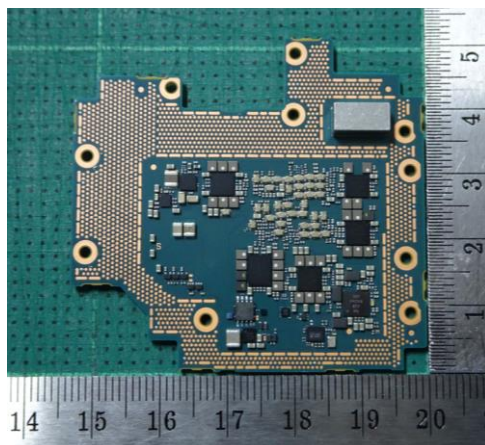
Only ①Front PBA (Rear-side)
