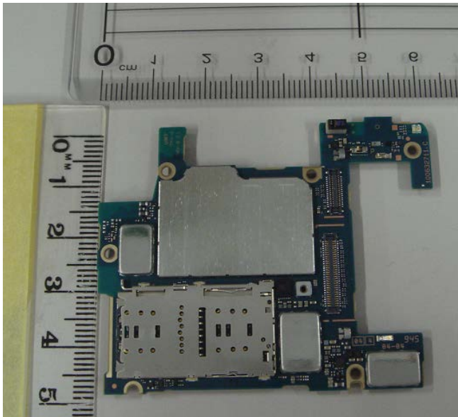
Internal PWB with Shield cases (Front-side)
