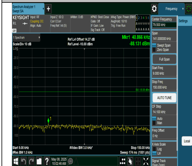
Band41-20MHz-QPSK-41490-1RB#0-0.009~0.15-PASS
