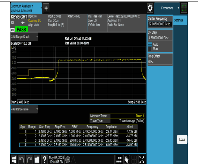
Band41-20MHz-QPSK-39750-100RB#0-PASS
