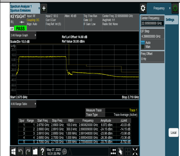
Band41-15MHz-QPSK-41515-75RB#0-PASS
