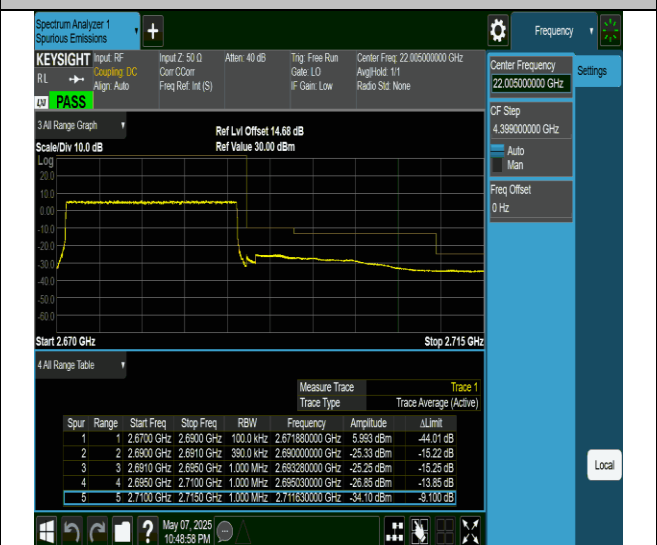
Band41-20MHz-QPSK-41490-100RB#0-PASS
