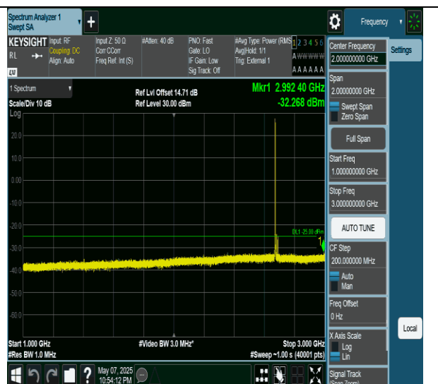
Band41-20MHz-QPSK-41490-1RB#0-1000~3000-PASS
