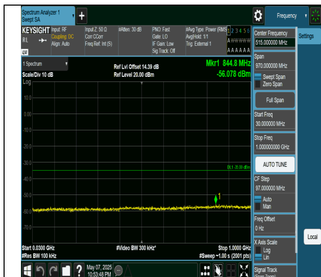
Band41-20MHz-QPSK-41490-1RB#0-30~1000-PASS
