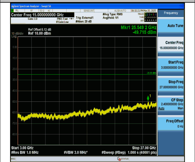
Band41-20MHz-QPSK-40620-1RB#0-3000~27000-PASS
