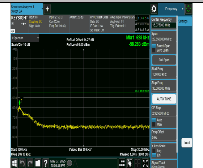
Band41-20MHz-QPSK-41490-1RB#0-0.15~30-PASS
