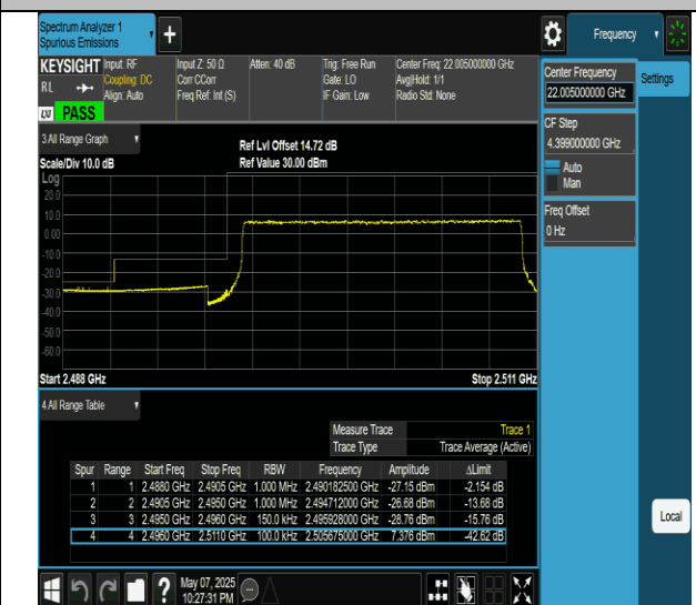
Band41-15MHz-QPSK-39725-75RB#0-PASS
