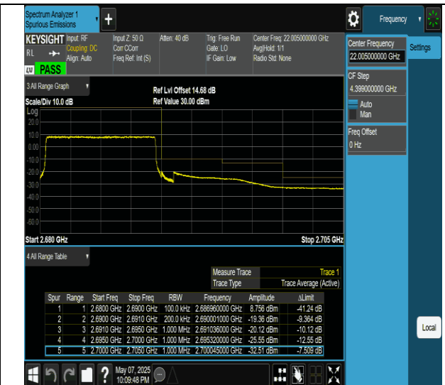
Band41-10MHz-QPSK-41540-50RB#0-PASS
