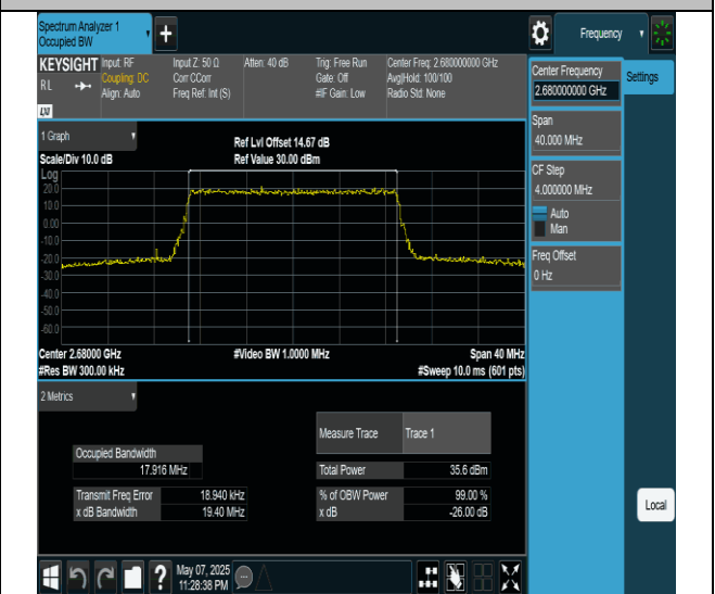
Band41-20MHz-64QAM-41490-100RB#0-PASS
