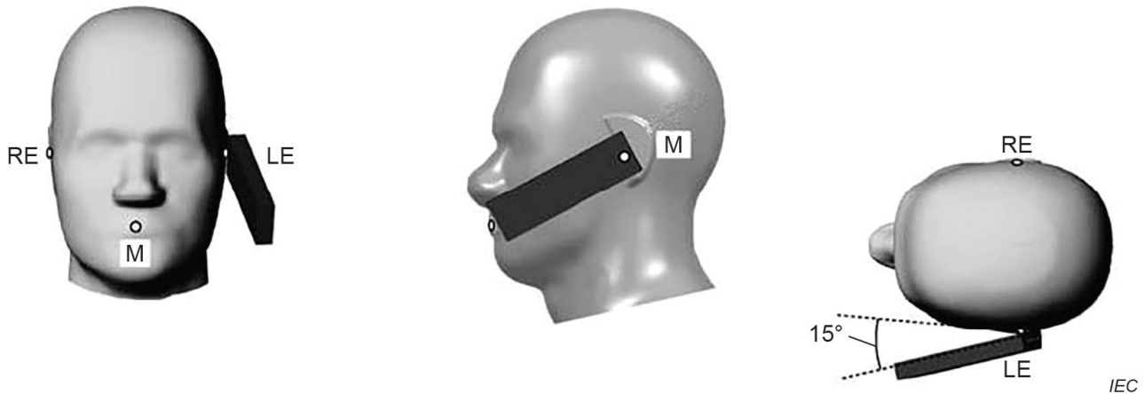
Figure 11-5: Front, Side and Top View of Tilt 15^\circ Position
