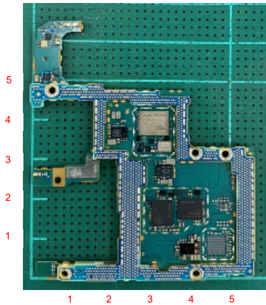
Internal Main-PWB Rear without Shield case (Front-side)
