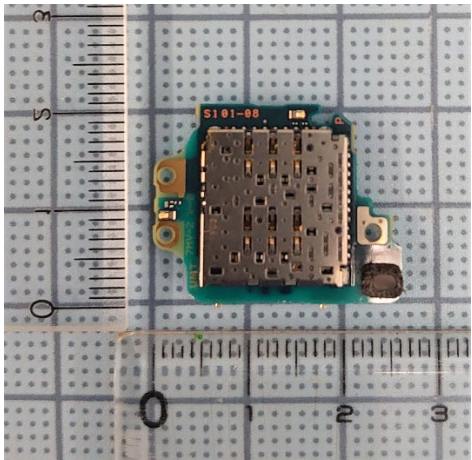
Internal Sub-PWB (Front-side)
