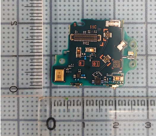
Internal Sub-PBA (Rear-side)
