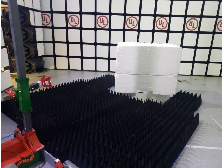
RADIATED PHOTO (>1GHz BT/BLE/2.4 WLAN)
