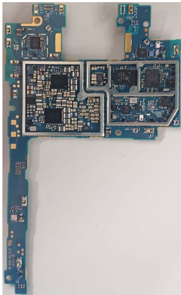
Internal PWB without Shield cases (Rear-side)
