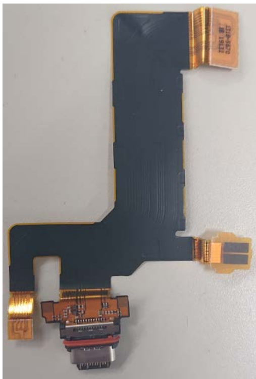
Relay FPC (Front-side)
