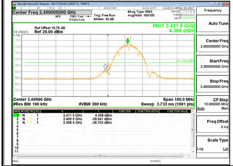
2.4GHz 2TX CBE CH1 (Chain 0)
