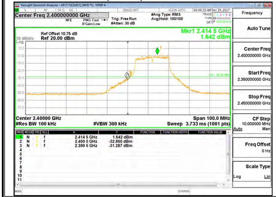
2.4GHz 2TX CBE CH1 (Chain 1)
