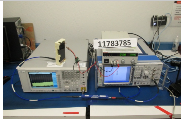
ANTENNA PORT CONDUCTED PHOTO
