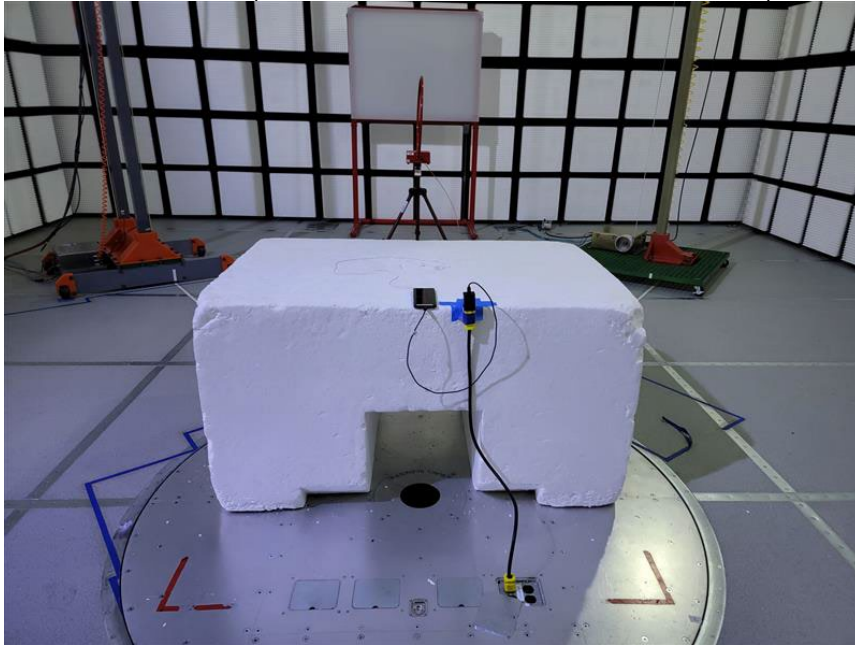
RADIATED PHOTO (<30 MHz BLE/BT C0/C1, 2.4 WLAN MIMO)
