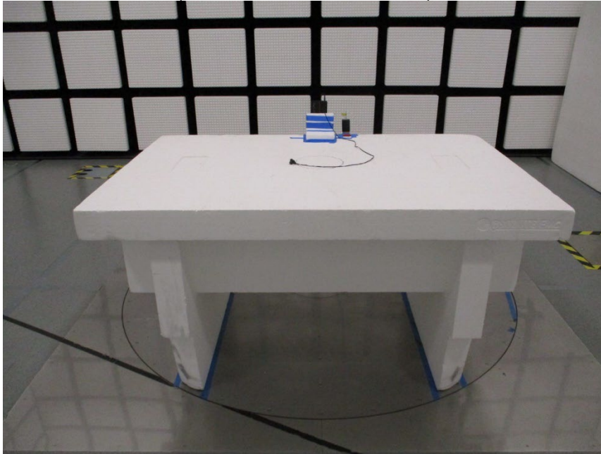
RADIATED PHOTO (30-1000 MHz 5 WLAN MIMO)
