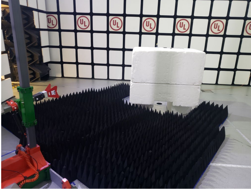
RADIATED PHOTO (>1GHz BLE/BT C0/C1, 2.4 WLAN MIMO)
