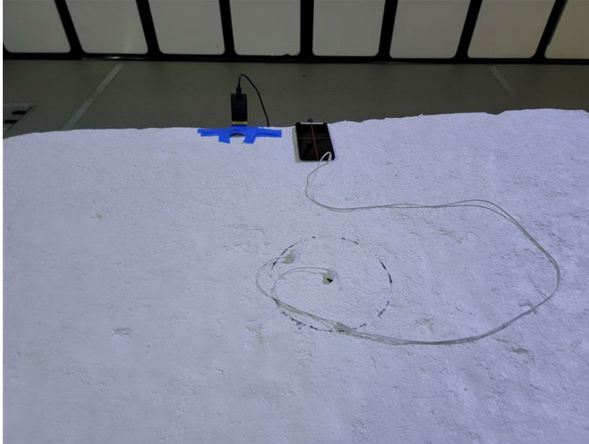
RADIATED PHOTO (30-1000 MHz BLE/BT C0/C1, 2.4 WLAN MIMO)
