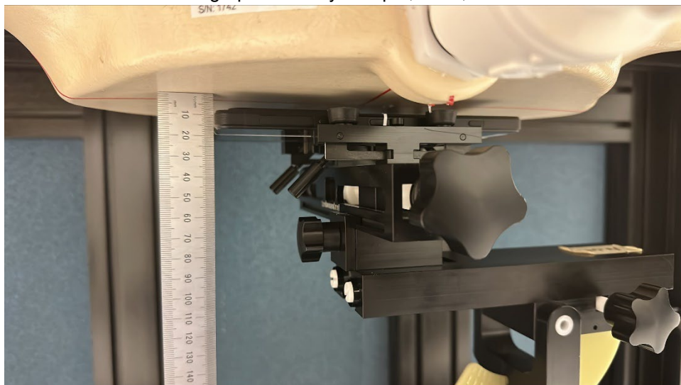
Photograph 10: Body/Hotspot, Back, 10 mm
