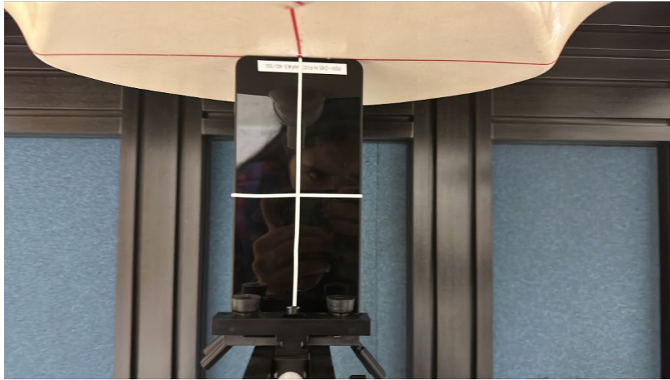
Photograph 19: Extremity, Edge Bottom, 0 mm
