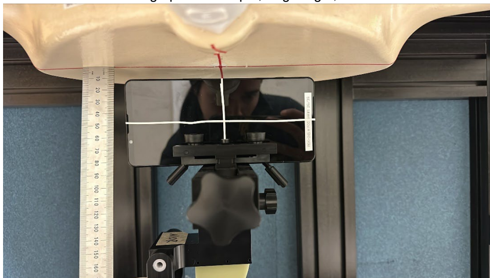
Photograph 14: Hotspot, Edge Right, 10 mm
