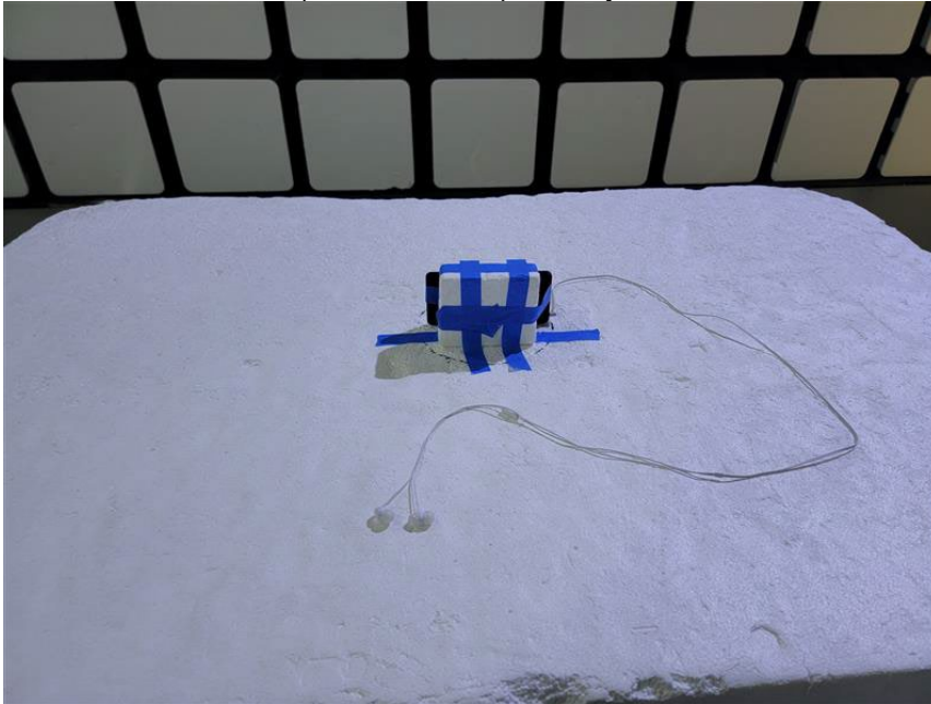
RADIATED PHOTO (30-1000 MHz) Battery
