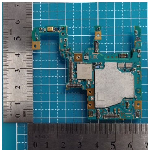
Combined ①Front PBA and ②Rear PBA with Shield case (Rear-side)
