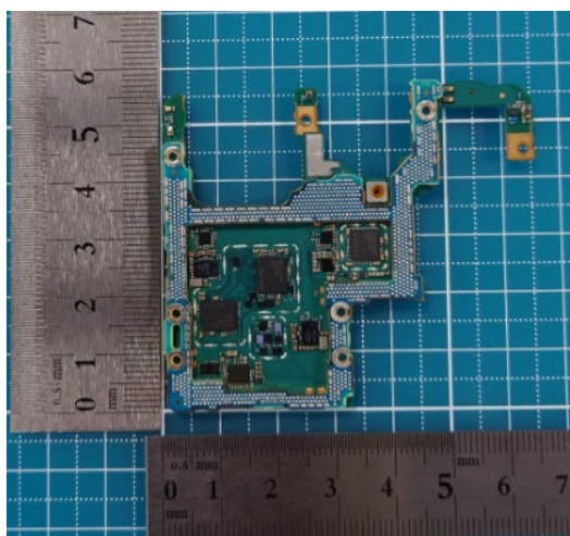
Only ②Rear PBA without Shield case (Front-side)
