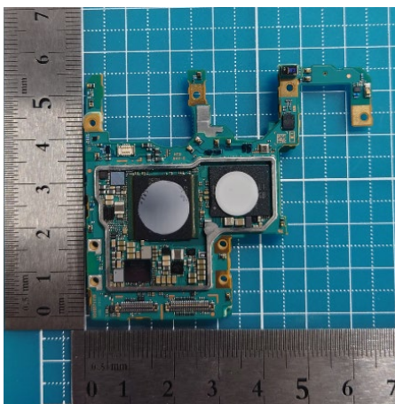
Combined ①Front PBA and ②Rear PBA without Shield cases (Front-side)
