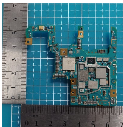
Combined ①Front PBA and ②Rear PBA without Shield case (Rear-side)
