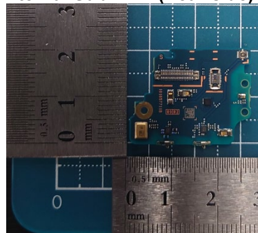
Internal Sub-PBA (Rear-side)
