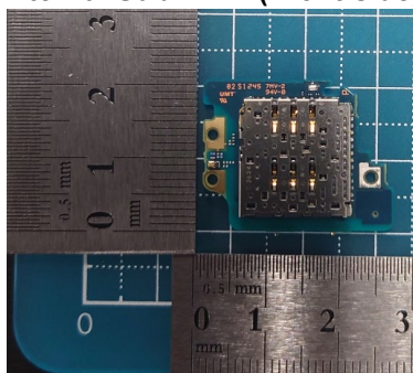
Internal Sub-PWB (Front-side)
