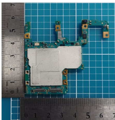
Combined ①Front PBA and ②Rear PBA with Shield cases (Front-side)
