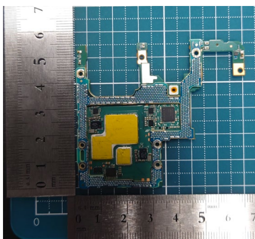
Only ②Rear PBA with Shield case (Front-side)
