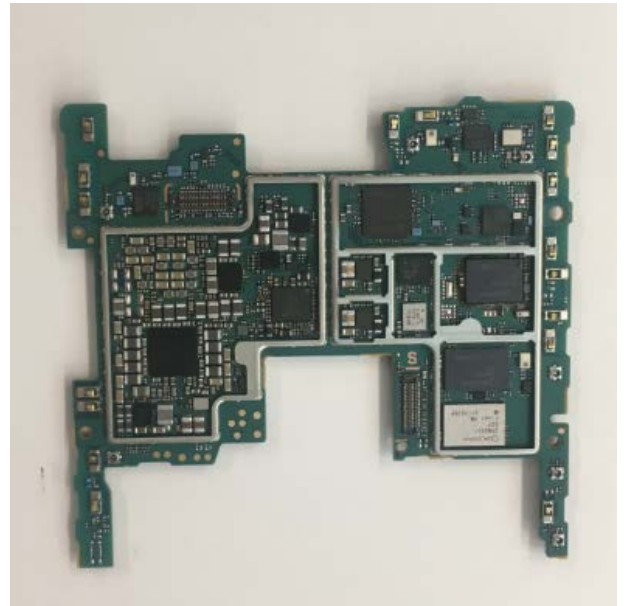
Internal PWB without Shield cases (Rear-side)
