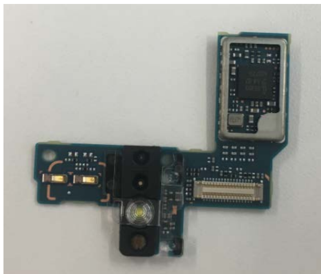
Internal Sub-PWB without Shield cases (Front-side)
