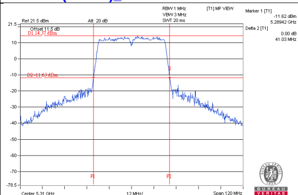
802.11ac (VHT40)_Chain 0 / CH62
