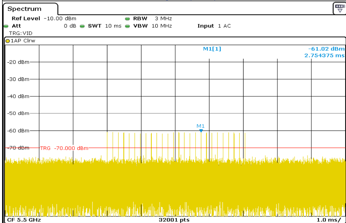
Radar Signal 2
