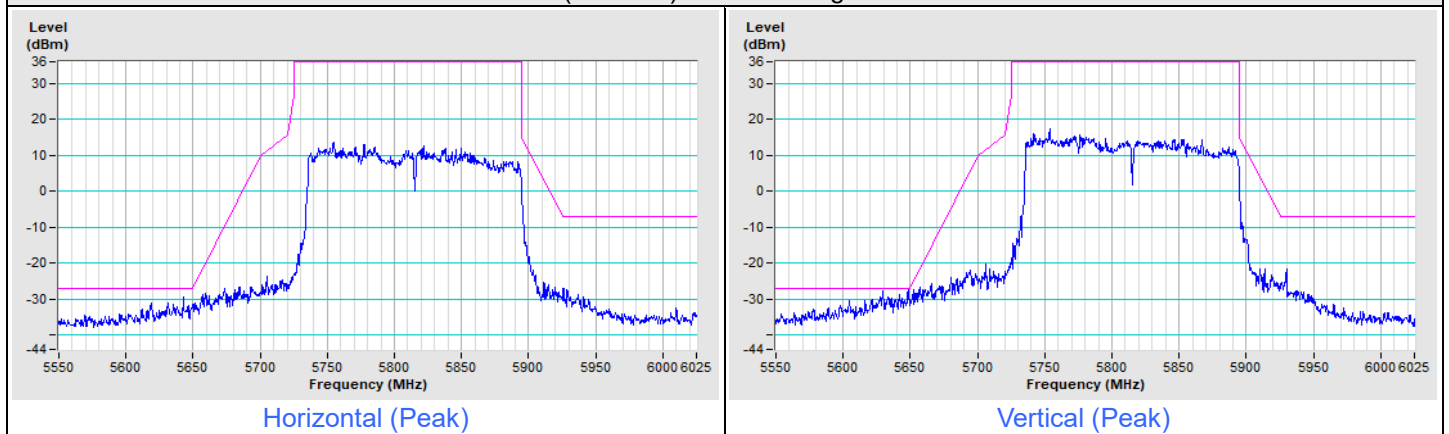
802.11be (EHT160) Beamforming Channel 163
