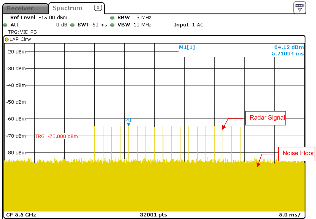
Radar Signal 0
