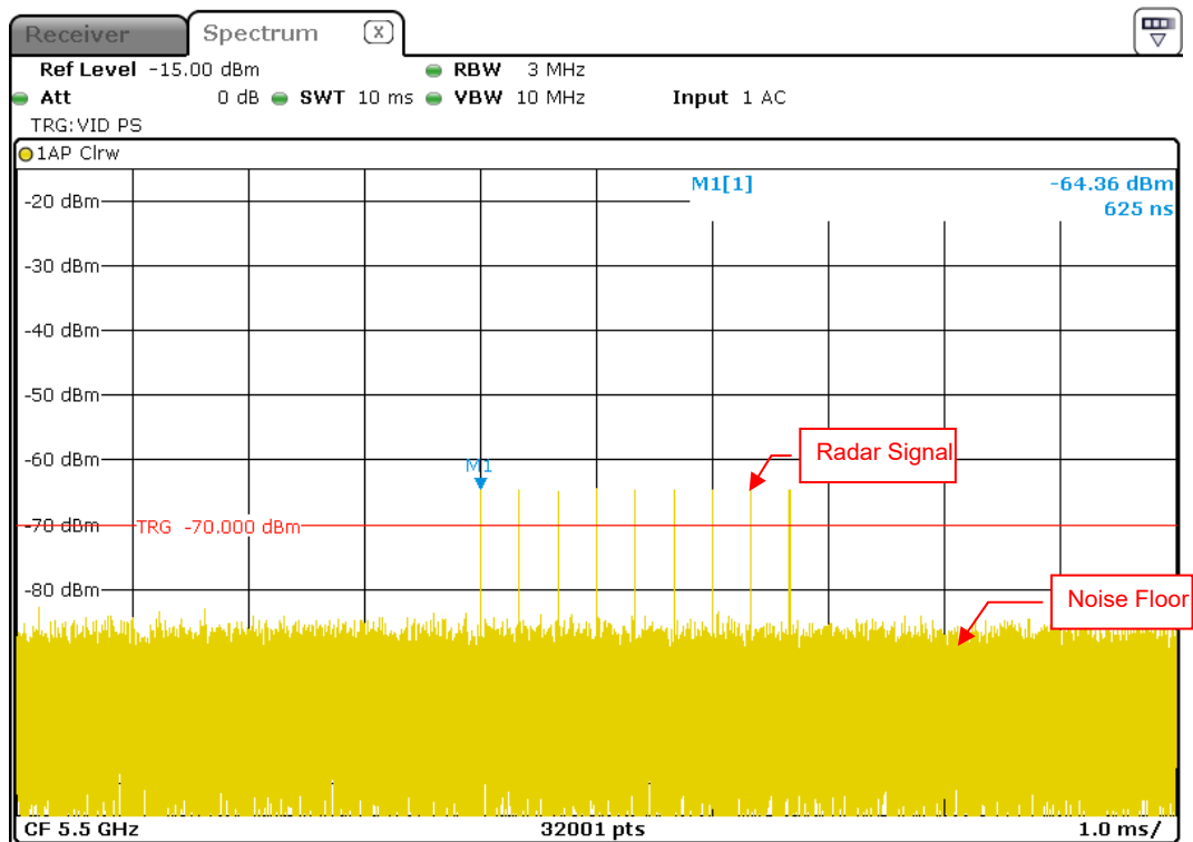
Radar Signal 6
