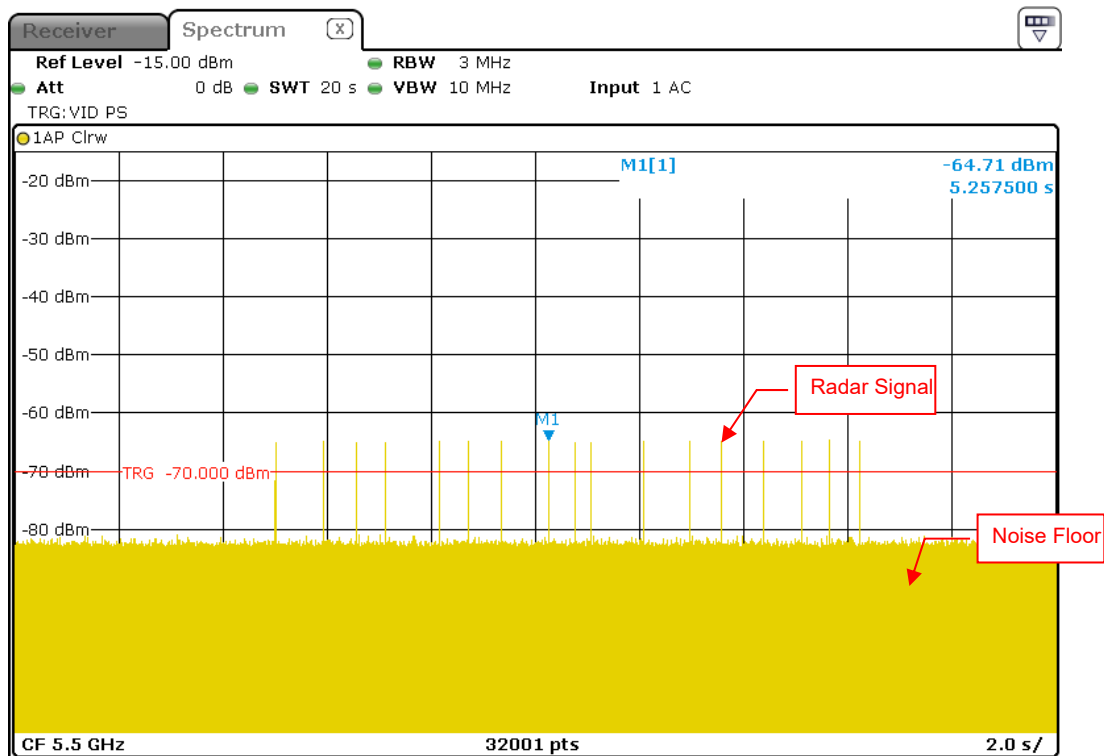
Radar Signal 5
