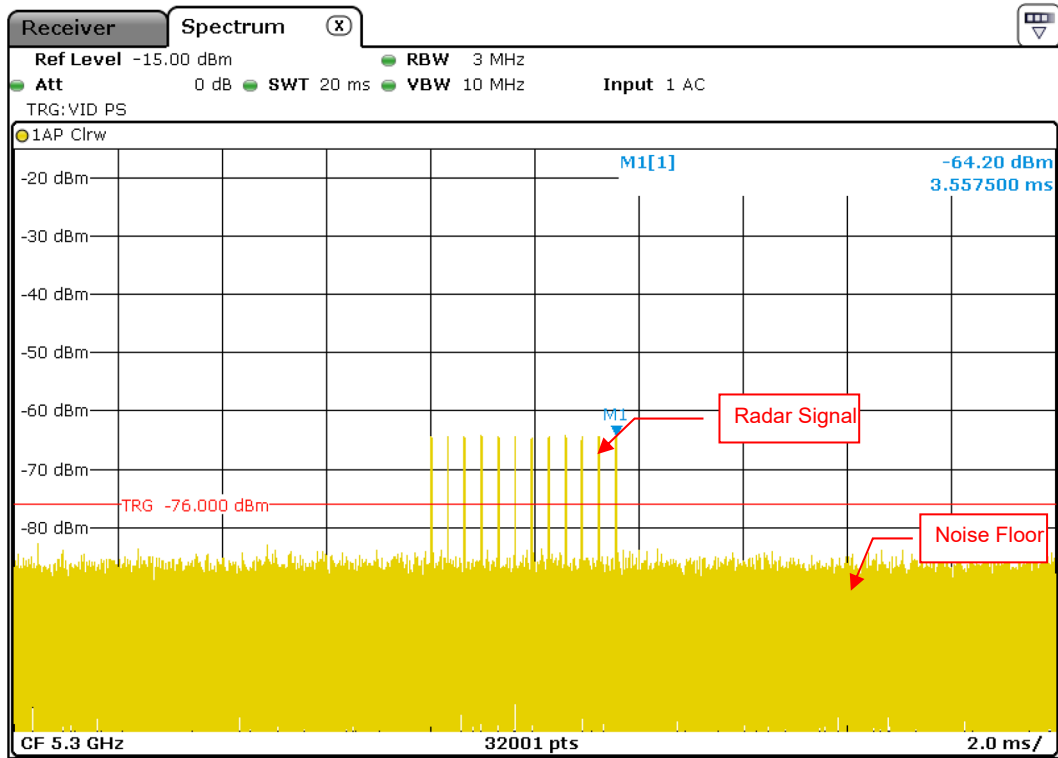
Radar Signal 4
