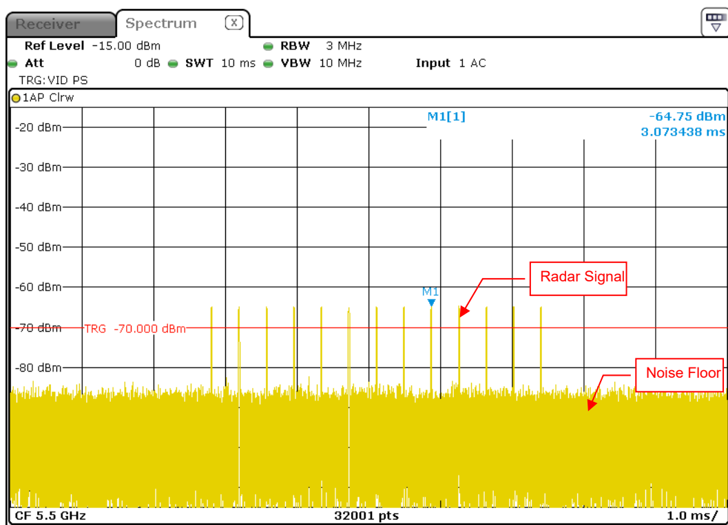
Radar Signal 4
