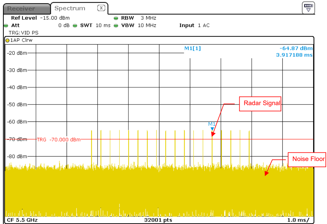
Radar Signal 3
