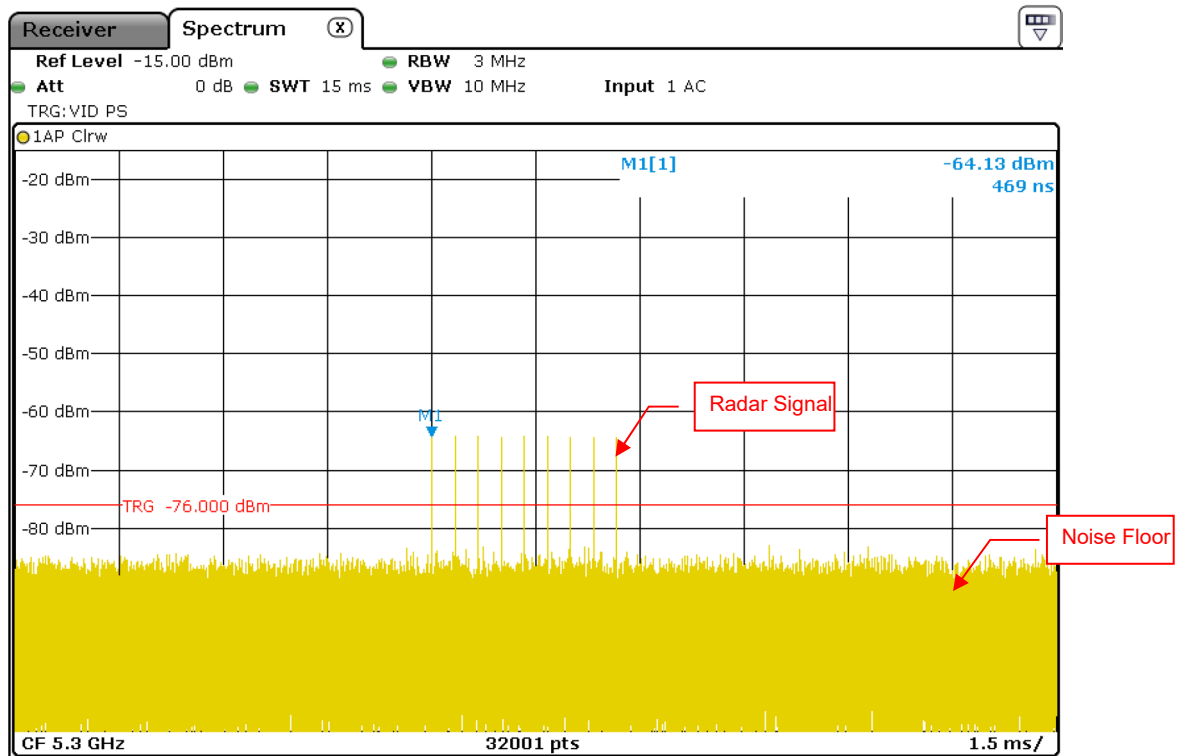
Radar Signal 6
