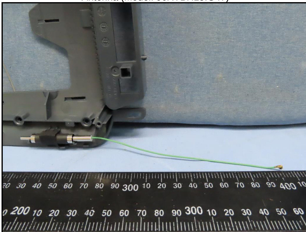
Antenna (Model: 90XYBH15.G47)
