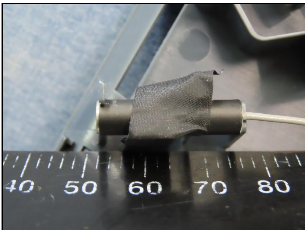
Antenna (Model: 90XYBH15.G54)
