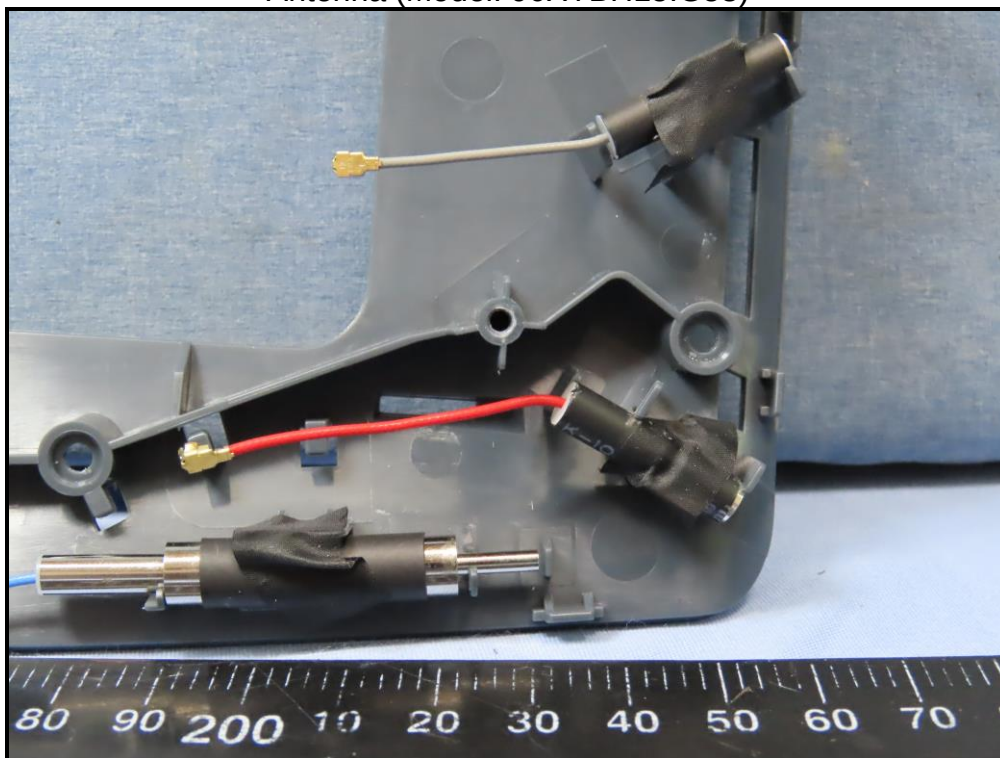
Antenna (Model: 90XYBH15.G53)
