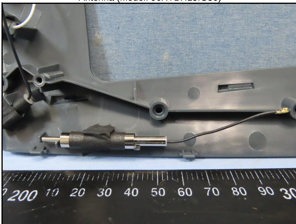
Antenna (Model: 90XYBH15.G50)
