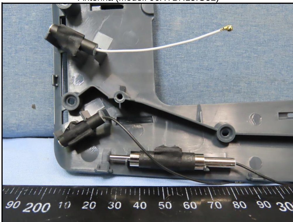
Antenna (Model: 90XYBH15.G52)
