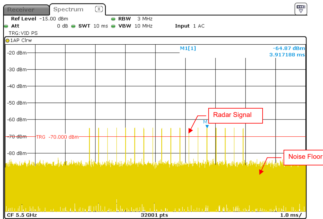
Radar Signal 3
