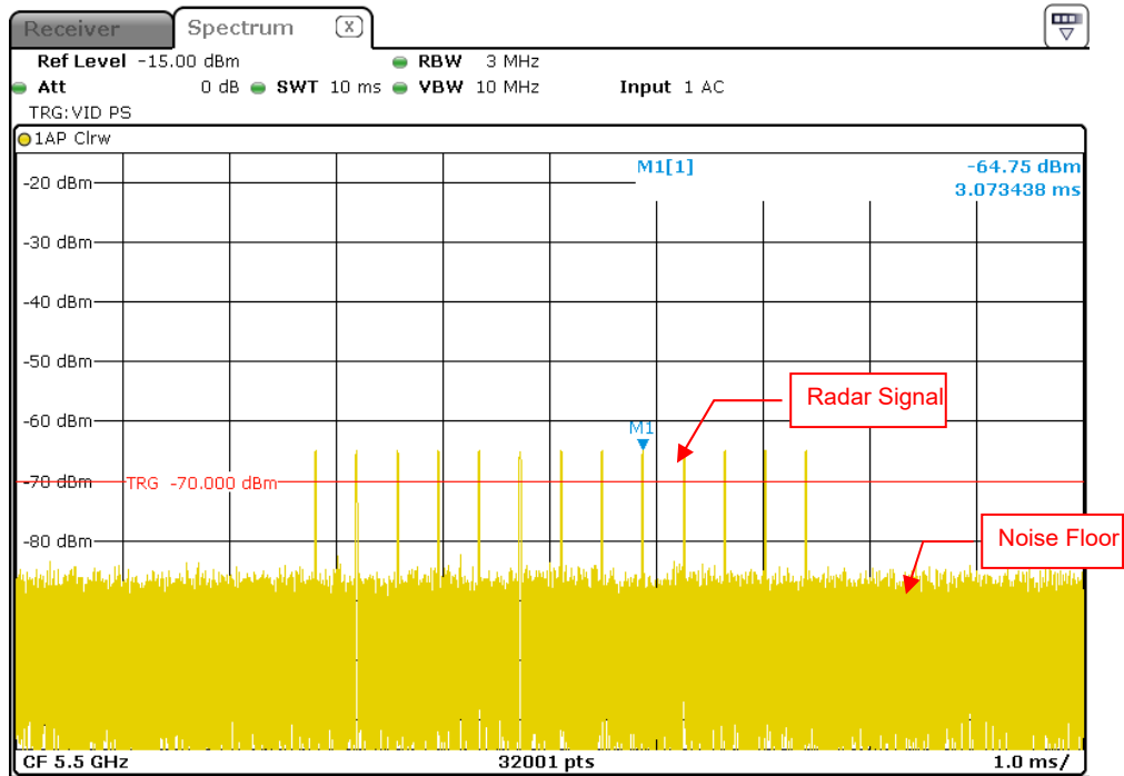
Radar Signal 4
