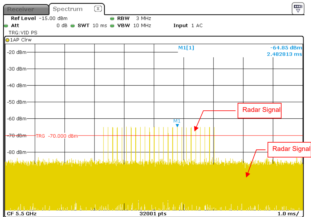
Radar Signal 2
