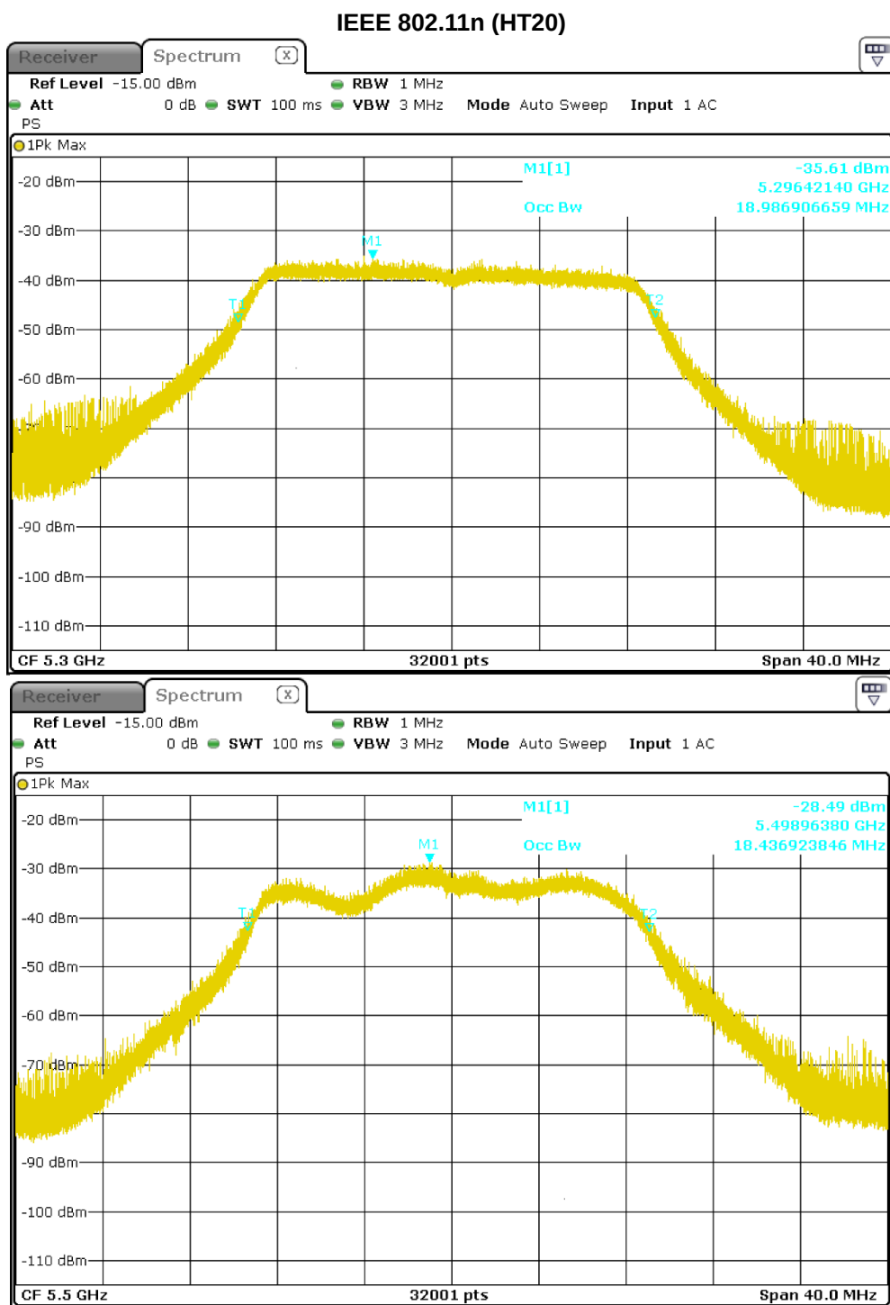
U-NII 99% Channel bandwidth
