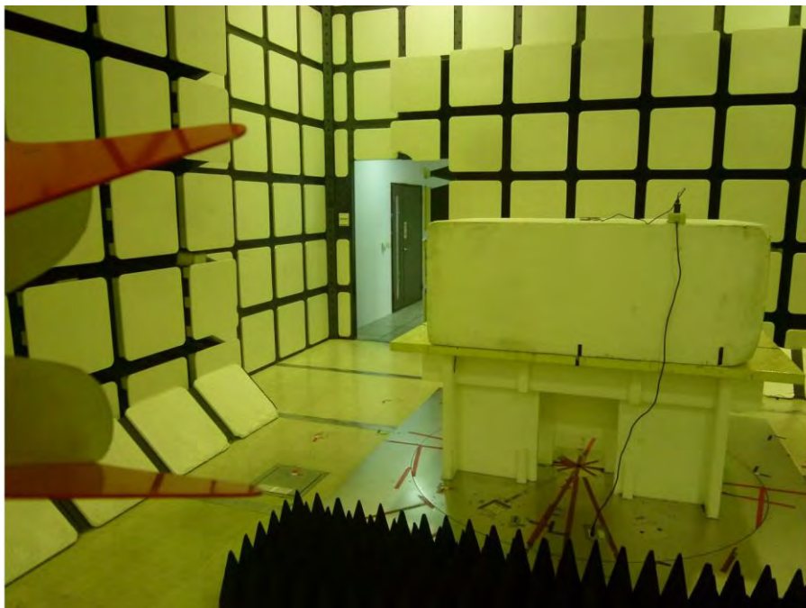
Above 1 GHz _ Rear View (AC Adapter : 2ACS005B)
