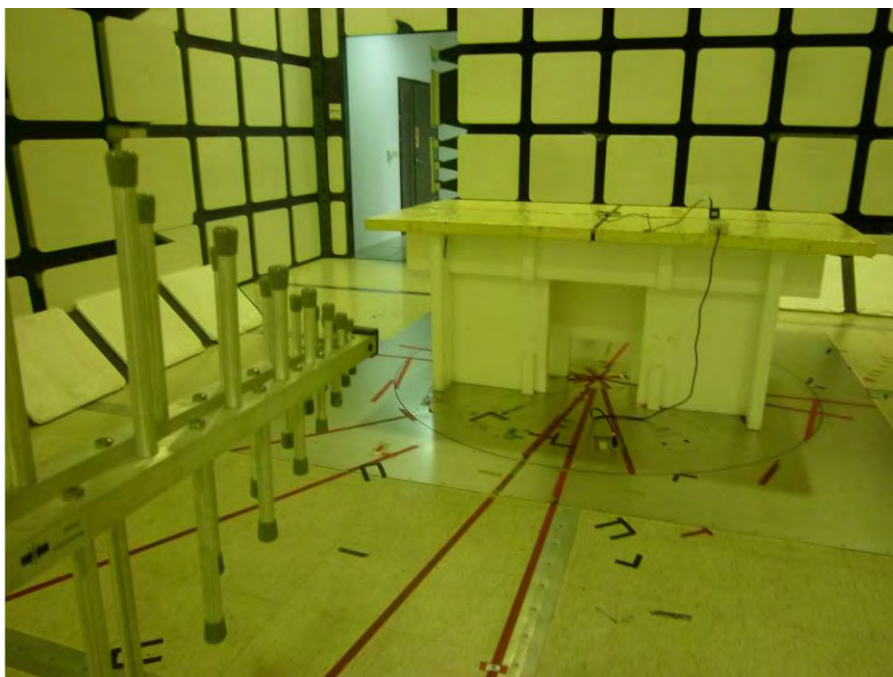
Below 1 GHz _ Rear View (AC Adapter : AD2083329)
