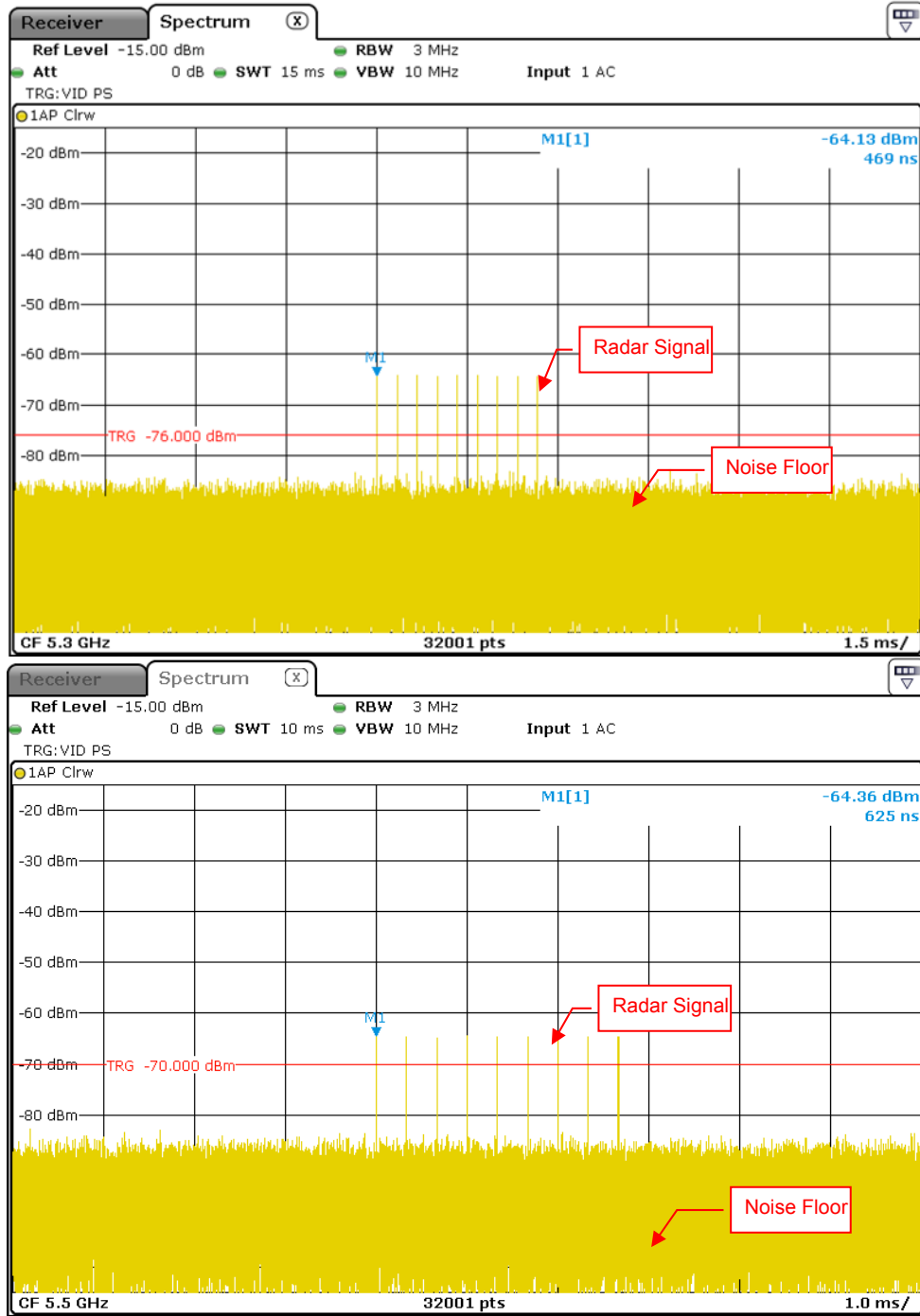
Radar Signal 6
