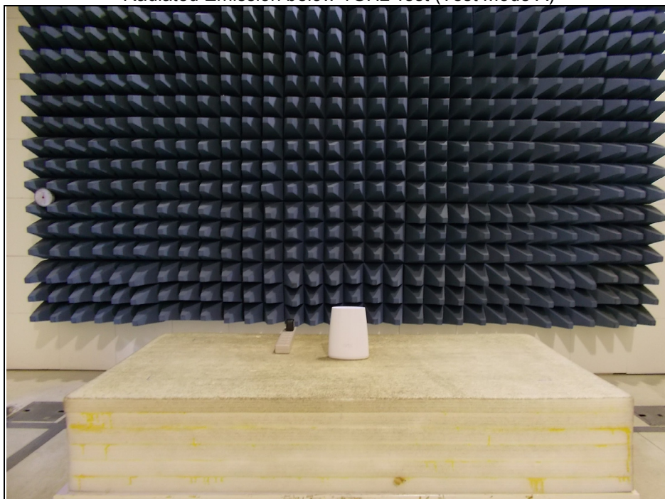
Radiated Emission below 1GHz Test (Test Mode A)
