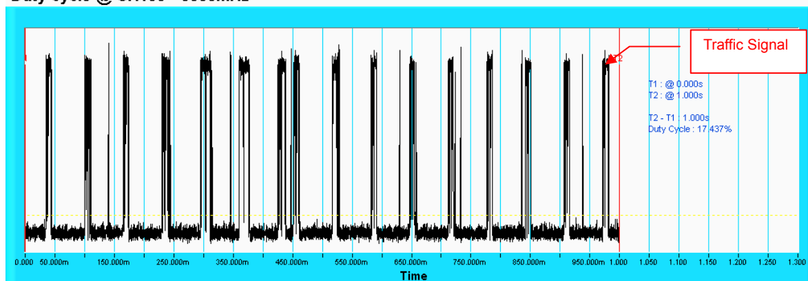
Duty cycle @ CH100 - 5500MHz
