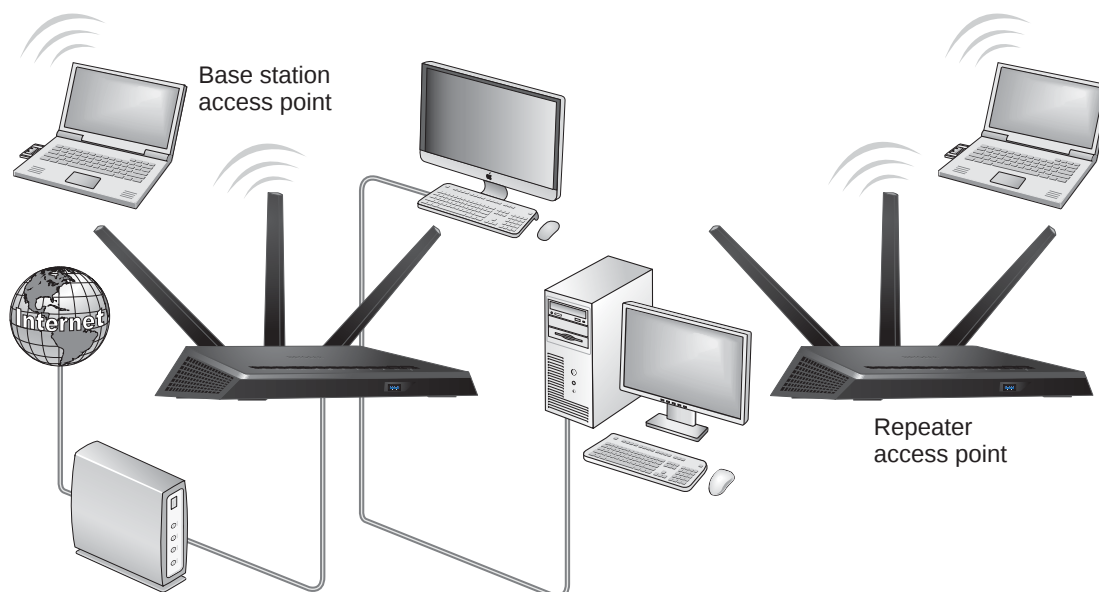
Figure 13. Wireless repeating scenario
