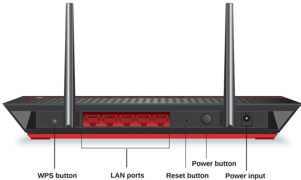
Figure 1. Rear panel
