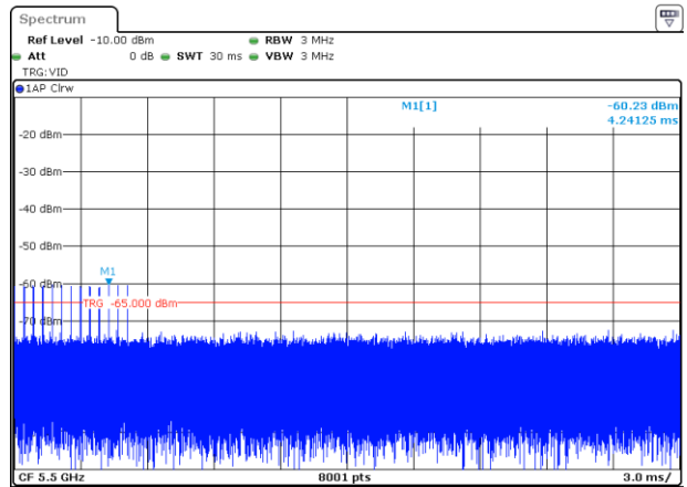
Radar #5DFS detection threshold level
