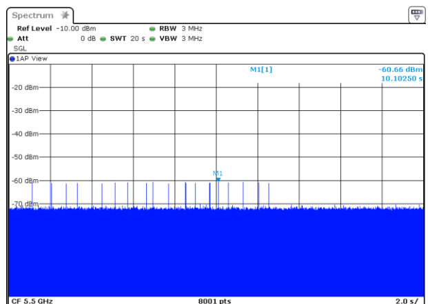
Radar #6DFS detection threshold level
