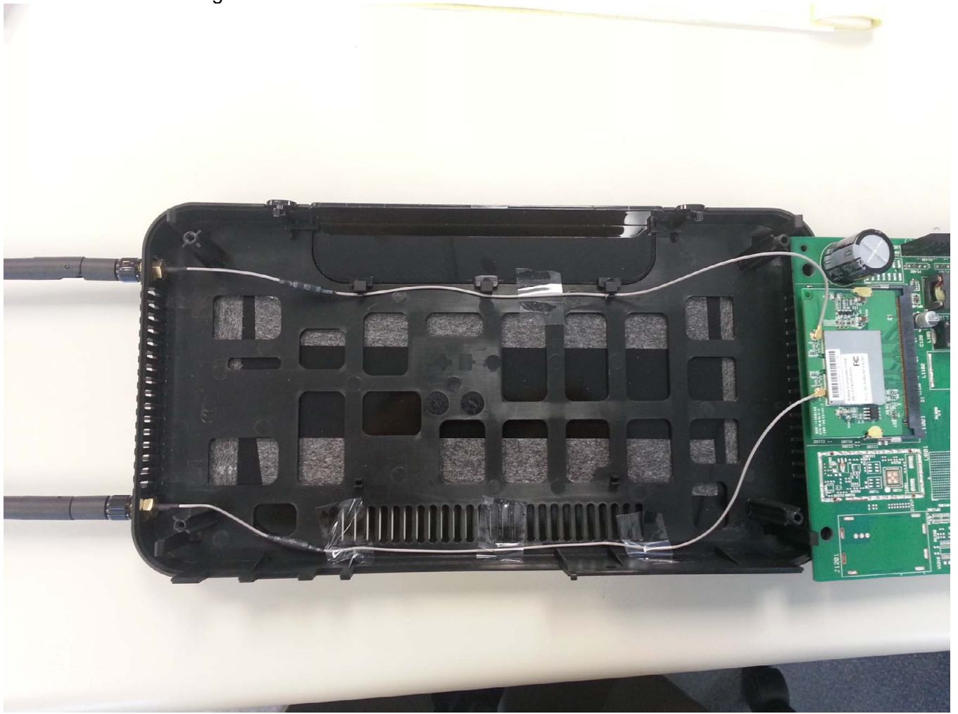
Main PC board showing connection to antennas
